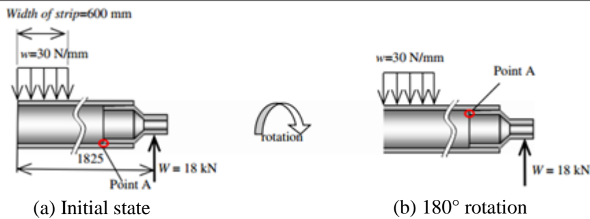
Figure 4 Dimensions and loading condition of new roller
