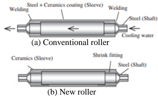
Figure 2 Roller structure
