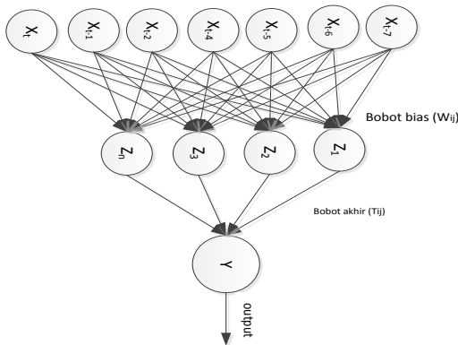
Figure 2. Network Architecture MLP Method Seismic Data of Mt. Merapi
