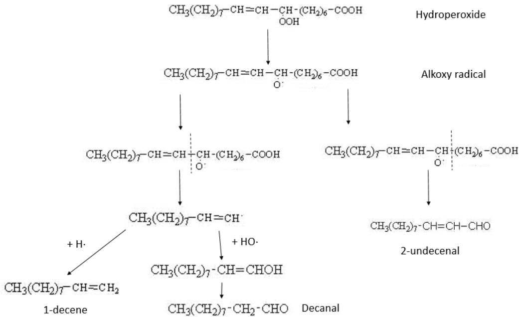
2 Figure 2-7. The possible pathways of secondary oxidation of oleic acid.
