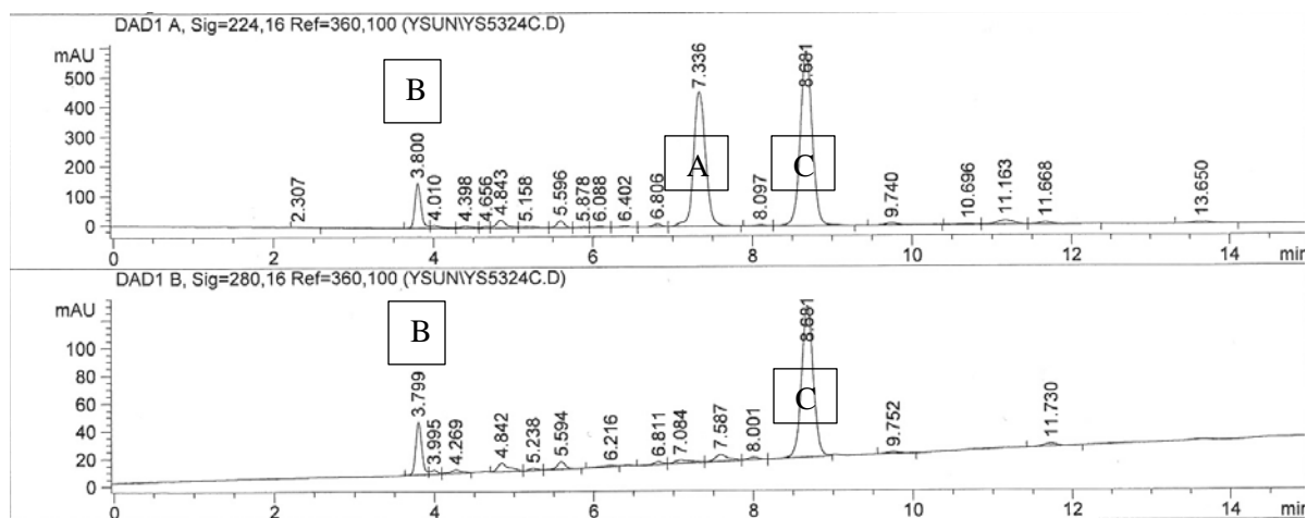
1 2 Figure 4-1. High-performance liquid chromatography (HPLC) chromatograms of starting 3 materials (a, b) and resultants (c) of synthesis of tyrosol DHA ester at 280 nm. A: DHA; B: 4 tyrosol; and C: tyrosol DHA ester.
