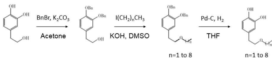
8 9 Figure 2-2. Synthesis of hydroxytyrosol alkyl ethers by a three-step method.
