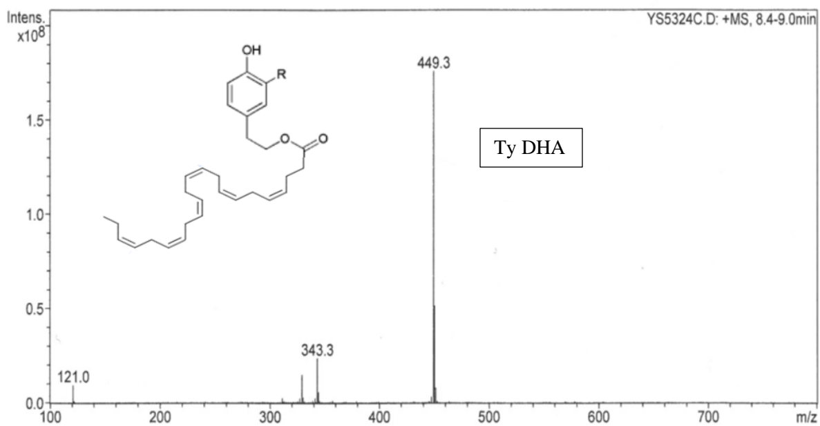
5 6 Figure 4-2. Chemical structures and mass spectrometric data of tyrosol DHA ester.
