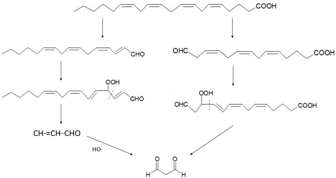
5 Figure 2-8. The possible generation pathways of malondialdehyde (MDA).
