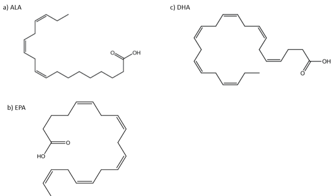
1 2 Figure 2-5. Chemical structure of \alpha -linolenic acid (ALA), eicosapentaenoic acid (EPA) and 3 docosahexaenoic acid (DHA).
