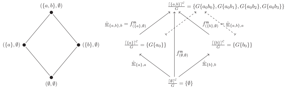
Fig. 13. The Hasse diagram of the poset P[\emptyset, \{a, b\}, \emptyset] in the context of Example 1.7 and, on the right-hand side, the associated diagram of sets.
