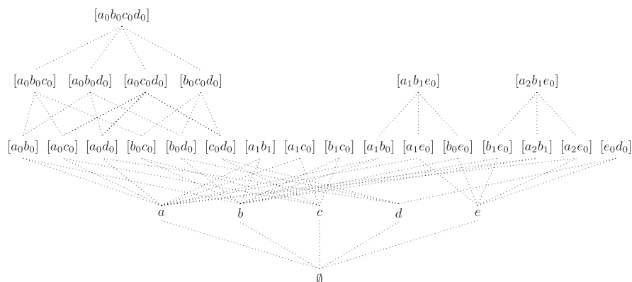
Fig. 6. The set system \mathcal{C}_S , with dotted lines representing the Hasse diagram of the associated poset. We use shorthand notation, where we write, e.g., [a_0 b_0 c_0] for the orbit \mathbb{Z}^2\{a_0, b_0, c_0\} .
