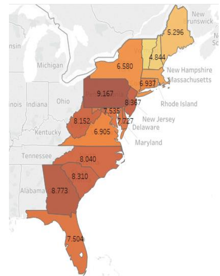
Figure 4. Daily mean PM 2.5 concentration in US east coast in 2016
