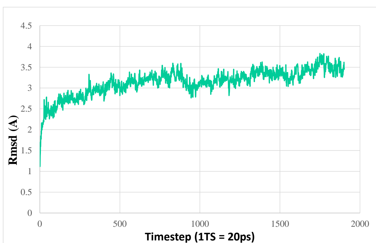
Figure 1: RMSD plot
