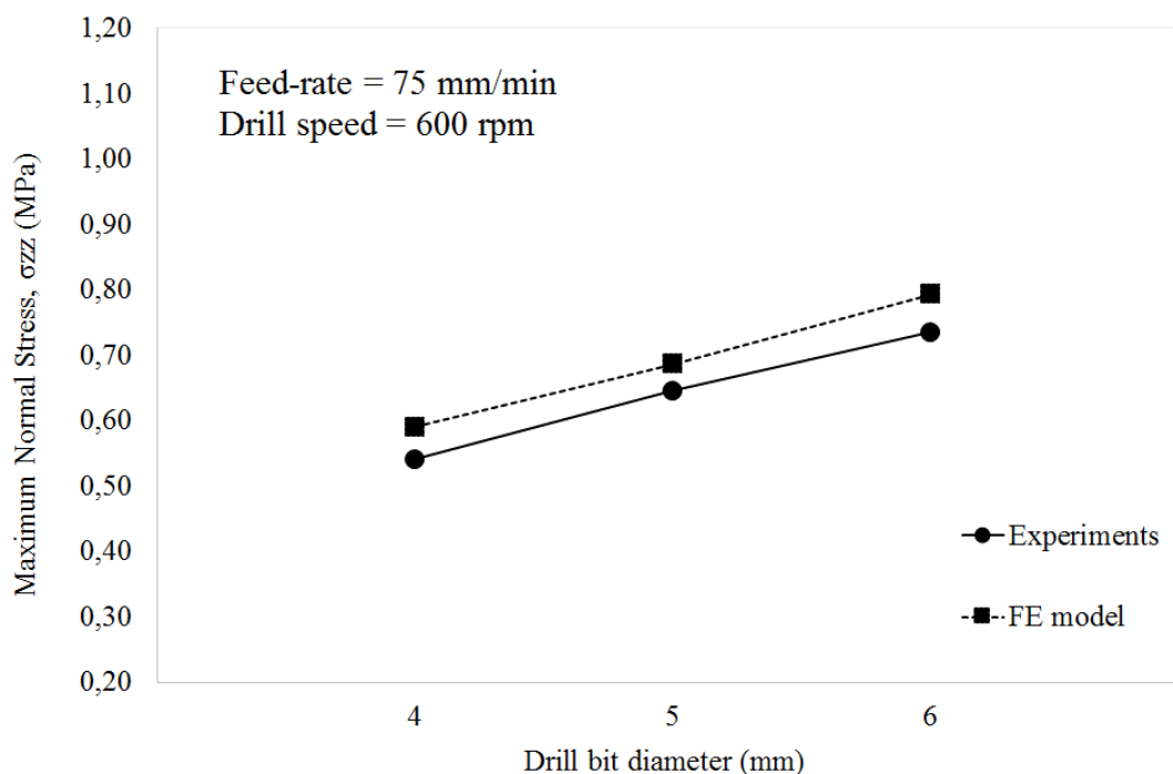
Figure 5: Results comparison for obtained stress at 4 mm of drilling depth, function of drill bit
