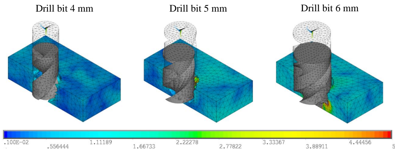
Figure 4: Results for obtained von-Mises stresses [MPa] at time=3,25s, function of drill bit
