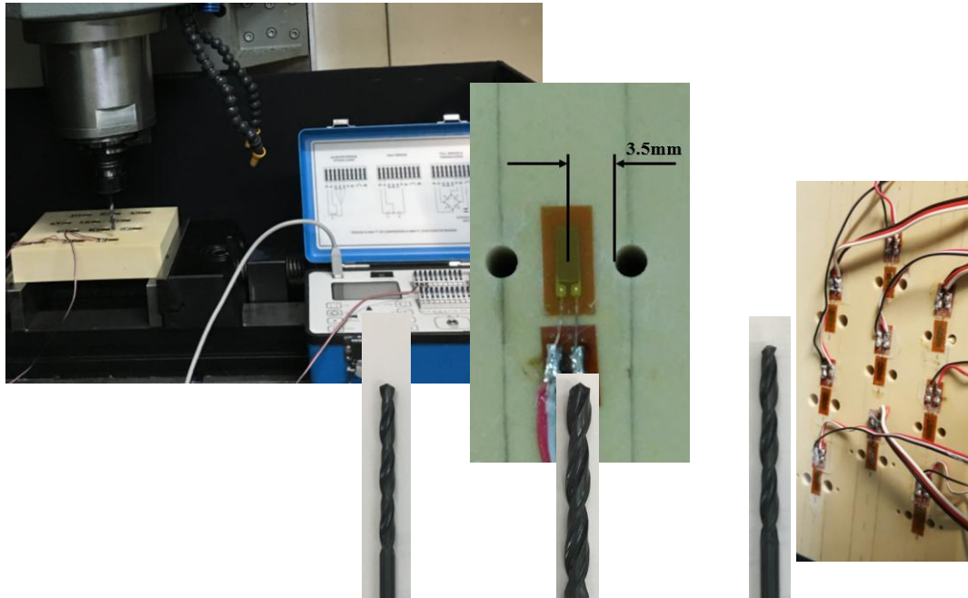
Figure 1: Experimental setup used for strain acquisition
