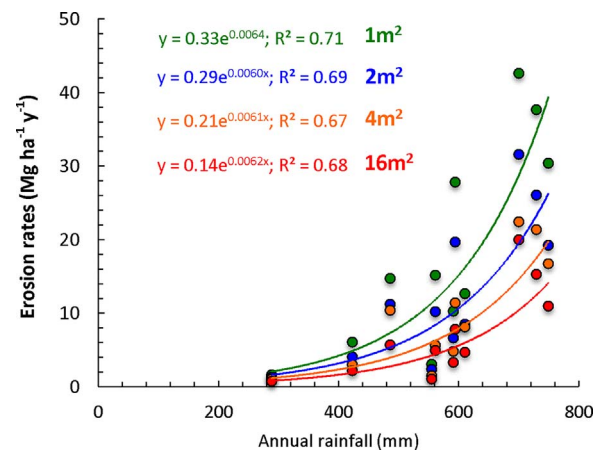
Fig. 6. Relationship between erosion rates and annual rainfall in each plot size.
