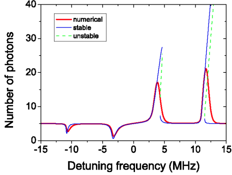
FIGURE 5. Average number of photons \bar{n} versus the detuning. The blue curves are obtained from the Langevin equations (17) and (19). They show the bistability with the solid curve denoting stable solutions, while the dashed curve denotes the unstable one. The red curve is obtained from the master equation (15). The driving amplitude is taken as \Omega_{R0}/2\pi = 5\text{MHz} . The parameters are for the qubit: \Delta/2\pi = 1\text{GHz} , \varepsilon = 0.01\Delta , \Gamma_0/2\pi = 125\text{kHz} , the resonator: \omega_r/2\pi = 6\text{MHz} , \kappa/2\pi = 1.7\text{kHz} , N_{th} = 5 , and the coupling: g/2\pi = 3.3\text{MHz} .
