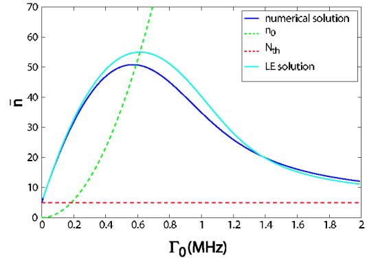
FIGURE 7. Average number of photons in the resonator as function of the qubit's relaxation rate, \Gamma_0 at the one-photon resonance, \Omega_R = \omega_r for g_3 = 0 and N_{th} = 5 . The dark blue line shows the numerical solution of the master equation, the light blue solid line represents the solution of the Langevin equation, Eq. (17). The green and red dashed curves represent respectively the saturation number n_0 and the thermal photon number N_{th} . The parameters are as in Fig. 5 (except for \Gamma_0 ).
