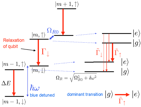
FIGURE 3. Dressed states of a driven qubit near resonance. Here m is the number of photons of the driving field, which is assumed to be quantized.
