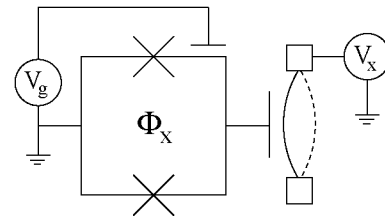
FIGURE 2. A charge qubit is coupled to a nano-mechanical resonator.
