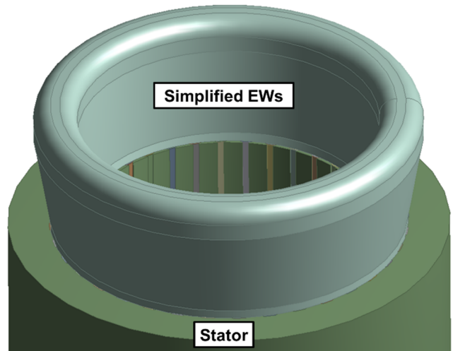
Figure 1: Simplified end winding geometry
