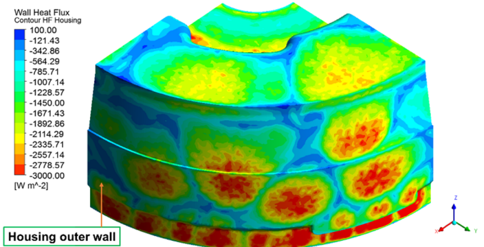
Figure 11: Housing wall's heat flux, new EWs model
