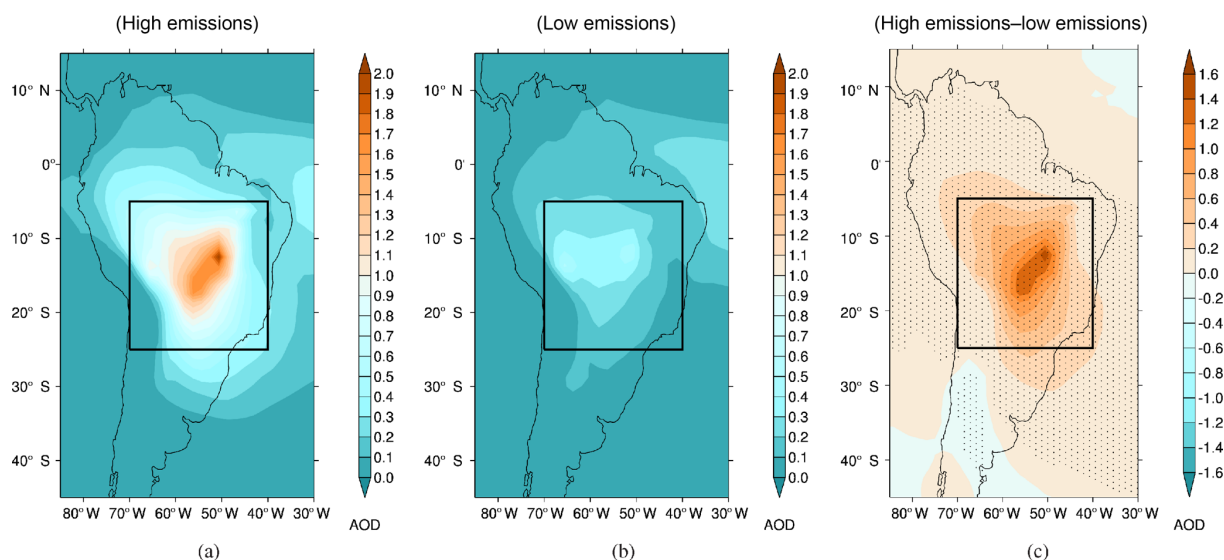
Figure 5. (a) The September mean biomass burning AOD at 0.44 \mu\text{m} for the high emissions experiment. The outlined box contains the area used to calculate mean values in Table 1. (b) The September mean biomass burning AOD at 0.44 \mu\text{m} for the low emissions experiment. (c) Plot of the difference in the September AOD between the high and low emissions experiment. Stippling represents 95 % confidence limit.
