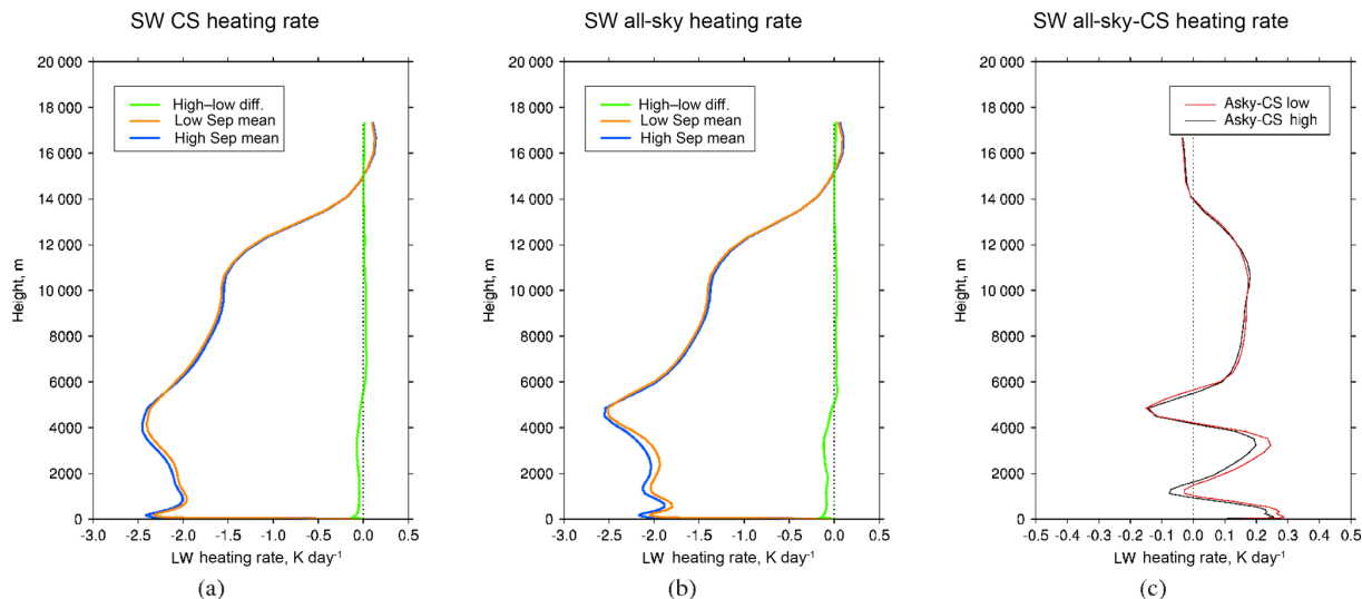
Figure 13. September mean LW heating rates (averaged over the BB box 5\text{--}25^\circ\text{S} , 40\text{--}70^\circ\text{W} ) for high and low emissions for (a) clear sky, (b) all sky and (c) all-sky–clear-sky differences.
