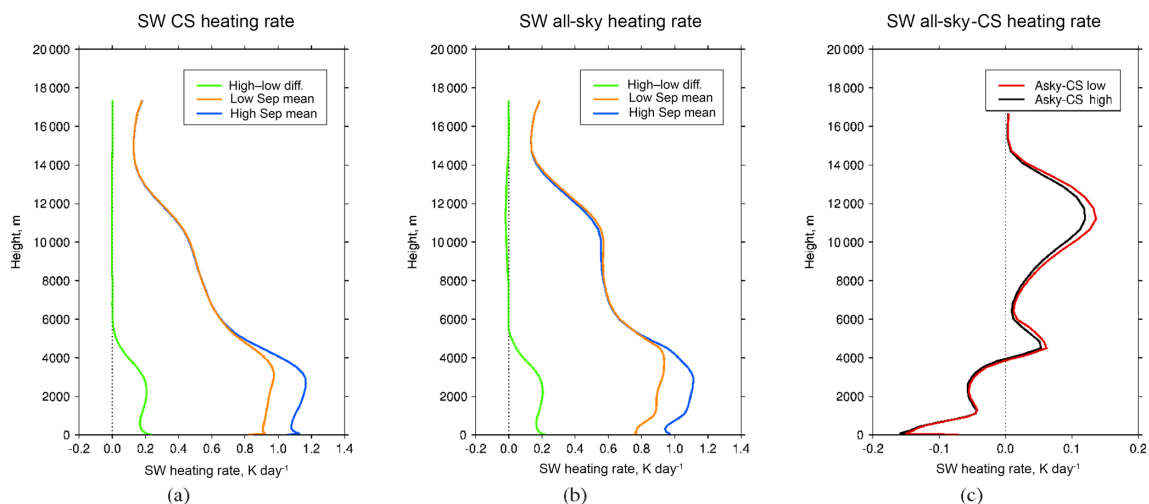
Figure 12. September mean SW heating rates (averaged over the BB box 5\text{--}25^\circ\text{S} , 40\text{--}70^\circ\text{W} ) for high and low emissions: (a) clear sky, (b) all-sky and (c) all-sky–clear-sky differences, showing heating rate changes due to cloud only.
