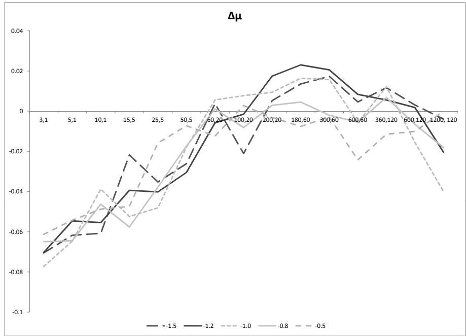
Fig. 3. Stopping premium, ( \Delta\mu ), from short-term (3,1) stop-loss strategies to longer-term (1200,120) stop-loss strategies with exit thresholds, ( \gamma ), of 1.5, 1.2, 1, 0.8, and 0.5 standard deviations from the mean with a 0 standard deviation re-entry threshold, ( \delta )
