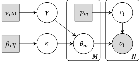
Fig. 3: The HBNI model, with per-class noise parameters \theta_m and shared hyperparameters, \kappa, \gamma .
