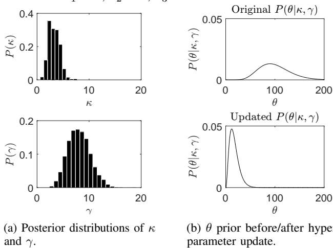
Fig. 5: Inference of high-level noise parameters \kappa , \gamma . Median hyperparameters were used for the plots on the right.
