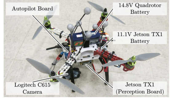
Fig. 7: Hardware overview.
