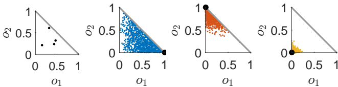
(a) 4 low-level classifier observations. (b) Classifications for c = 1 , \theta_{c=1} = 1 . (c) Classifications for c = 2 , \theta_{c=2} = 6 . (d) Classifications for c = 3 , \theta_{c=3} = 20 .
