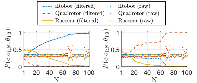
(a) SSBF posterior over time. (b) HBNI posterior over time.
