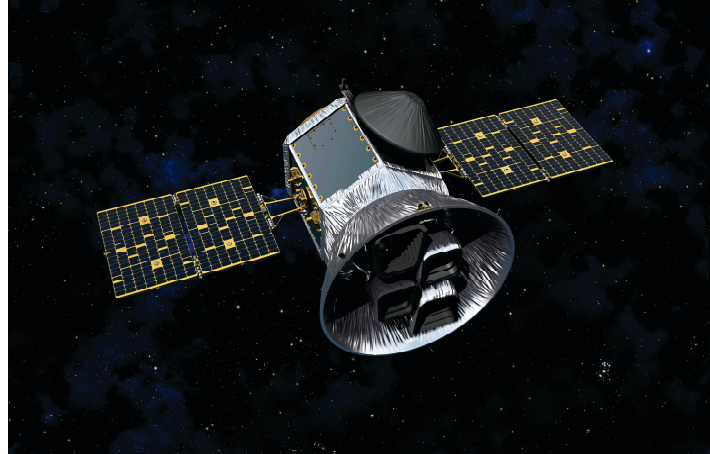
Figure 5. Left. —Diagram illustrating the orientations of the four TESS cameras, lens hoods, and mounting platform. Right. —Artist's conception of the TESS spacecraft and payload.
