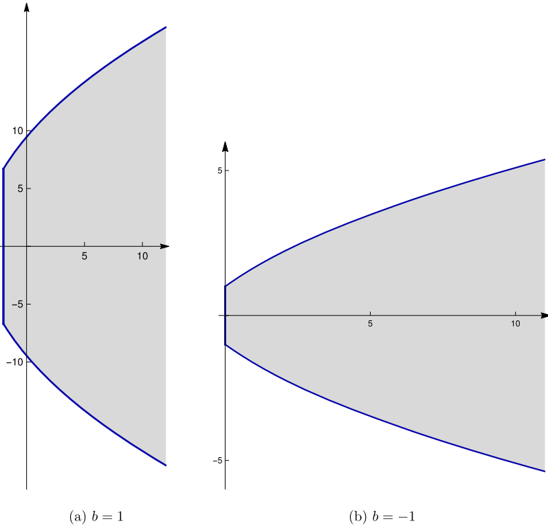
Fig. 3. The plots show the regions given in Theorem 7.4 (iv), (v), respectively, that contain W(A_{[B]}) for (a) b > 0 and (b) b < 0 ; it is assumed that \min \sigma(A_N) = 0 , C\|\overline{\text{Im } B}\| = 1 , \mu = -1 for both cases and \xi = -4 in (a).
