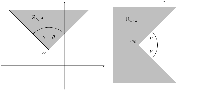
Fig. 2. The sectors S_{z_0, \theta} and U_{w_0, \nu} , defined in (6.1) and (6.2), respectively.
