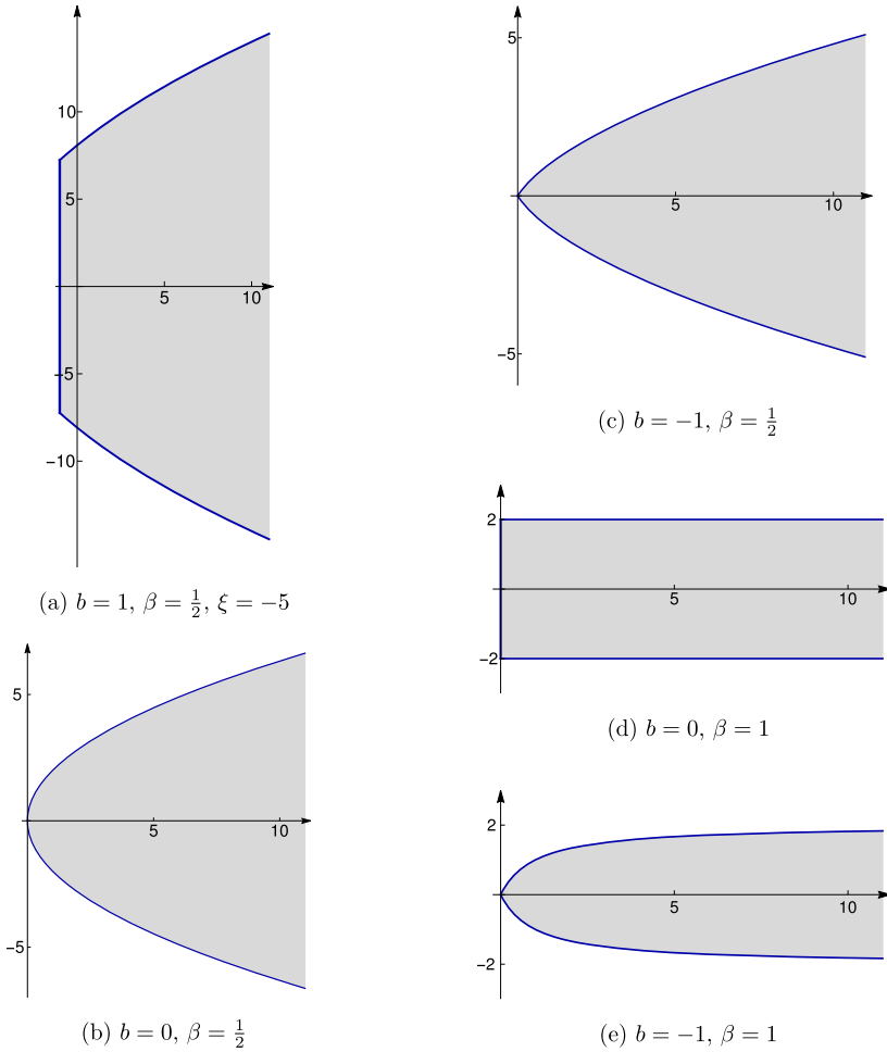
Fig. 1. The plots show the regions given by the right-hand sides of (5.12), (5.13), (5.15) with \mu = 0, C = 1 and \|\overline{\text{Im } B}\| = 1 for the following cases: \beta = \frac{1}{2} in (a)–(c) ( b > 0, b = 0, b < 0 , respectively) and \beta = 1 in (d), (e) ( b = 0, b < 0 , respectively).
