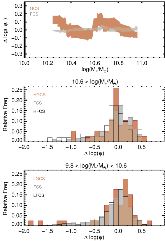
Figure 5. Top: median value of \Delta\log(\psi_*) as a function of M_* for the GCS sample in a sliding tophat bin containing 25 galaxies (red shaded area). The width of the shaded region denotes the bootstrapped uncertainty in the median value. The median value of \Delta\log(\psi_*) for the FCS sample in bins covering the range in stellar mass corresponding to that of the sliding tophat applied to the GCS sample is shown as a grey shaded region, with the width again indicating the uncertainty in the median. Middle: distribution of \Delta\log(\psi_*) for the HGCS sample (filled red histogram), the HFCS sample (open black histogram), and the FCS sample in the mass range \log(M_*/M_\odot) \geq 10.6 . All three distributions are similar to the degree that the null hypothesis that they are all drawn from the same parent population cannot be discarded. Bottom: as middle panel but for the stellar mass range 9.8 \leq \log(M_*/M_\odot) < 10.6 , i.e. the LGCS and LFCS samples.
