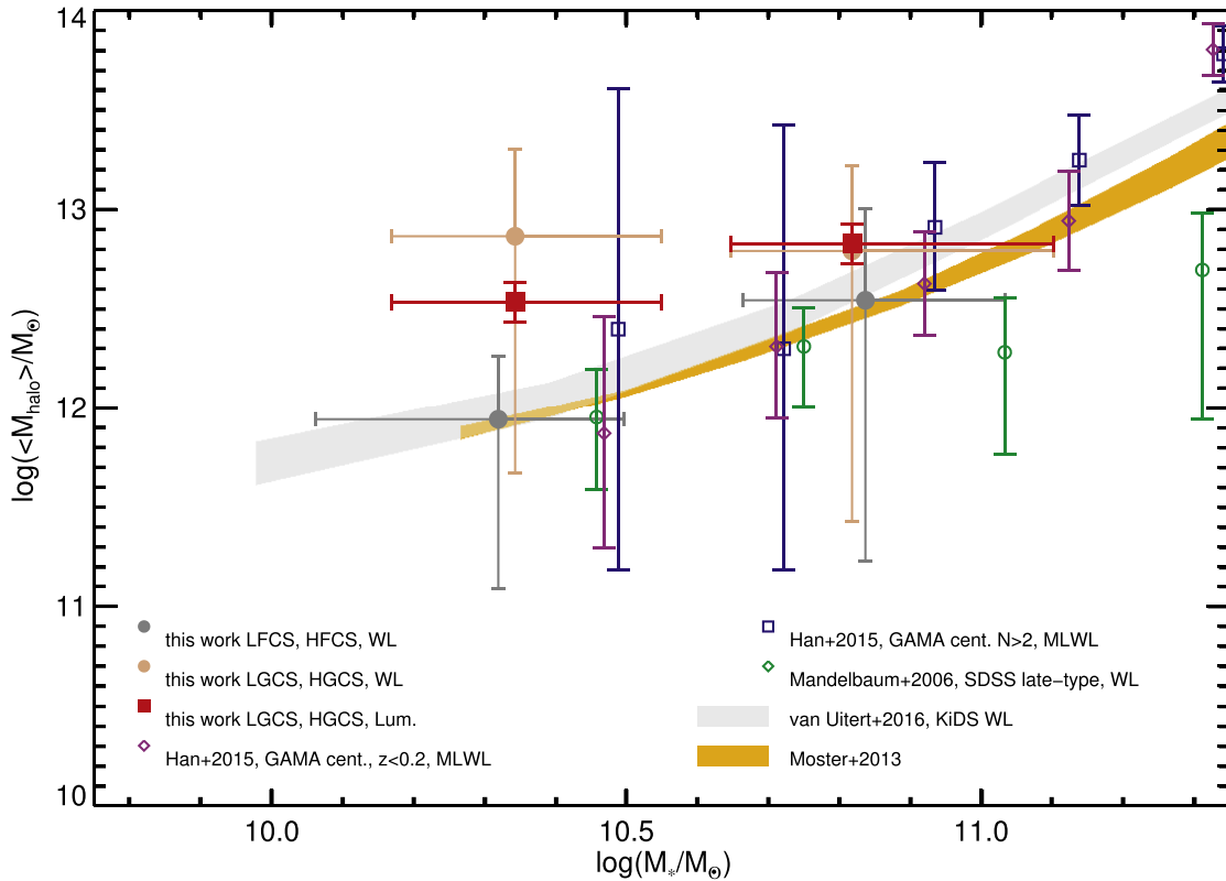
Figure 6. Average host DMH mass of the LFCS and HFCS samples (grey filled circles) as determined from stacked weak-lensing measurements using the KiDS galaxy–galaxy weak-lensing pipeline as detailed in Appendix B. The symbols denote the mode of the posterior PDFs, while the error bars show the 68 per cent HPD interval containing the mode. In stellar mass, the symbols denote the median with the error bars indicating the 16th–84th percentile range in stellar mass contributing to the stack. For the LGCS and HGCS samples, the independent group luminosity-based median DMH mass estimates are shown as filled red squares with the error bars indicating the uncertainty in the median. For comparison, the empirical median M_{\text{halo}}-M_{*} relation derived by van Uitert et al. (2016) using the full KiDS–GAMA overlap, as well as the abundance matching based M_{*}-M_{\text{halo}} relation of Moster et al. (2013) – converted to the form M_{\text{halo}}-M_{*} (Han et al. 2015) – are shown as grey (dash-dotted) and yellow (dashed) outlined regions, with the width indicating the range between the 16th and 84th percentile. For further comparison, the results of two recent independent comparable weak-lensing analysis are overlaid. The median DMH halo masses found by Han et al. (2015) using a SDSS imaging-based maximum-likelihood weak-lensing analysis in bins of central galaxy stellar mass for a volume-limited (at z = 0.2 ) sample of GAMA central galaxies and a flux-limited sample of GAMA group central galaxies ( N \geq 3 , i.e. with some similarity to our GCS sample), are shown as open purple diamonds and open blue squares, respectively. Similarly, the median DMH masses of a flux-limited sample of central late-type SDSS galaxies presented by Mandelbaum et al. (2006) are shown as open green circles.
