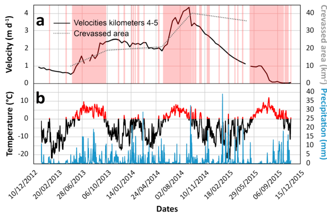
Figure 8. (a) Velocities of Aavatsmarkbreen glacier throughout its surge averaged between kilometers 4 and 5 (Figure 1 for kilometers). The gray dotted line represents the total crevasse area on the glacier measured using TerraSAR-X images. Melt seasons are shaded in red. (b) Daily air temperature (in red and black) and precipitation (blue) collected at Ny Ålesund (from eklima.no , Norwegian Met Office), for location see black triangle in Figure 1a.
