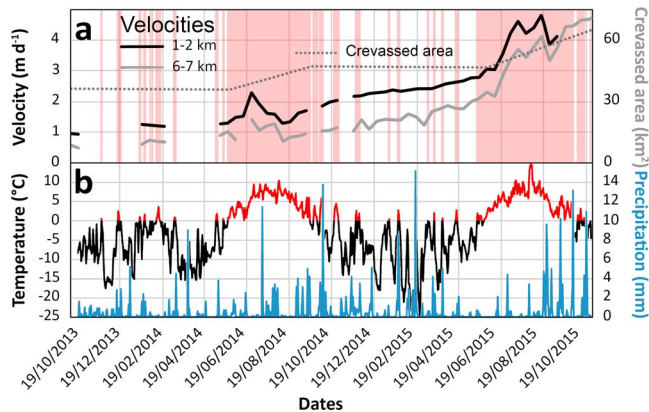
Figure 12. (a) Velocities of the glacier Wahlenbergbreen from feature tracking between pairs of TerraSAR-X images (Table S1). The gray dotted line represents the total crevassed area on the glacier measured using TerraSAR-X images. Melt seasons are shaded in red. (b) Daily air temperature (in red and black) and precipitation (blue) collected at Longyearbyen airport (from eklima.no , Norwegian Met Office). For location see black triangle in Figure 3.
