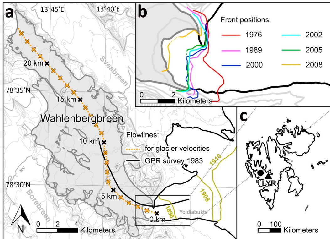
Figure 3. Location of Wahlenbergreen in Svalbard. Topographic map modified from http://toposvalbard.npolar.no (Norwegian Polar Institute), gray glacier outline is from 2007, downloaded from the Randolph Glacier Inventory 5.0 (Pfeffer et al., 2014). Glacier front positions from 1976 to 2008 mapped using Landsat images (Table S1), older front positions from Hagen et al. (1993), Plassen et al. (2004), and De De Geer (1910). The orange dotted line, marked every kilometer, represents the glacier centerline used to extract glacier velocities. The continuous black line marks the 1983 GPR survey line (Bamber, 1987).
