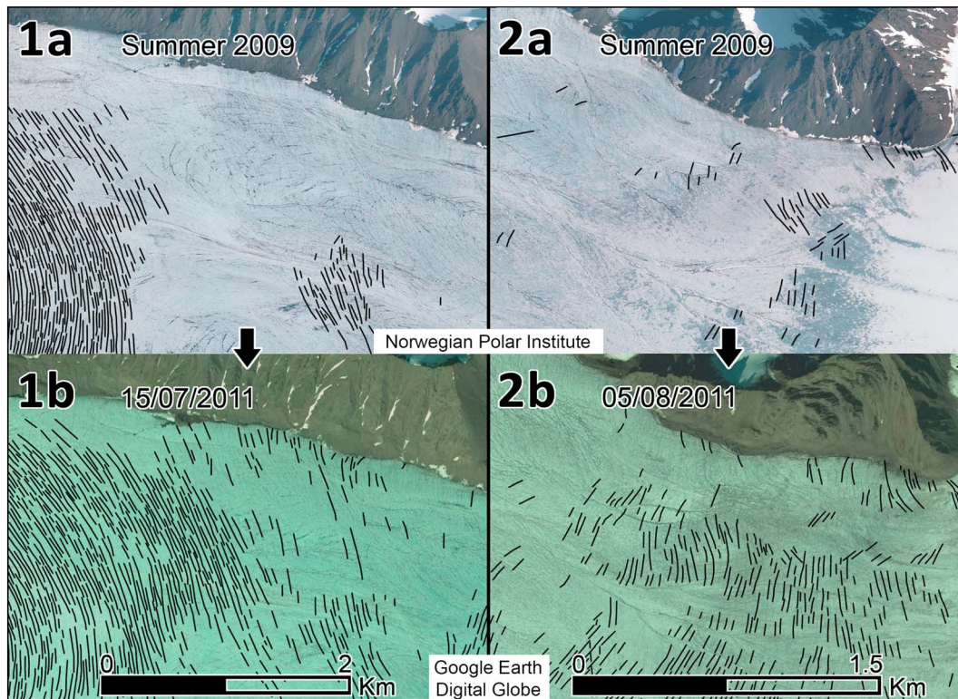
Figure 6. Comparison of surface crevassing between 2009 and 2011 for Aavatsmarkbreen. Images from 2009 are from the Norwegian Polar Institute (Topsvalbard.npolar.no), images from 2011 are from DigitalGlobe (Google Earth; Table S1). The contrast of the images was enhanced. See Figure 1 for the location of zones a and b.
