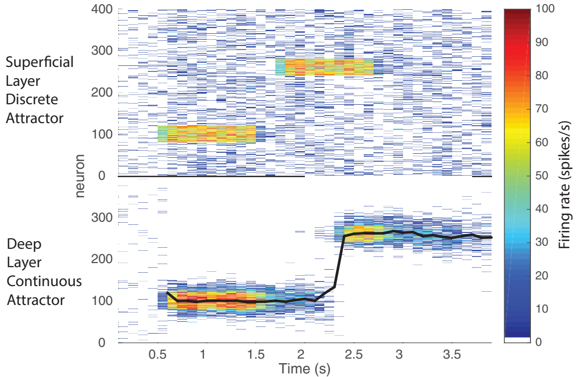
Figure 9: A jump transition in the deep continuous attractor network. Simulation of the operation of the superficial discrete attractor network (above) and the deep continuous attractor network (below). Time from 0 to 4 s is shown along the abscissa. Neurons 0–400 above are the 10 pools in the superficial module discrete attractor network. Neurons 0–400 below are the excitatory neurons in the deep module continuous attractor network. The colour indicates the firing rate of each neuron, with the calibration bar showing the rate in spikes/s measured over 100 ms epochs. At time 500–1500 ms pool 3 of the superficial discrete attractor network received an external input, and after a short period, it entered a high firing rate attractor state which died off after the stimulus to pool 3 was removed. Via the connections from the superficial to the deep module, neurons in the corresponding part of the continuous attractor network started firing. The width (standard deviation) of the Gaussian profile for the recurrent connectivity synaptic strength was 60 neurons. After a delay of 200 ms, discrete superficial pool 7 was activated by an external input, from time=1700–2700 ms. The discrete attractor pool 7 entered a high firing rate attractor state, which died off some time after the stimulus to pool 7 was removed. The figure shows that the deep continuous attractor packet or bubble of activity jumped without a continuous transition from its position when it was being activated by the input from superficial pool 3 to the position when it was being activated by the input from superficial pool 7. The centre of gravity of the deep (continuous attractor) pool is shown by the black line.
