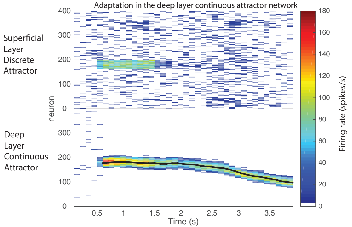
Figure 12: Effects of adaptation on a continuous attractor network. Simulation of the operation of the superficial discrete attractor network (above) and the deep continuous attractor network (below). Time from 0 to 4 s is shown along the abscissa. Neurons 0–400 above are the 10 pools in the superficial module discrete attractor network. Neurons 0–400 below are the excitatory neurons in the deep module continuous attractor network. The colour indicates the firing rate of each neuron, with the calibration bar showing the rate in spikes/s measured over 100 ms epochs. At time 500–1500 ms pool 5 of the superficial discrete attractor network received an external input, and after a short period, it entered a high firing rate attractor state which died off after the stimulus to pool 5 was removed. Via the connections from the superficial to the deep module, neurons in the continuous attractor network started firing. The width (standard deviation) of the Gaussian profile for the recurrent connectivity synaptic strength was 15 neurons. The figure shows that when it was no longer clamped by the firing in the superficial network, the deep continuous attractor packet or bubble of activity drifted continuously from its position when it was being activated by the input from superficial pool 5 across the space mapped by the continuous attractor network. The centre of gravity of the deep (continuous attractor) pool is shown by the black line.
