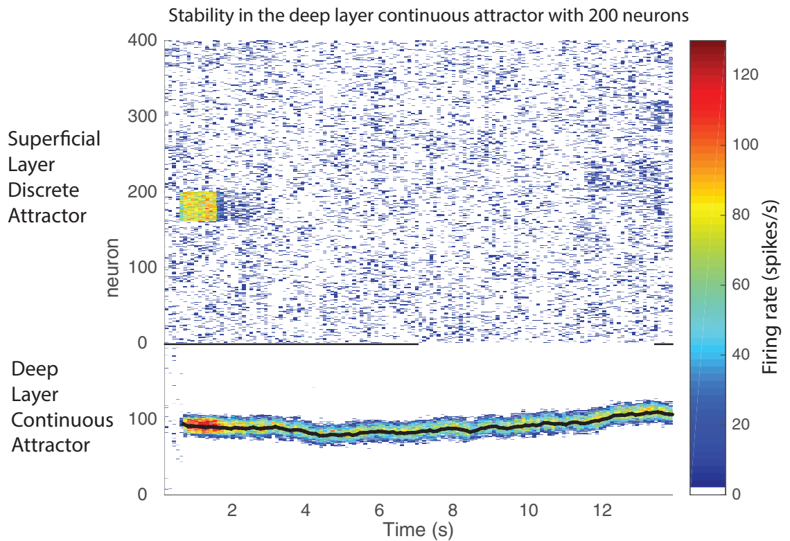
Figure 10: Stability of the continuous attractor network with stochastic integrate-and-fire neurons. Simulation of the operation of the superficial discrete attractor network (above) and the deep continuous attractor network (below) for a case where there is a relatively small number of excitatory neurons, 200, in the deep attractor network. Time from 0 to 14 s is shown along the abscissa. Neurons 0–400 above are the 10 pools in the superficial module discrete attractor network. Neurons 0–200 below are the excitatory neurons in the deep module continuous attractor network. The colour indicates the firing rate of each neuron, with the calibration bar showing the rate in spikes/s measured over 100 ms epochs. At time 500–1500 ms pool 5 of the superficial discrete attractor network received an external input, and after a short period, it entered a high firing rate attractor state which died off after the stimulus to pool 5 was removed. Via the connections from the superficial to the deep module, neurons in the continuous attractor network started firing. The width (standard deviation) of the Gaussian profile for the recurrent connectivity synaptic strength was 15 neurons. The centre of gravity of the deep (continuous attractor) pool is shown by the black line. The figure shows that there was some short-term noise in the continuous attractor network, and some long-term drift over the 12 s period in which it received no external input. (Target=0.35)
