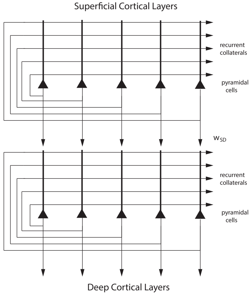
Figure 3: Schematic drawing of the cortical architecture simulated in Experiment 1 with a discrete attractor network in the superficial layers connecting to a discrete attractor network in the deep layers. One local patch or module or column of neocortex was modelled. Pyramidal cells are represented by filled triangles, their dendrites are indicated by thick lines above the cell body, and the axons are represented by thin lines. Synapses are present wherever an axon crosses a dendrite. The superficial layers (2 and 3) were modelled as a fully connected discrete attractor network, which connected via synapses of strength w_{SD} to the network in the deep layers also modelled as a fully connected discrete attractor network. The difference between the two networks was that there was adaptation of the neuronal firing in the deep layer network. Both networks were integrate-and-fire attractor networks with n possible attractor states. Five populations of neurons, each implementing one of the attractor states are signified by the five pyramidal cells drawn for each network. For the simulations described here there were n=10 orthogonal attractor states in the each network, each implemented by a population of neurons with strong excitatory connections between the neurons with value w_+ for the NMDA and AMPA synapses. There were N_s=1000 neurons in each network, of which 0.8 were excitatory (pyramidal cells), and 0.2 were inhibitory (not illustrated).
