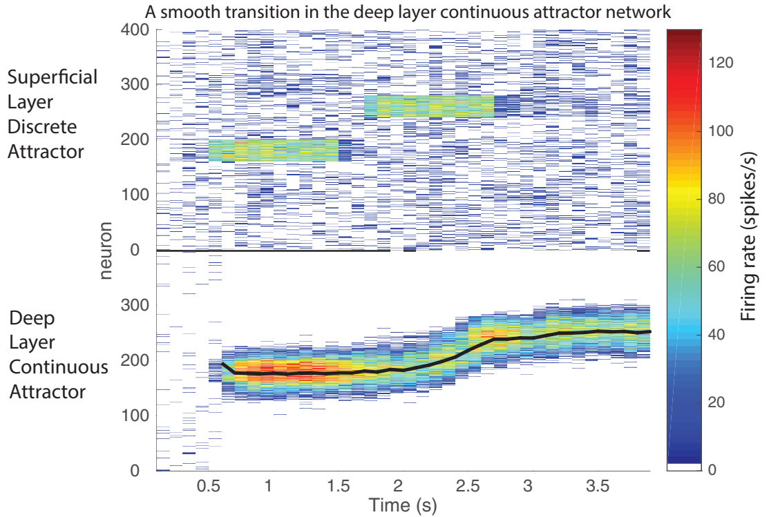
Figure 8: A smooth transition in the deep continuous attractor network. Simulation of the operation of the superficial discrete attractor network (above) and the deep continuous attractor network (below). Time from 0 to 4 s is shown along the abscissa. Neurons 0–400 above are the 10 pools in the superficial module discrete attractor network. Neurons 0–400 below are the excitatory neurons in the deep module continuous attractor network. The colour indicates the firing rate of each neuron, with the calibration bar showing the rate in spikes/s measured over 100 ms epochs. At time 500–1500 ms pool 5 of the superficial discrete attractor network received an external input, and after a short period, it entered a high firing rate attractor state which died off after the stimulus to pool 5 was removed. Via the connections from the superficial to the deep module, neurons in the corresponding part of the continuous attractor network started firing. The width (standard deviation) of the Gaussian profile for the recurrent connectivity synaptic strength was 60 neurons. After a delay of 200 ms, pool 7 was activated by an external input, from time=1700–2700 ms. The discrete attractor pool 7 entered a high firing rate attractor state, which died off some time after the stimulus to pool 7 was removed. The figure shows that the deep continuous attractor packet or bubble of activity moved somewhat continuously from its position when it was being activated by the input from superficial pool 5 to the position when it was being activated by the input from superficial pool 7. The centre of gravity of the deep (continuous attractor) pool is shown by the black line. The figure shows that no such continuous transition occurred in the superficial, discrete attractor, network. The spontaneous firing rate of the neurons in the deep layer not in the packet of activity was inhibited in this and the following figures by inhibition received through the inhibitory neurons from the excitatory neurons firing fast in the continuous attractor.
