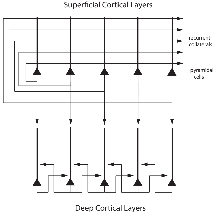
Figure 7: Schematic drawing of the cortical architecture simulated in Experiment 2. One local patch or module or column of neocortex was modelled. Pyramidal cells are represented by filled triangles, their dendrites are indicated by thick lines above the cell body, and the axons are represented by thin lines. Synapses are present in the superficial layers wherever an axon crosses a dendrite; and in the deep layers by where the arrows at the end of each axon point to a dendrite. The superficial layers (2 and 3) were modelled as a fully connected discrete attractor network. This is an integrate-and-fire attractor network with n possible attractor states. Five populations of neurons, each implementing one of the attractor states are signified by the five pyramidal cells drawn. For the simulations described here there were n=10 orthogonal attractor states in the superficial layer of the module, each implemented by a population of neurons with strong excitatory connections between the neurons with value w_+=2.1 for the NMDA and AMPA synapses. There were always N_s=500 neurons in the superficial layer of the module, of which 0.8 were excitatory (pyramidal cells), and 0.2 were inhibitory (not illustrated). The deep layers (layer 5) were modelled as an integrate-and-fire continuous attractor network. The main difference was that the (excitatory) recurrent collaterals connected more strongly to their neighbours than to more distant neurons, as shown schematically. The number of neurons in the deep, continuous attractor, network was typically N=500 neurons, but in some investigations was set to N=125 , 250, 1000 or 1500 neurons. Each of the n=10 local regions of the deep layers received inputs from one of the n discrete attractor populations of neurons in the superficial layers, in a way that could be set up by self-organizing topographic map formation.
