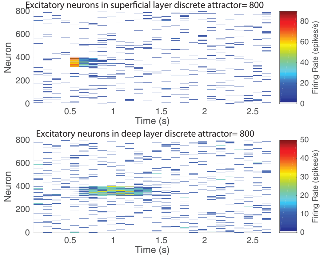
Figure 5: Effects of adaptation on the time course of the deep layer discrete attractor in Experiment 1. Simulation of the operation of the superficial discrete attractor network (above) and the deep discrete attractor network (below), both of which contained 800 excitatory neurons. Time from 0 to 2.7 s is shown along the abscissa. Neurons 0–800 above are the excitatory neurons in the 10 pools in the superficial module discrete attractor network. Neurons 0–800 below are the excitatory neurons in the 10 pools in the deep module discrete attractor network. The colour indicates the firing rate of each neuron, with the calibration bar showing the rate in spikes/s measured over 100 ms epochs. After 500 ms of spontaneous activity, at time 500–600 ms pool 5 of the superficial discrete attractor network received an external input, and after a short period, it entered a high firing rate attractor state which died off after the stimulus to pool 5 was removed. Via the connections from the superficial to the deep module, neurons in the corresponding pool 5 of the deep discrete attractor network started firing, showing that the deep network was operating as an attractor. However, with the neuronal adaptation, the firing in the deep network continued for only approximately 800 ms. Without the neuronal adaptation the firing in the deep network continued indefinitely. For parameters, see text. Additional parameters: w+ for deep attractor=2.2; AHPCaD = 1.0; inh0n = 1.00; inhS = 1.05; inhD = 1.07.
