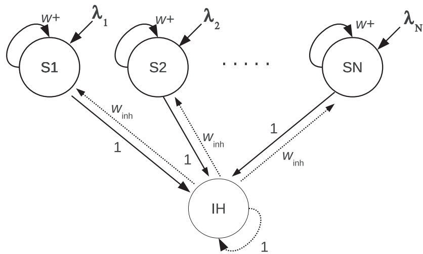
Figure 4: The architecture of a superficial or deep module containing one fully connected discrete attractor network. The excitatory neurons are divided into N=10 selective pools or neuronal populations S1–SN of which three are shown, S1, S2 and SN. The synaptic connections have strengths that are consistent with associative learning. In particular, there are strong intra-pool connection strengths w_+ . The excitatory neurons receive inputs from the inhibitory neurons with synaptic connection strength w_{inh}=1 . The other connection strengths are 1. The integrate-and-fire spiking module contained 500 neurons, with 40 in each of the 10 non-overlapping excitatory pools, and 100 in the inhibitory pool IH. Each neuron in the network also receives external Poisson inputs \lambda_{ext} from 800 external neurons at a typical rate of 3 Hz/synapse to simulate the effect of inputs coming from other brain areas.
