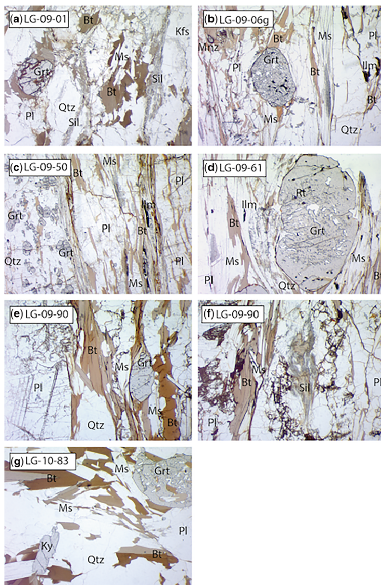
Fig. 2. Thin section photomicrographs. Mineral abbreviations after Whitney & Evans (2010) : Bt, biotite; Grt, garnet; Kfsp, potassium feldspar; Ky, kyanite; Mus, muscovite; Pl, plagioclase; Qtz, quartz; Sill, sillimanite; Field of view 5.5 mm. Further images are available in the Supplementary material.
