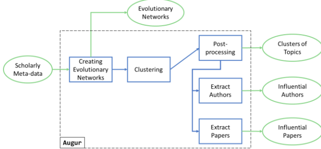
Figure 1: Workflow of Augur. The rectangles represent the stages. The circles represent the input/output data.
