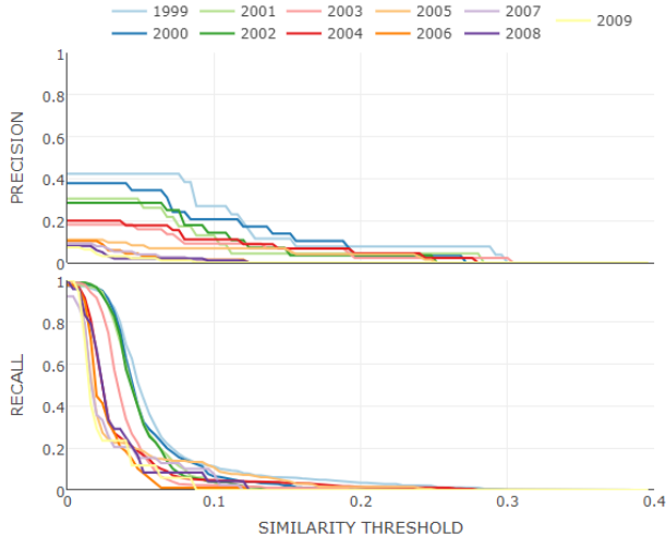
Figure 4: Performance of Fast Greedy algorithm.
