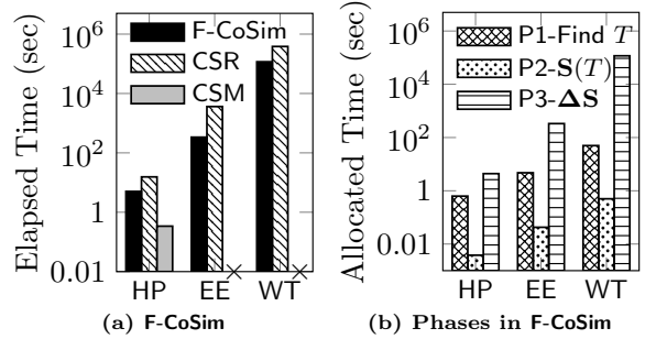
Figure 4: Time Efficiency on Static Graphs
