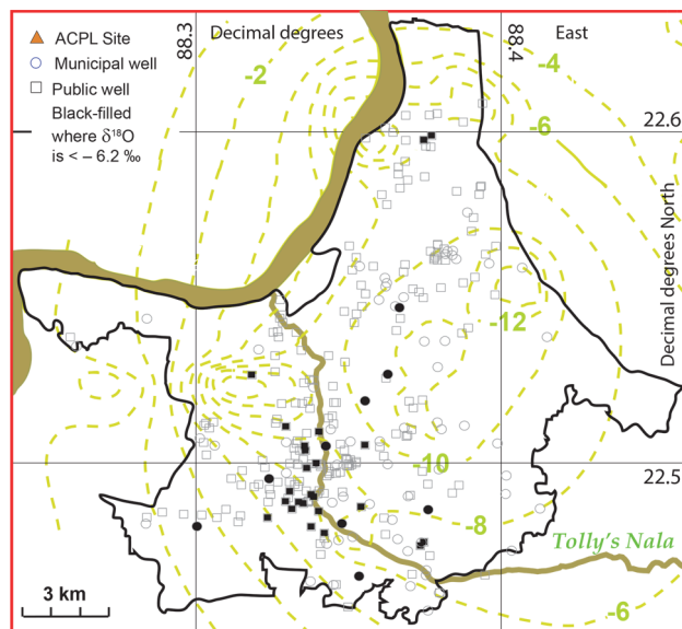
Figure 9. Map of the distribution of groundwaters with values of \delta^{18}\text{O} less than -6.2 ‰, volume-weighted annual mean for \delta^{18}\text{O} in local rainfall. The isotopically light groundwater is located close to Tolly's Nala and cluster around the ACPL site and a site on Tolly's Nala about 1 km south of the ACPL site. This distribution proves the existence of a direct route for recharge between Tolly's Nala and the underlying late Pleistocene aquifer.
