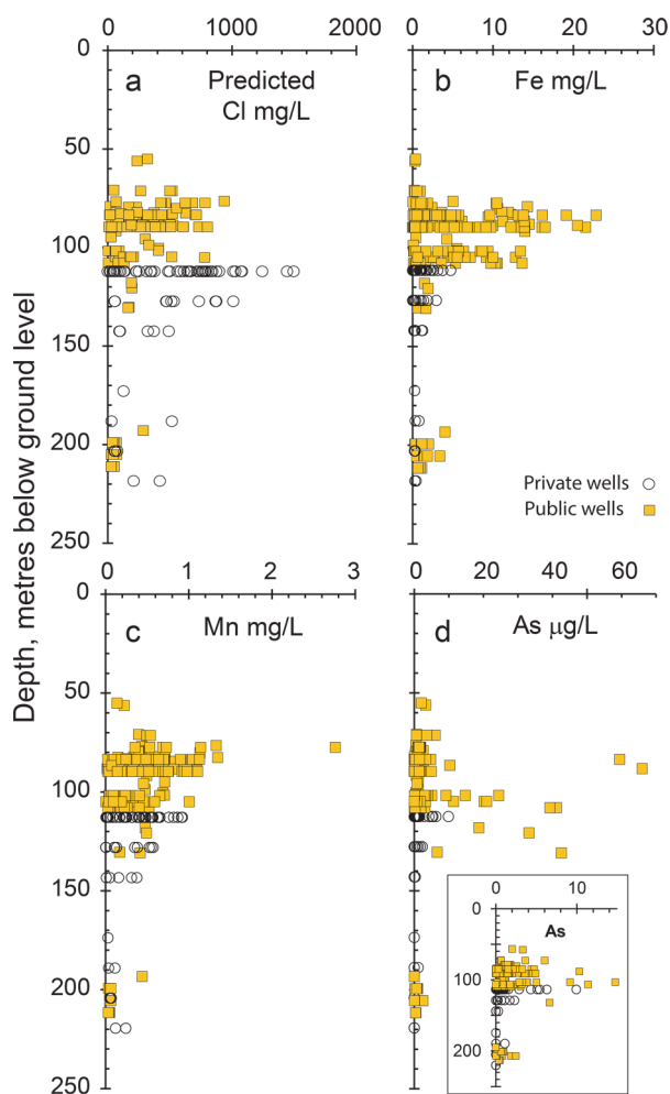
Figure 11. Depth profiles of Predicted-Cl (a), Fe (b), Mn (c), and As (d), in groundwater beneath the Kolkata Municipal Corporation. Depths given to midscreen. Predicted-Cl is Cl predicted from Br concentrations, a measure that emphasizes the influence of marine-derived waters by removing anthropogenic Cl. Values are not plotted for the 24 groundwaters with Cl/Br below the marine-mixing line in Figure 12a.
