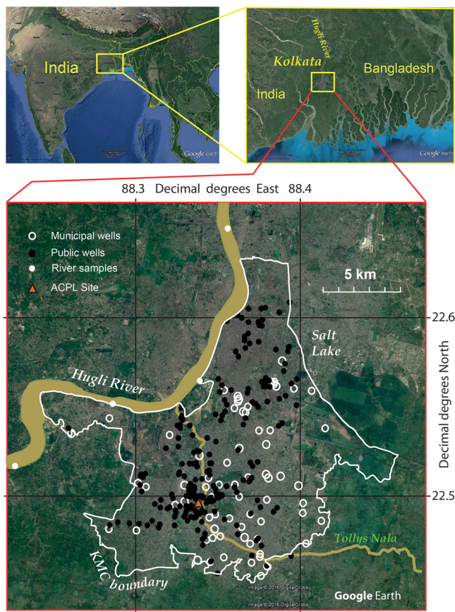
Figure 1. Map showing the boundary of the Kolkata Municipal Corporation (KMC) and the locations of sampled wells, 4 of 5 river-sampling sites (the fifth is 13 km north of the map limit) and the location of the ACPL factory (red filled triangle at 88.339° E, 22.496° N) that manufactured Paris green, an arsenical pesticide, between 1965 and 1985. GPS of all locations are in Table S1 to WGS84, as used in Google Earth.
