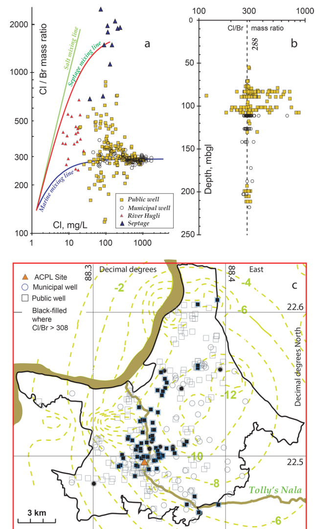
Figure 12. (a) Cross plot of Cl and Cl/Br in groundwater beneath the KMC and for septage in West Bengal. 59 Groundwaters contaminated by sewage and septage plot above the marine-mixing line; (b) depth, to midscreen, of Cl/Br; values >308 are not present beneath 110 m depth—we use 308 rather than the marine value of 288 to allow for analytical uncertainty; and (c) distribution across KMC of Cl/Br values of groundwater, showing that most Cl/Br values >308 occur close to Tolly's Nala.
