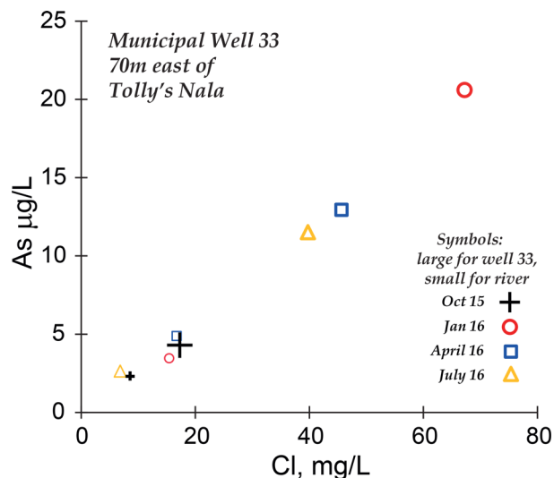
Figure 10. Seasonal changes in As and Cl in groundwater from Well 33, sited 70 m east of Tolly's Nala. Water from this well comprises varying proportions of groundwater and river water from Tolly's Nala. Linear mixing is shown by most constituents (Table S1). The mixing line shows that Well 33 is partly recharged by river-bank infiltration from Tolly's Nala. For river data, we use the river sample RC of Table S1, which was the nearest river sample to the confluence of the River Hugli and Tolly's Nala, some 2.0 km upstream of the confluence.
