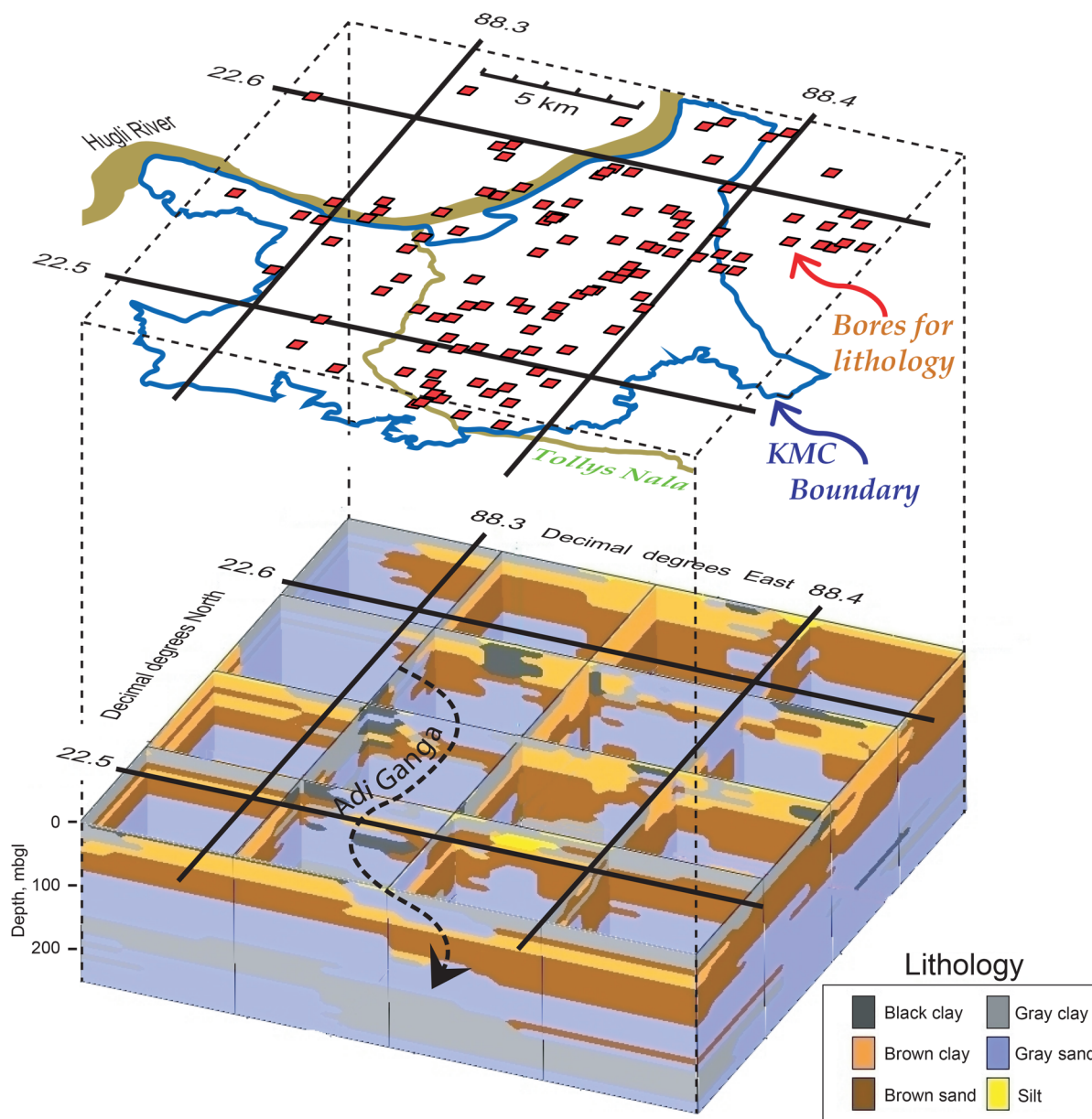
Figure 5. Geology beneath KMC and borehole locations ( n = 109 ) used to map the distribution of facies. Borehole data from ref 38. The deep palaeo-channel of the Adi Ganga, a previous course of the Hugli River, is shown as a dotted line in the lower part.
