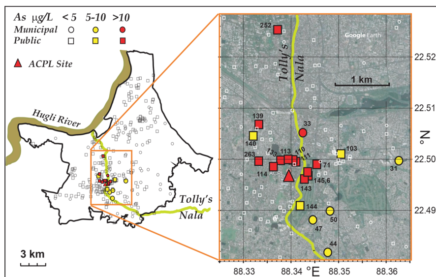
Figure 6. Distribution of As in groundwater beneath the KMC. Sample locations in Table S1. Groundwaters with >5 \mu\text{g/L} As are close to Tolly's Nala and/or the ACPL factory site, where Paris green, an arsenical pesticide, was manufactured between 1965 and 1985.
