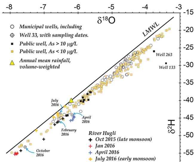
Figure 8. Isotopic compositions of groundwaters compared to the local meteoric water line, LMWL, for the region, 44 which is essentially the same as the global MWL. Groundwaters plot along a mixing line between isotopically less-depleted late Pleistocene groundwaters with \delta^{18}\text{O} of around -3 to -4 ‰, and river waters ranging from -6.1 to -7.9 ‰.
