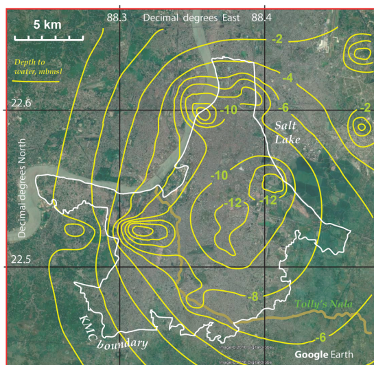
Figure 3. Modeled depth to the water table, relative to mean sea level, of groundwater beneath Kolkata outlining cones of depression caused by abstraction of groundwater for public supply. Model of ref 79; Table 2 of that reference gives measured water levels used to calibrate the model.
