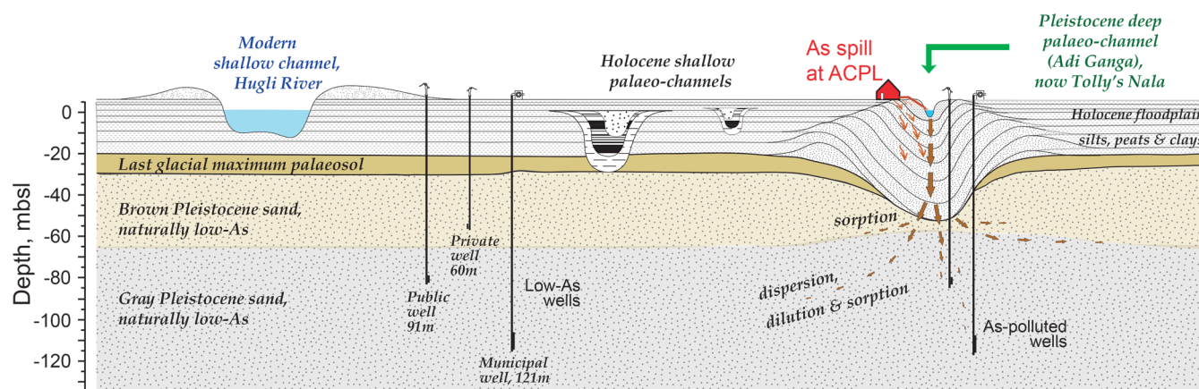
Figure 7. Schematic E–W cross-section through southern KMC, showing the disposition of major sedimentary units: floodplain deposits over a palaeosol over a late Pleistocene aquifer of brown sand over gray sand. Channels from Holocene river incision are filled largely by clays. One preglacial (deep) palaeo-channel marks the old course of the Adi Ganga river and is infilled with mostly sand, thereby forming a conduit for recharge to the late Pleistocene aquifer. The site of historical As-pollution at the ACPL factory is next to Tolly's Nala, which may be vestigial remnant of the Adi Ganga.
