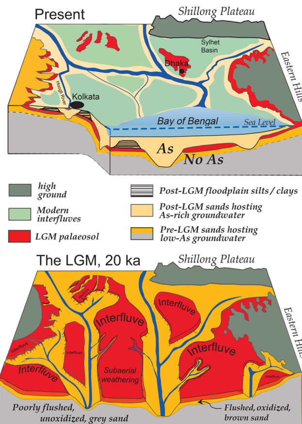
Figure 4. Schematic cross-section E–W through the Bengal Basin, showing, not to scale, the approximate distribution of pre- and post-LGM sediments. Pollution of groundwater by As is confined almost exclusively to post-LGM sediments. Updated from ref 29.
