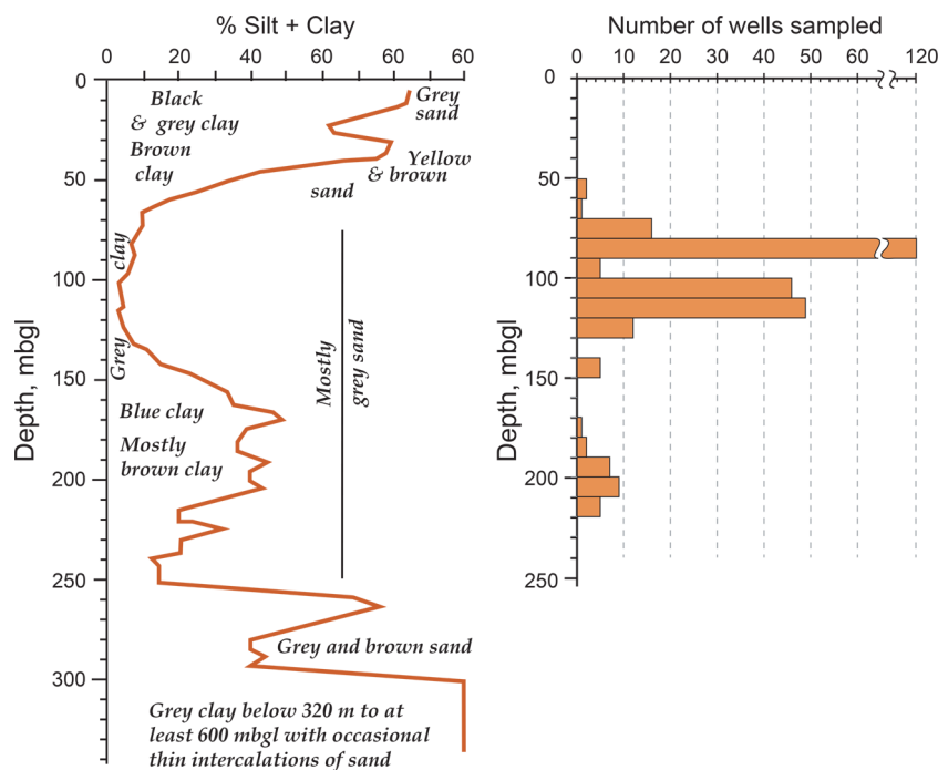
Figure 2. Composite lithological section compiled from 109 borehole logs used for Figure 5 (data from ref 38) together with a histogram of the number of wells sampled for this study compiled into 10 m bins using depths to midscreen.
