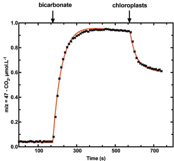
Fig. 6. Time course (black crosses) of ^{13}\text{C}^{18}\text{O}^{16}\text{O} ( m/z=47 ) and curve fitting (red line) using COPASI software as described in the Materials and methods. Low ^{18}\text{O} -enriched \text{Ci} (2.5 \text{mM} ) was injected at t=170 s, and chloroplasts at t=577 s after chemical equilibrium had been reached.
