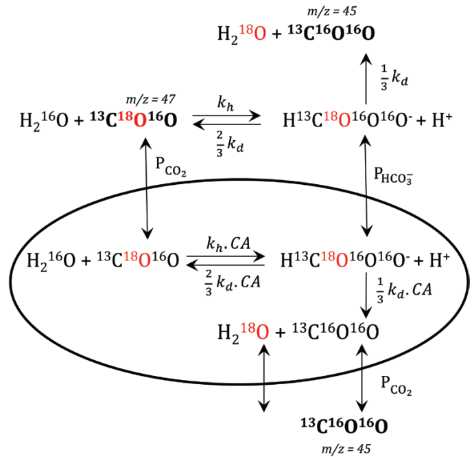
Fig. 1. A diagram of the assumed exchange of inorganic carbon isotopes with water used in the mathematical simulations and modelling described herein. P_{\text{HCO}_3^-} , \text{HCO}_3^- permeability of chloroplast; P_{\text{CO}_2} , \text{CO}_2 permeability of chloroplast; k_h , \text{CO}_2 hydration rate constant; k_d , \text{HCO}_3^- dehydration rate constant; CA, scaling factor of carbonic anhydrase activity. As the loss of ^{18}\text{O} from Ci species is the key component of measurements, ^{18}\text{O} is labelled in red. Ci species measurable in the mass spectrometer are in bold, and mass over charge value ( m/z ) specified. ^{13}\text{C} -labelled inorganic carbon is used for all assays.
