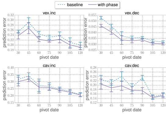
Figure 7: Mean normalized MSE for the baseline and phase-informed prediction over different pivot dates ( x -axis) for videos with less than 5 phases, broken down by the shape of the last phase of \mathbf{x}_{1:t_p} , \Delta t=15 days.
