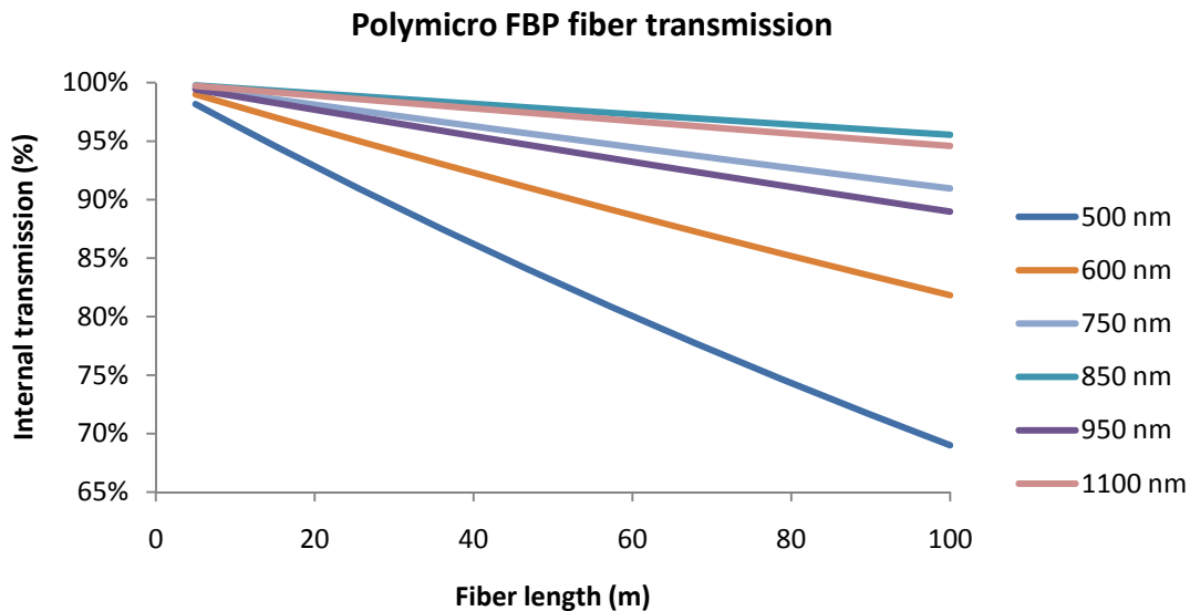
Figure 9: Fiber throughput as a function of fiber length at six different wavelengths for Polymicro FBP broadband fibers. This assumes optimal f -number, which is f/3 to f/4 . Note that at shorter wavelengths the fibers have a lower throughput, which gets progressively worse for \lambda < 500 nm. Data provided by Polymicro.
