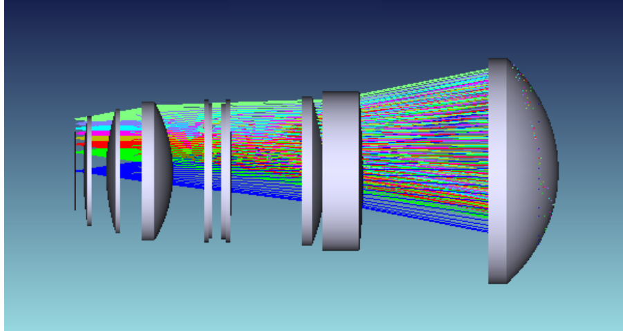
Figure 1: One option (DESPEC-SK-3C) for the DESpec optics. From right to left they are C1 to C3, the two-component ADC, C4, C5', and the field-flattener C6. The focal plane of fiber-ends would be just to the left of the new C6. "C1" is a little less than 1 meter in diameter. The optical train is 1.9 meters long. C1, C2, C3, and C4 are already installed on the telescope as part of DECam.
