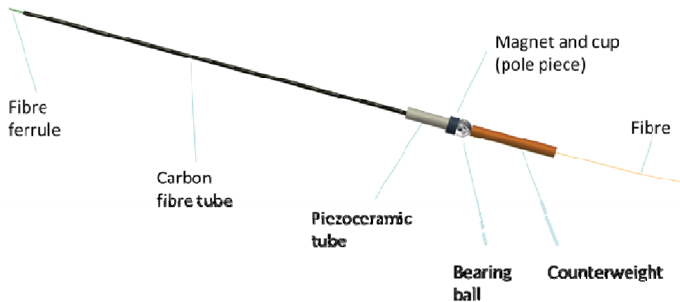
Figure 6: The MOHAWK unit fiber positioner. The spines pivot from mounts at the base and are driven by piezo-electric actuators.
