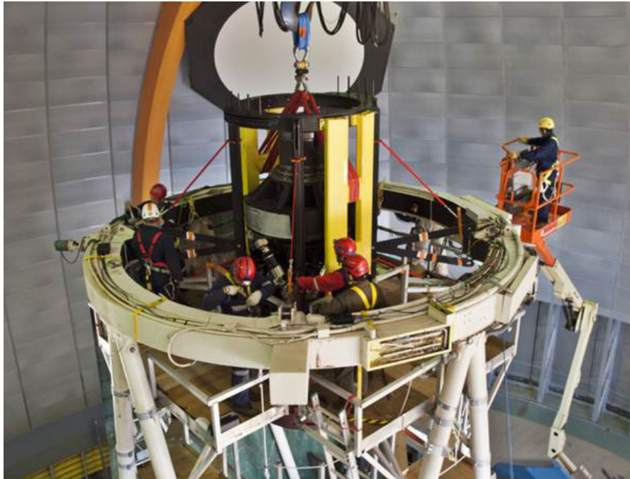
Figure 12: The new top end of the Blanco 4m telescope, during installation of the new prime focus cage to hold DECam.
