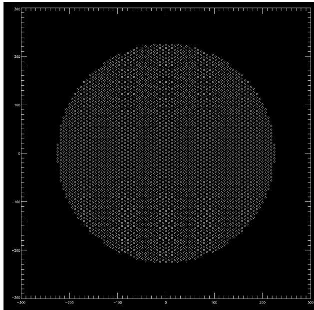
Figure 3: Array of DESpec fiber positioners. Here we show 3781 locations with 7 mm spacing (pitch) within the clear aperture. If the pitch were 6.3 mm, the clear aperture could accommodate 4675 fiber positioners. The x and y axes have units of mm. We have used a clear aperture of D=451 mm.
