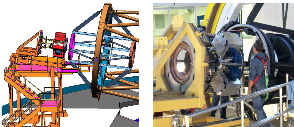
Figure 11: The DECam camera installation fixture (schematic at left, in close-up at right) at Fermilab. Right image shows the installation fixture being used to mount the camera in the Prime Focus Cage (black, at right).
