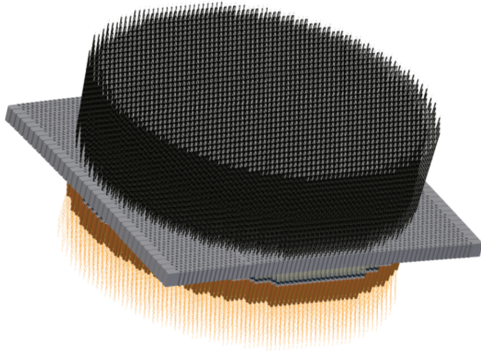
Figure 5: The MOHAWK fiber positioner with DESpec specifications, i.e., 4000 fibers with a 7mm pitch, placed in a 450mm diameter focal plane.
