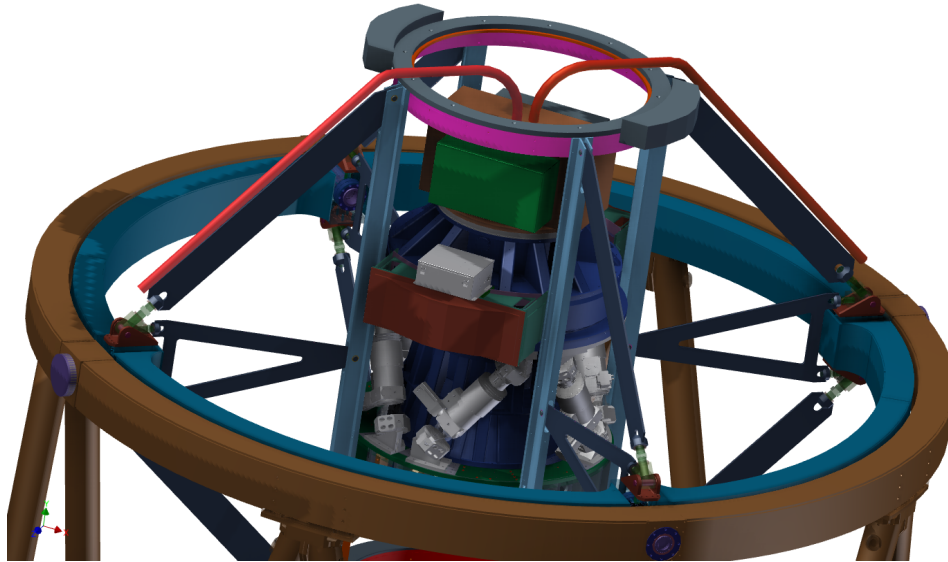
Figure 7: A schematic drawing of a MOHAWK-style fiber positioner positioned on top of the DESpec corrector optics, including the fiber bundles that would feed potential DESpec spectrographs.
