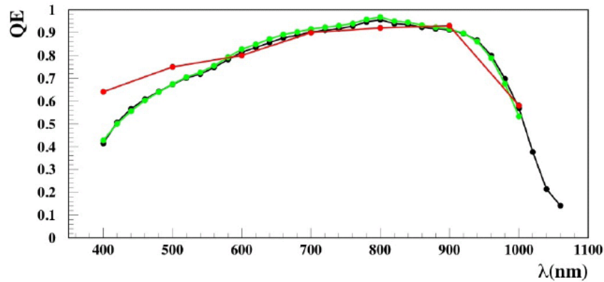
Figure 10: The absolute QE of three typical CCDs produced for the Dark Energy Camera. The blue side of the two-arm spectrographs could also use DECam 2kx4k CCDs.
