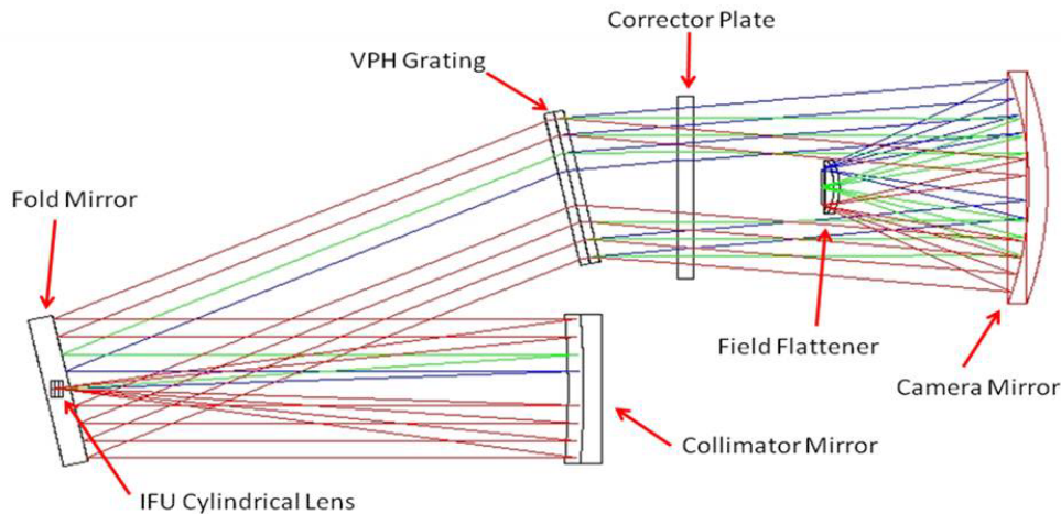
Figure 8: Optical layout of one of the VIRUS unit spectrographs. Light enters through a fiber slit on the left and is reflected by the collimator mirror and fold mirror before it passes through the grating. The vacuum Schmidt camera houses the CCD detector, which is located in the middle of the optical beam, just to the left of the field flattener lens. The overall length of the VIRUS is ~0.75m.
