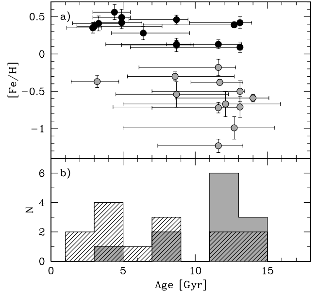
Fig. 7. Top panel show ages versus [Fe/H] for the now in total 26 microlensed dwarf and subgiant stars in the Bulge. Stars with [Fe/H] > 0 are marked with black circles and stars with [Fe/H] < 0 with grey circles. Bottom panel shows age histograms for the metal-rich stars (hatched histogram) and metal-poor stars (grey histogram).
