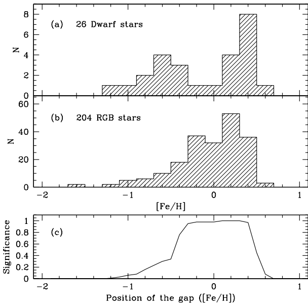
Fig. 6. a) MDF for our 26 microlensed dwarf stars in the bulge. b) MDF for 204 RGB stars in the bulge, from Zoccali et al. (2008). c) The significance for the failure to reproduce a gap vs. position of a gap in the dwarf star MDF (see explanation in Sect. 4.1).
