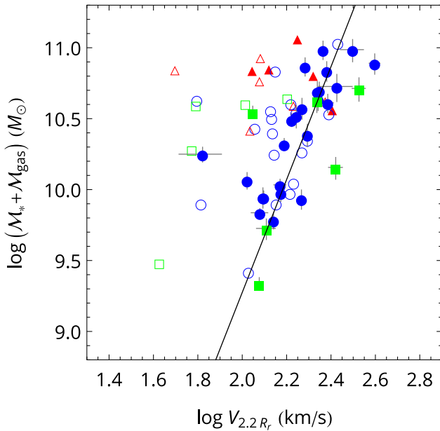
Figure 9. The baryonic TFR for the DYNAMO sample. Galaxies from the sample are plotted as in Fig. 8, but galaxies classified as rotating discs (RD and PR) have been highlighted. The error bars are omitted from the other points for clarity. The local baryonic TFR of McGaugh et al. (2000) is shown by the solid line and agrees well for the RD galaxies. Comparing with Fig. 8, it is apparent that the offset from the stellar mass TFR results from the high gas fractions inferred for many of the galaxies in our sample. The RD classified galaxy B 11-2 shows much lower circular velocity than expected; this galaxy is very round in appearance – the photometric inclination may not accurately reflect the kinematic inclination.
