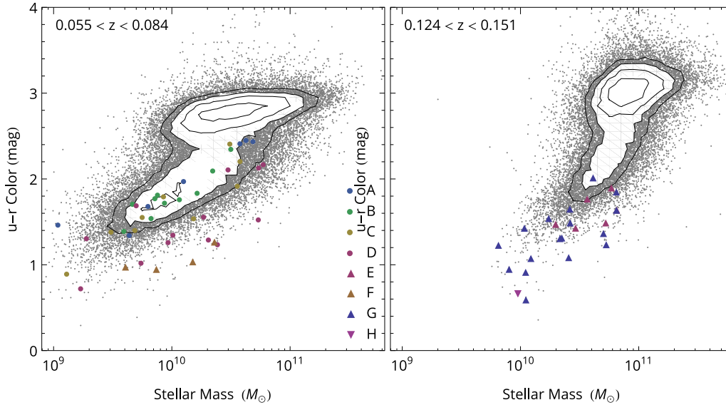
Figure 2. The u - r colours and masses for the SDSS spectroscopic sample are shown by the grey points and contours for the two redshift ranges of our selection criteria. Galaxies making up the DYNAMO selection within each redshift range are highlighted with coloured symbols. The symbol shape and colour correspond to the selection window as shown in the key, and match the symbol coding of Fig. 1. The impact of the limit of SDSS spectroscopy to apparent r -band magnitude less than 17.7 is reflected in the range of stellar masses included in each redshift range: \gtrsim 10^9 for the lower redshift range and \gtrsim 10^{10} for the higher redshift range.
