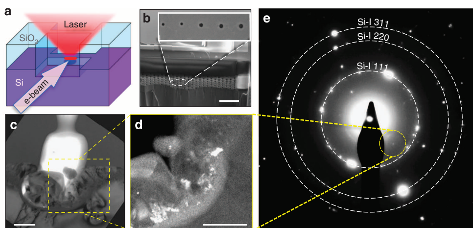
Figure 1 | Ultrashort laser-induced confined microexplosion experiments in silicon. (a) Schematic depiction of a microexplosion at the Si surface under a layer of SiO 2 in a sample cut by a focused ion beam (FIB) for electron diffraction analysis. (b) Scanning electron microscope (SEM) image of FIB-opened voids produced by 440-nJ fs-laser pulses focused to 95 \text{ J cm}^{-2} ; scale bar, 10 \mu\text{m} (the inset shows a magnified top view of the voids located 2 \mu\text{m} apart). (c) TEM bright-field image of a void at the Si/SiO 2 interface (the laser pulse was coming from the top); the shock-wave-modified area in Si is clearly observed under the void in SiO 2 . (d) A magnified dark-field TEM image of the shock-wave-affected area beneath the Si surface. Scale bars, 200 \text{ nm} (c,d). (e) Electron diffraction pattern from the area marked in c. The yellow dashed circle in e indicates the reflections used to generate the dark-field image shown in d.
