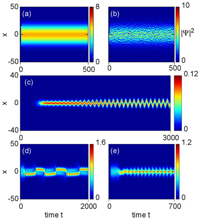
FIG. 4. (Color online) Evolution of the polariton density for Gaussian pumping P(x) = P_{\max} \exp(-x^2/W^2) ( A = 0 ). (a),(b) The condensate densities in the coherent and incoherent cases, respectively. Parameters are R = 1 , \gamma/\gamma_R = 1.5, 5 for (a) and (b), respectively, g = 0.38 , P_{\max}/P_{\text{th}} = 1.7 , W = 44.7 . Frames below show examples of coherent nonstationary states: (c),(d) oscillating wave packets with parameters R = 2.5 , \gamma/\gamma_R = 0.15 , g = 3 , and R = 1 , \gamma/\gamma_R = 0.7 , g = 0.38 , P_{\max}/P_{\text{th}} = 1.8 , W = 15.8 , respectively, and (e) a breather with parameters R = 1 , \gamma/\gamma_R = 0.7 , g = 0.38 , P_{\max}/P_{\text{th}} = 1.6 , W = 15.8 .
