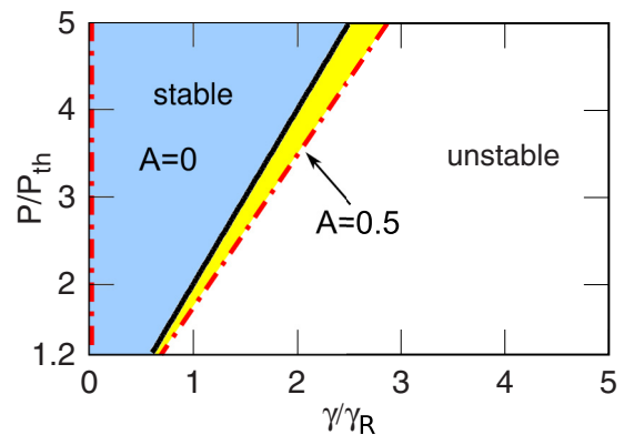
FIG. 3. (Color online) Comparison of stability regions with and without the energy relaxation term included. In both cases, p = 0 . Red dash-dotted lines mark out the stable region for A = 0.5 , which partially overlaps with the stable region for A = 0 . Parameters are R = 1 , g = 1 , g_R = 2g , \gamma_R = 1 , and \gamma \in [0, 5] .
