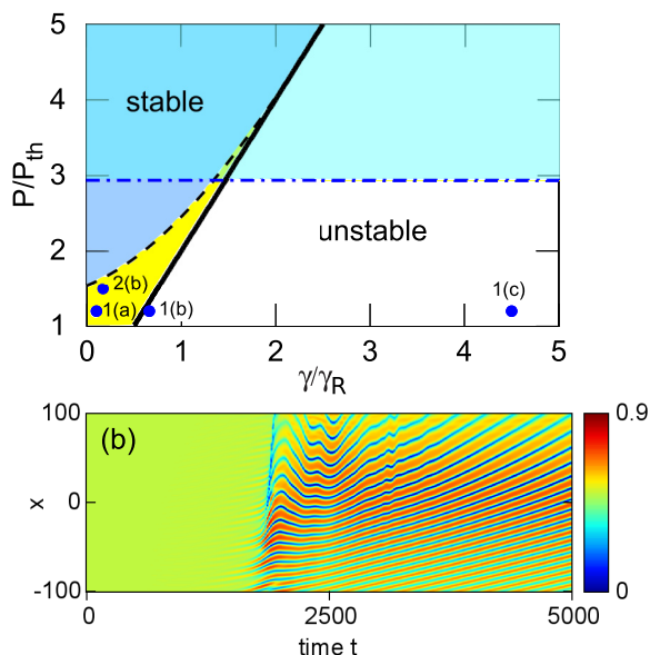
FIG. 2. (Color online) (a) Stability limits of a static condensate created with homogeneous pumping (solid line) and for a uniform condensate flowing with momentum p = 1 (dashed line). Parameters are R = 1 , g = 1 , g_R = 2g , and \gamma_R = 1 . The dash-dotted line corresponds to the critical velocity condition p = c_s = \sqrt{2g|\psi|^2} . The black solid line corresponds to the analytical condition (5) for stability of the homogeneous solution. Blue points correspond to particular cases from Fig. 1. (b) Evolution of |\psi(x,t)|^2 for a uniform flow with homogeneous pumping and momentum p = 1 in the motionally unstable regime, P/P_{\text{th}} = 1.5 , \gamma/\gamma_R = 0.17 .
