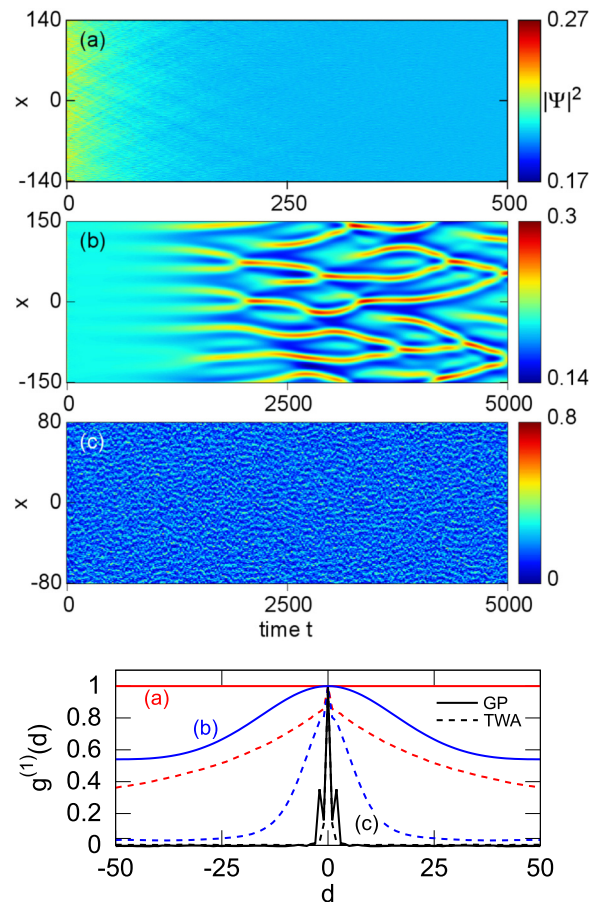
FIG. 1. (Color online) Evolution of the stationary state \psi_0 = \sqrt{(P - P_{\text{th}})/\gamma} with additional noise in the case of homogeneous pumping. The evolution of density in (a) the stable case and (b),(c) the unstable case near and far from the critical point, respectively. Parameters are R = 1 , g = 1 , g_R = 2g , P/P_{\text{th}} = 1.2 , and \gamma/\gamma_R = 0.1, 0.66, 4.5 for (a), (b), and (c), respectively. Bottom panel shows the first-order correlation functions g^{(1)}(d) = \langle \psi^*(x)\psi(x+d) \rangle / \langle |\psi(x)|^2 \rangle at t = t_{\text{max}} , calculated from about 500 samples. Solid lines show g^{(1)} calculated with Eqs. (1) and dashed lines depict the corresponding results with quantum fluctuations included (see text). Corresponding parameters in physical units are time unit \tau = \gamma_R^{-1} = 10 ps, length unit \xi = 3.4 \mu\text{m} , g = 3.4 \mu\text{eV} \mu\text{m}^2 , R = 5.1 \times 10^{-3} \mu\text{m}^2 \text{ps}^{-1} for d = 2 \mu\text{m} , m^* = 5 \times 10^{-5} m_e , and \beta = 0.003 . TWA correlation lengths are (a) \xi = 70 \mu\text{m} , (b) \xi = 17 \mu\text{m} , and (c) \xi = 3 \mu\text{m} .
