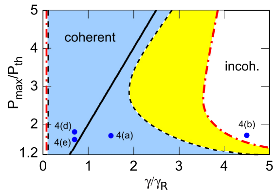
FIG. 5. (Color online) Stability regions for Gaussian pumping profiles. The lines mark out the coherent regions for narrower pumping of width W = 15.8 (dash-dotted lines) and for wider pumping of width W = 44.7 (dashed lines). The black solid line corresponds to the analytical stability condition of a homogeneous condensate [19]. Blue points correspond to particular cases from Fig. 4. Parameters are R = 1 , g = 0.38 , g_R = 2g , and \gamma_R = 1 . For the choice of scaling parameters as in Fig. 1, the width of the pumping is W = 54 \mu\text{m} (dash-dotted lines) and W = 152 \mu\text{m} (dashed lines).
