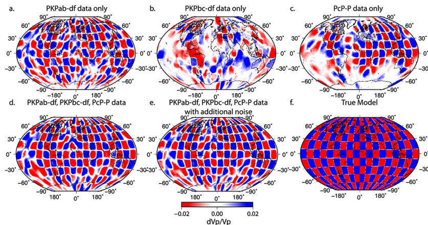
Figure 13. The recovered model using (a) the PKPab-df data set only, (b) the PKPbc-df data set only, (c) the PcP-P data set only, (d) all three data sets, and (e) all three data sets with additional noise added. Also shown is (f) the true model used in the checkerboard resolution tests to produce synthetic data. This input model (Figure 13f) has alternating 20^\circ squares of \pm 2\% velocity perturbations.
