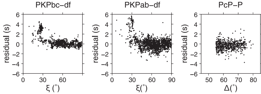
Figure 5. (left) The PKPbc-df , (middle) PKPab-df , and (right) PcP-P differential travel time data sets used in this study. Travel time residuals are plotted with respect to \xi(^{\circ}) (left, middle) or epicentral distance \Delta(^{\circ}) (right).
