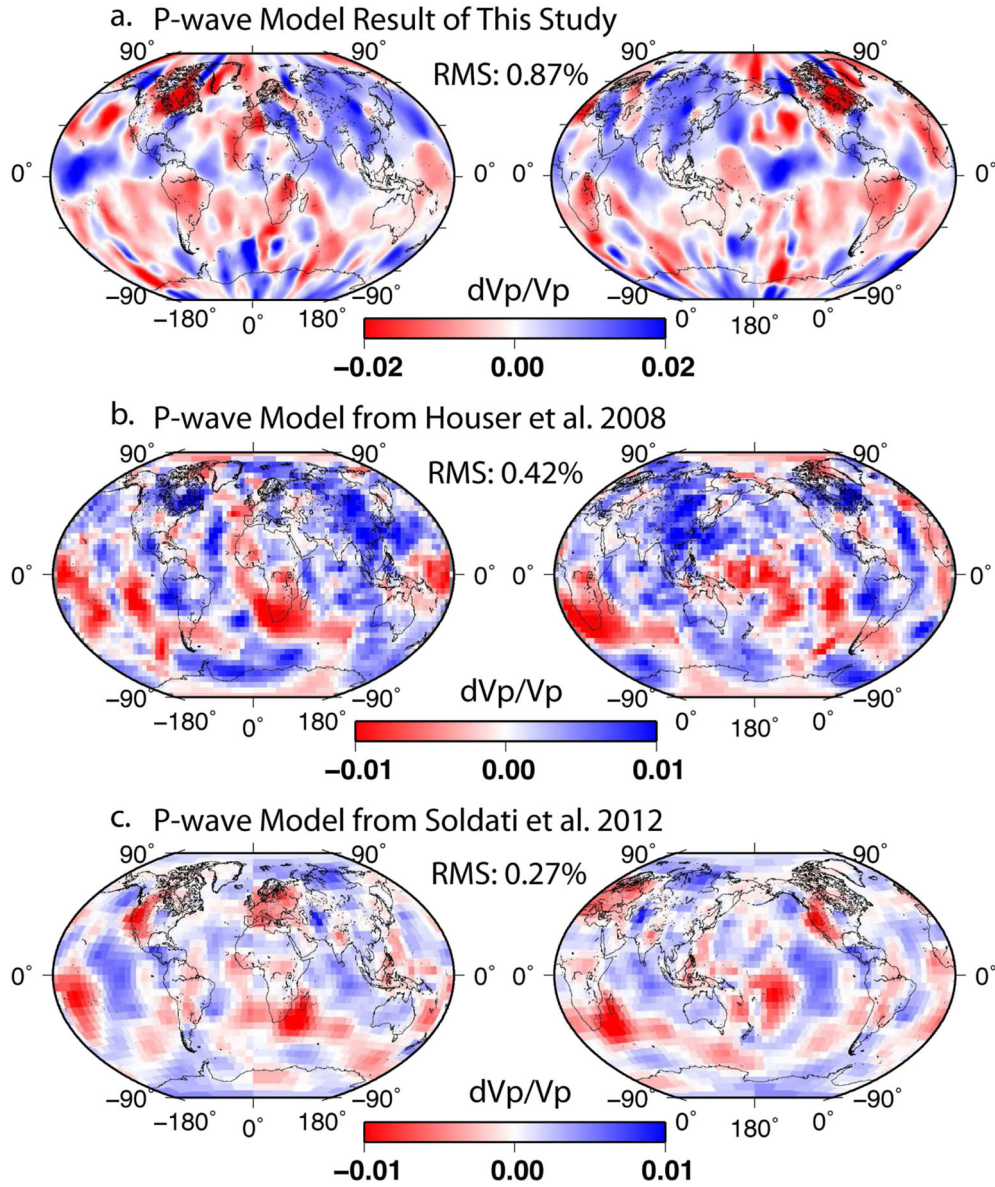
Figure 15. (a) The P wave model of the lowermost 300 km of the mantle from this study. (b) The P wave model of the lowermost 200 km of the mantle from Houser et al. [2008]. (c) The P wave model of the lowermost 200 km of the mantle from Soldati et al. [2012]. Note the differences in the color scale ranges for the different models. The root-mean-square (RMS) value of each model is noted.
