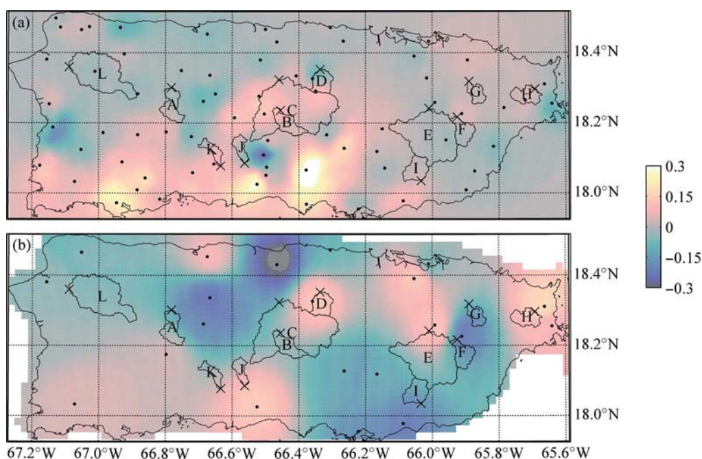
Fig. 4. The trend [ \% \text{ yr}^{-1} ] from 1955 to 2010 for annual mean (a) P and (b) PET. Significant as well as insignificant trends are shown. The points mark stations with > 20 yr time series of (a) P , and (b) T_{\min} and T_{\max} (used to derive PET, see Sect. 4.2). Catchments identified by letters and stream gauges by crosses.
