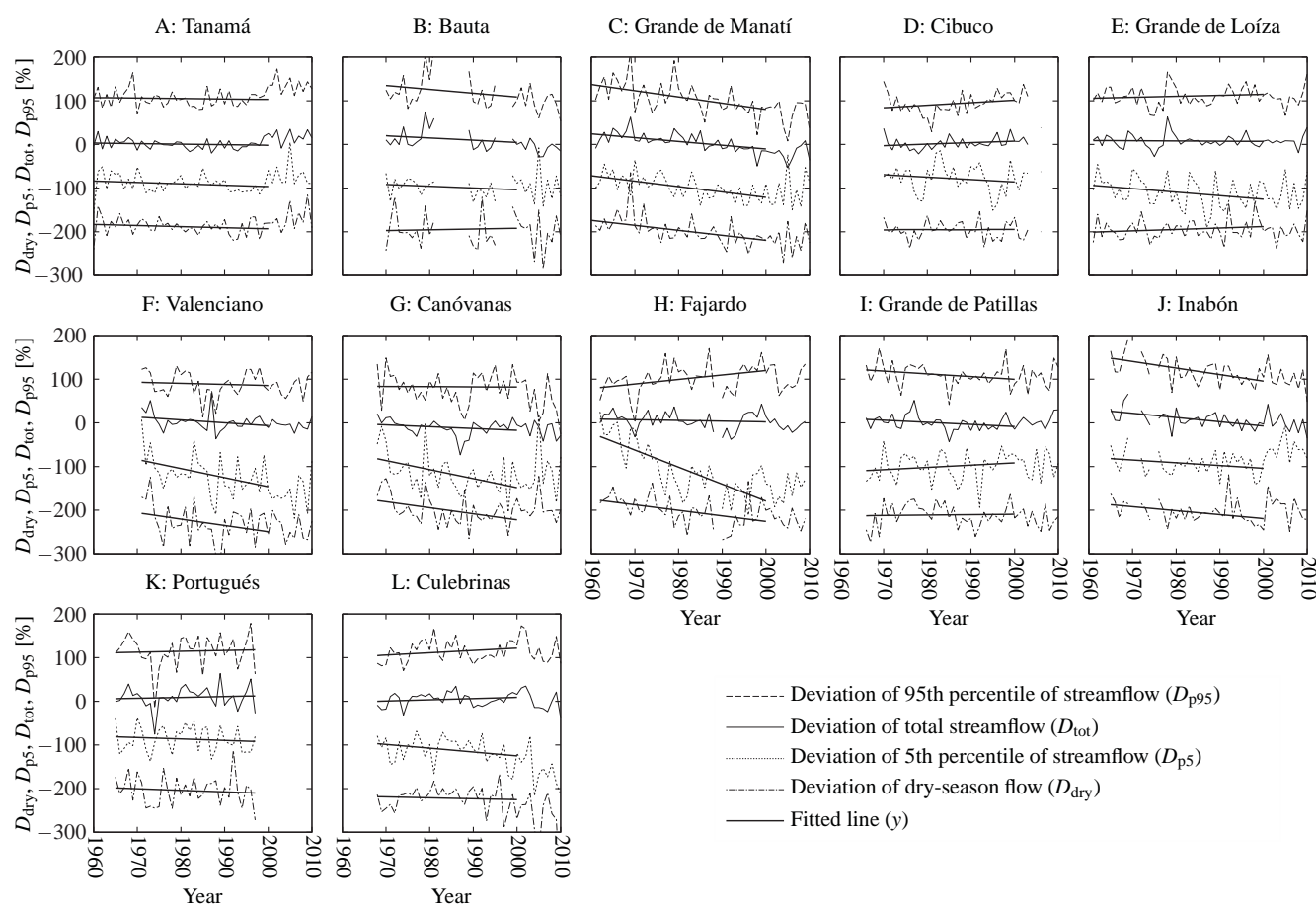
Fig. 6. Annual time series of D_{p95} , D_{tot} , D_{p5} , and D_{dry} (displayed, respectively, from top to bottom in each panel; calculated using Eq. 4) and fitted trend lines. For clarity the D_{p95} , D_{p5} , and D_{dry} time series were offset by +100, -100, and -200 %, respectively.
