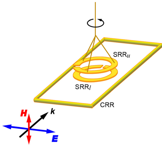
FIG. 1. Schematic representation of the tri-resonator magnetoelastic metamaterial device. The CRR and lower SRR ( SRR_l ) are fixed to the dielectric substrate. The upper SRR ( SRR_u ) is suspended by a thin rubber wire and is free to rotate about the common axis. The directions of the incident electric ( E ) and magnetic ( H ) fields and wavevector ( k ) are also shown.
