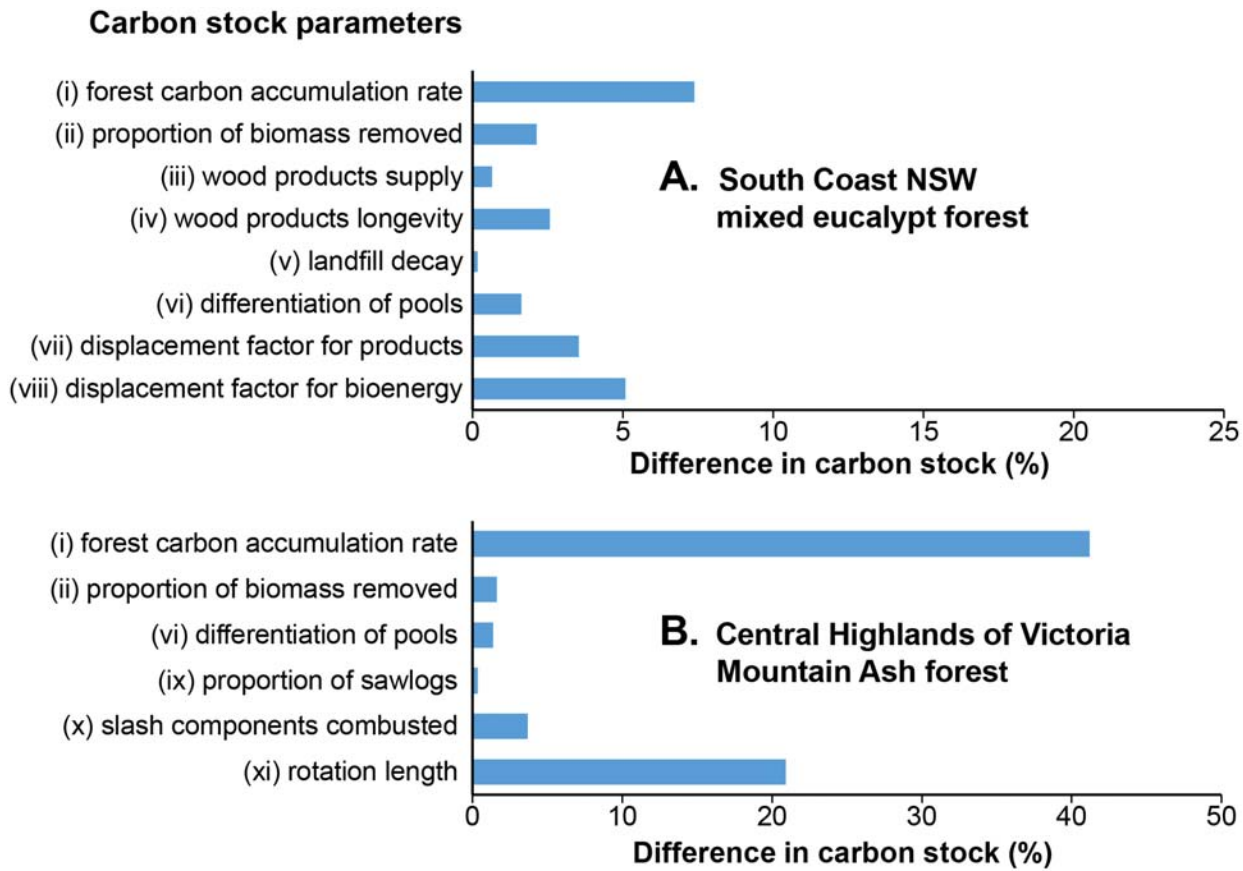
Fig 4. Differences in simulated carbon stocks (tC ha -1 ) as percentages of the total system carbon stock. Differences were calculated from use of minimum or maximum values of parameters listed in Tables B and C in S3 Appendix in a simulation for 50 years in (A) mixed native eucalypt forest on the South Coast of NSW, and (B) Mountain Ash forest in the Central Highlands of Victoria.
