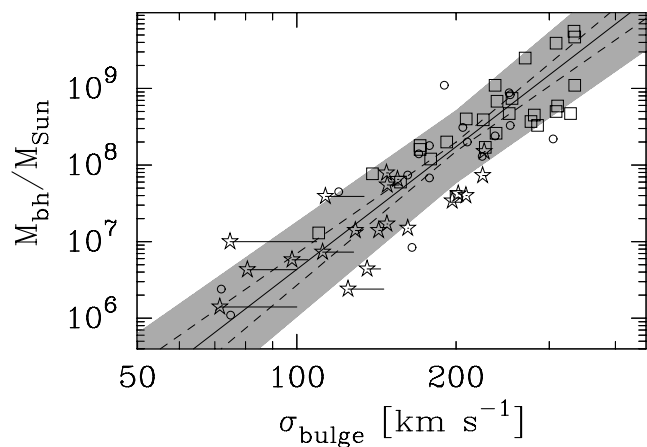
Figure 7. Adaptation of Fig. 5 such that (i) the central velocity dispersions of the barred galaxies, \sigma_{\text{obs}} , have been adjusted to a new ‘ \sigma_{\text{bulge}} ’ value following equation (11) using C = 0.7 , and (ii) the lines and shaded area now trace the M_{\text{bh}}-\sigma relation defined by the non-barred galaxies, as given by the second last entry in Table 2. Squares, stars and circles denote elliptical, barred and non-barred disc galaxies, respectively. The small lines emanating from the barred galaxies show their previous location in Fig. 5.
