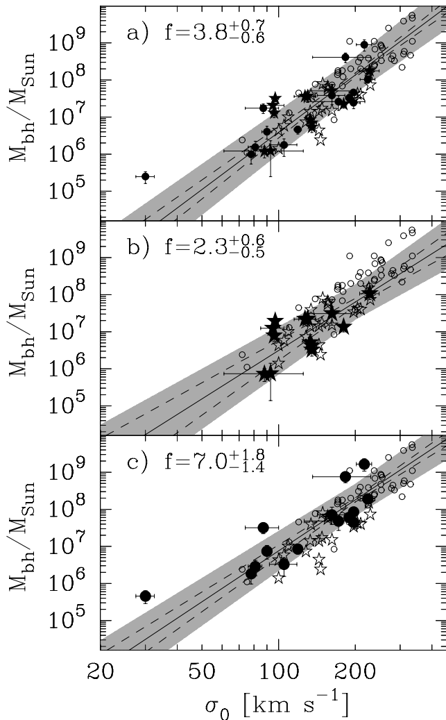
Figure 4. Similar to Fig. 3, except that the optimal f -factor (inset in figure) to bring the AGN virial products in line with the corresponding M_{\text{bh}}-\sigma relation has been used. As in Fig. 3, the filled symbols in panels (a), (b) and (c) correspond to the full, barred and non-barred AGN sample, while the open stars and circles correspond to the barred and non-barred galaxies with direct SMBH mass measurements. A linear regression of \log M_{\text{bh}} on \log \sigma for the full, barred and non-barred sample of galaxies with direct SMBH mass measurements (see Section 2.1) has been used to construct the three different relations (given by equations 1, 3 and 2) shown in panel (a), (b) and (c), respectively.
