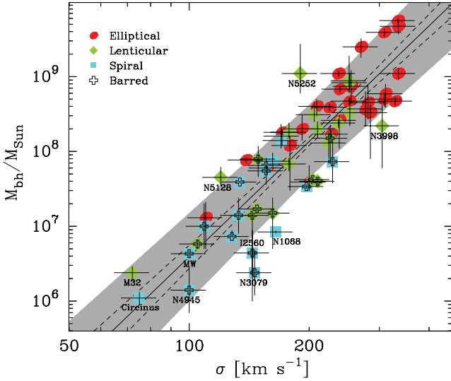
Figure 2. Updated M_{\text{bh}}-\sigma relation, containing 64 galaxies with reliable SMBH masses (see table 1 from Graham 2008b, and Table 1 from this paper). The solid line is derived from a regression of \log M_{\text{bh}} on \log \sigma , assuming a 10 per cent uncertainty on the velocity dispersions \sigma (see equation 1). The dashed lines trace the 1\sigma uncertainty on this relation, while the shaded area extends this boundary by 0.43 dex (the rms scatter about the relation) in the \log M_{\text{bh}} direction. The barred galaxies can be seen to dominate the distribution of points below the best-fitting line at low masses.
