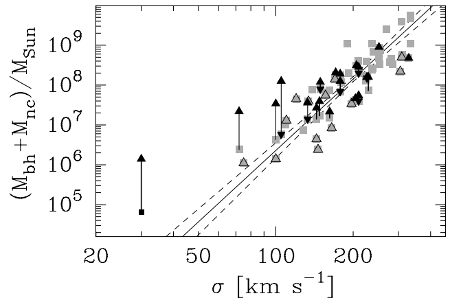
Figure 8. Adaptation of Fig. 5 using the 64 galaxies with direct SMBH masses (plus NGC 4395, lower left). The solid upward pointing arrowheads show the location of the combined black hole masses (Graham 2008b and Table 1) plus the nuclear star cluster mass (Graham & Spitler 2009; Graham, in preparation). For seven systems with only an upper limit to the nuclear cluster mass, a bi-directional arrow denotes the possible (M_{\text{bh}} + M_{\text{nc}}) mass range. Galaxies with dust obscured nuclei, and/or significant AGN whose flux may hide a nuclear star cluster, are plotted with open triangles on top of the mass of the SMBH.
