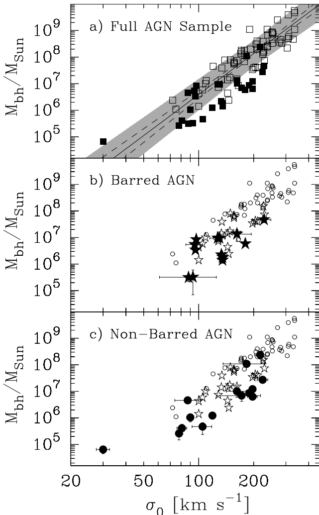
Figure 3. Panel (a): an updated version of Fig. 1 using the galaxies described in Section 2. One can see that the full sample of 28 AGN (filled squares) with RM-derived virial products overlap with some of the 64 galaxies with direct SMBH mass measurements (open squares). The lines and shaded region pertain to equation (1). Panels (b) and (c): both AGN and galaxies with bars are denoted by a star, while those without by a circle. Filled and open symbols pertain to our sample of AGN and galaxies with direct SMBH mass measurements, respectively. In all panels, as in Fig. 1, an f -factor of 1 has been used to plot the AGN virial products by the filled symbols.
