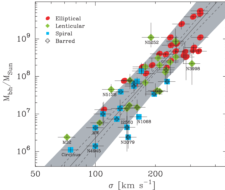
Figure 5. Similar to Fig. 2, except that a regression of \log \sigma on \log M_{\text{bh}} for the 64 galaxies with direct SMBH mass measurements has been used (see Table 2).
