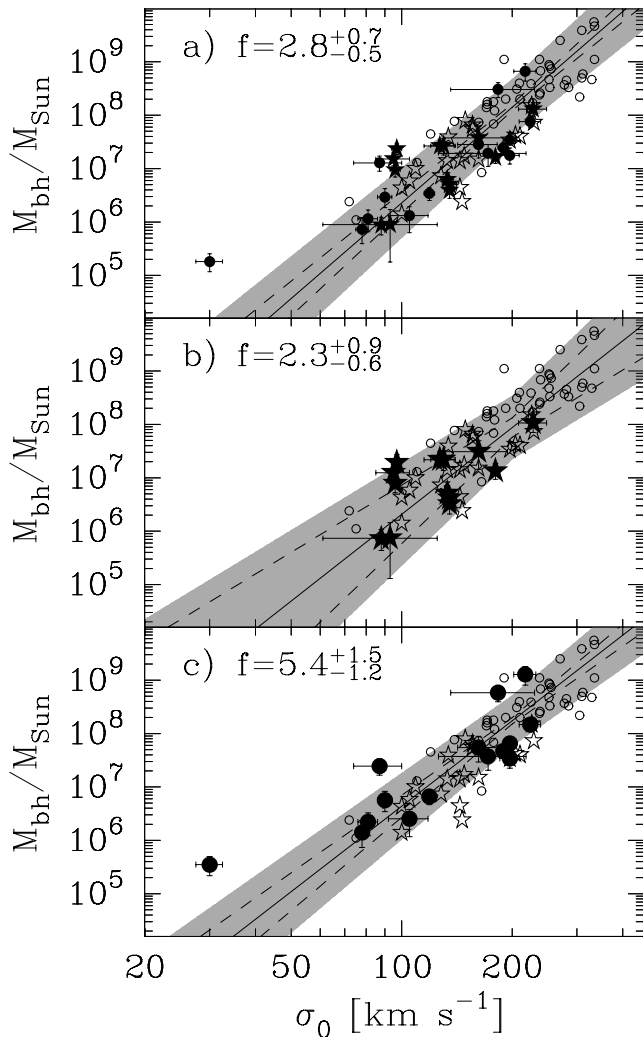
Figure 6. Similar to Fig. 4, except that a regression of \log \sigma on \log M_{\text{bh}} for the galaxies with direct SMBH mass measurements has been used to construct the three linear regressions in each panel (see Table 2). Excluding NGC 5548 gives f = 2.6^{+0.6}_{-0.4} , 2.3^{+0.9}_{-0.6} and 4.9^{+1.4}_{-1.1} in panels (a), (b) and (c), respectively.
