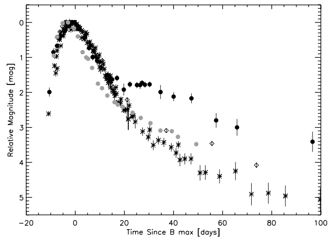
Figure 12. uvw1 -Band light curves of SNe Ia aligned by peak magnitude. Seven normal SNe Ia (asterisks/open diamonds) are shown compared to two subluminous SNe Ia (SNe 2005ke and 2007on). SN 2005ke (dark filled circles) breaks to a bright plateau, while SN 2007on (gray filled circles) breaks at an early epoch, but to a flat decline fainter than that of SN 2005ke. SN 2005df, a normal-luminosity SN Ia (open diamonds), features an early-time light curve similar to that of the other normal SNe Ia, but breaks at a late epoch to a very shallow decline.
