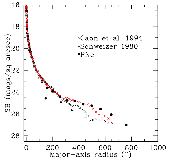
Fig. 6. Surface density profiles for the PNe and stars in NGC 1316. Red and black crosses mark the NE and SW major-axis B -band surface brightness profiles respectively (Caon et al., 1994). The hollow squares show the measurements from Schweizer (1980). The agreement with the NE major axis between 200'' and 500'' indicates that the PNe do trace the light, except where dust obscures the observations.
