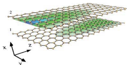
FIG. 1 Schematic of a nonlinear graphene coupler composed of two layers of graphene. The color pattern demonstrates how a plasmon beam excited in the top layer tunnels to the bottom layer (numerical results not to scale).
