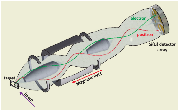
Fig. 2. (Color online) Schematic view of the magnetic pair spectrometer. (Courtesy of Caleb Gudu, ANU)
