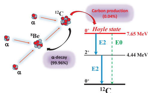
Fig. 1. 3\alpha -process and the formation of ^{12}\text{C} .
