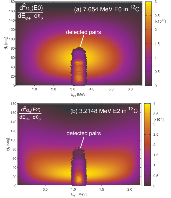
Fig. 4. (Color online) Calculated double differential pair emission rates for (a) the 7.654 MeV E0 and (b) the 3.2148 MeV E2 transitions in ^{12}\text{C} . The distribution of simulated events of electron–positron pairs detected with the magnetic pair spectrometer is also shown (“detected pairs”).
