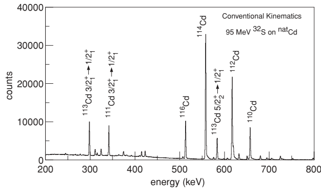
FIG. 1. Spectrum of \gamma rays observed at +65^\circ to the beam axis in coincidence with backscattered ^{32}\text{S} beam ions. This spectrum represents all of the data for the field-up direction in the detector at +65^\circ , obtained during the precession measurement on the Cd target.
