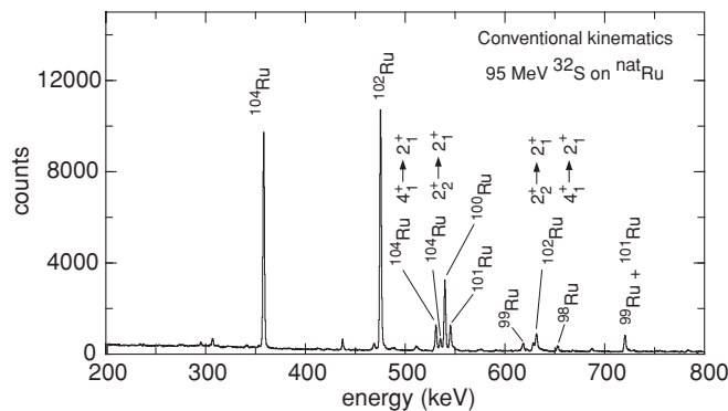
FIG. 3. Spectrum of \gamma rays observed at +65^\circ to the beam axis in coincidence with backscattered ^{32}\text{S} beam ions. This spectrum represents the data for the field-up direction in the detector at +65^\circ , obtained during the precession measurement on the natural Ru target.
