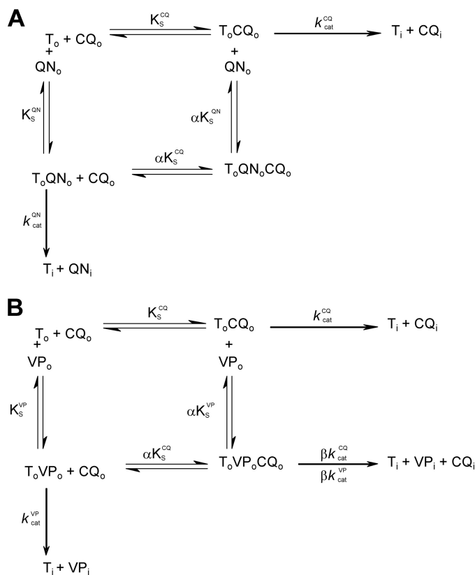
FIGURE 11. Proposed reaction schemes describing the interaction of PfCRT Dd2 with chloroquine, quinine and verapamil. A, chloroquine (CQ) and quinine (QN) act as full mixed-type inhibitors of PfCRT Dd2 -mediated transport. PfCRT Dd2 can bind chloroquine and quinine at distinct sites. The ternary complex ( T_o QN_o CQ_o ) is inactive. T_o represents PfCRT Dd2 in the outward facing conformation ( i.e. the extracellular face of the protein when in the oocyte plasma membrane and its luminal face when in the membrane of the digestive vacuole), and T_i represents PfCRT Dd2 in the inward facing conformation ( i.e. the cytosolic face of the protein when in the membrane of either the oocyte or the digestive vacuole). Likewise, CQ_o and QN_o are the extracellular/luminal drug concentrations, and CQ_i and QN_i are the cytosolic drug concentrations. K_S^{CQ} and K_S^{QN} are the respective quinine and chloroquine dissociation constants for PfCRT Dd2 ; \alpha is the factor by which K_S^{CQ} and K_S^{QN} change when the other drug is already bound to the transporter; and k_{cat}^{CQ} and k_{cat}^{QN} describe the rate constants of chloroquine and quinine transport. B, chloroquine and verapamil (VP) act as partial mixed-type inhibitors of PfCRT Dd2 -mediated transport. The ternary complex ( T_o VP_o CQ_o ) retains a low level of activity. VP_o and VP_i are the extracellular/luminal and cytosolic concentrations of verapamil, respectively. K_S^{VP} is the verapamil dissociation constant for PfCRT Dd2 ; \alpha is the factor by which K_S^{CQ} and K_S^{VP} change when the other drug is already bound to the transporter; k_{cat}^{VP} describes the rate constant of verapamil transport; and \beta is the factor by which verapamil and chloroquine affect the rate constant of the other drug's transport.
