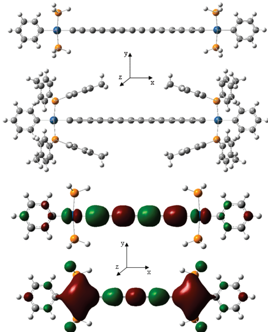
Figure 2. Top panel: trans,trans -( \text{H}_3\text{P} ) _2 ( \text{C}_6\text{H}_5 )Pt( \text{C}\equiv\text{C} ) _7 Pt( \text{C}_6\text{H}_5 )( \text{PH}_3 ) _2 ( PtC 14 Pt* ). Second panel: trans,trans -( p -MeC 6 H 4 ) _3 P( \text{C}_6\text{H}_5 )Pt( \text{C}\equiv\text{C} ) _7 Pt( \text{C}_6\text{H}_5 ){P( p -C 6 H 4 Me) _3 } _2 ( PtC 14 Pt* ). Third panel and fourth panel: Iso-density plots of the electron densities in the highest-occupied (third panel) and lowest-unoccupied (fourth panel) Kohn–Sham orbitals of PtC 8 Pt* .
