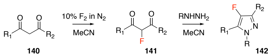
Figure 1.52: Continuous gas/liquid–liquid/liquid flow process for the synthesis of 4-fluoropyrazoles.
