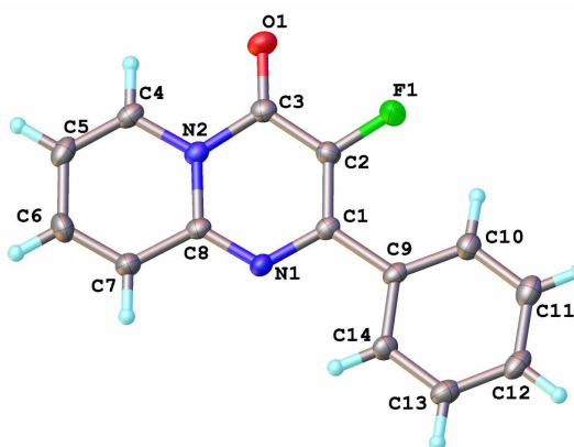
Figure 4.31: Molecular structure of 287 as determined by x-ray crystallography.
