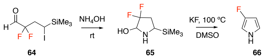
Figure 1.27: Synthesis of unprotected 3-fluoropyrrole 66 .
