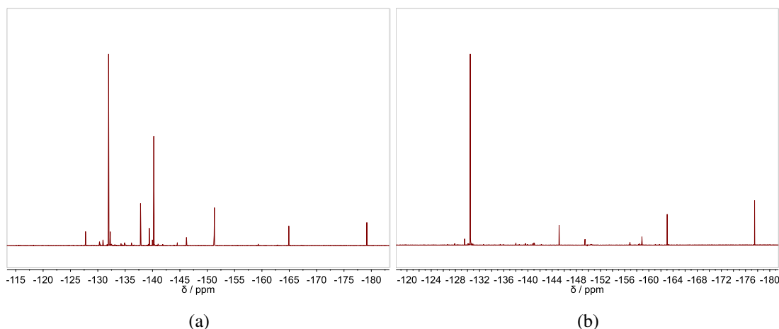
Figure 2.12: Comparison of the 19 F NMR spectra of the crude reaction mixtures from fluorination of 41 (a) and 155 (b) with Selectfluor TM .
