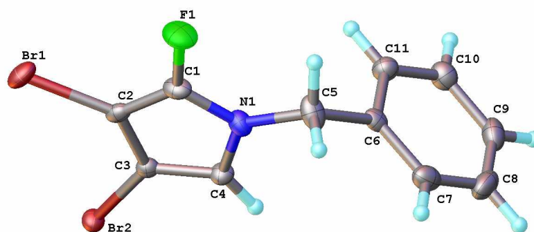
Figure 3.20: Molecular structure of 203 as confirmed by x-ray crystallography.
