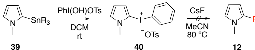
Figure 1.20: Attempted synthesis of fluoropyrrole 12 via an intermediate iodonium salt.
