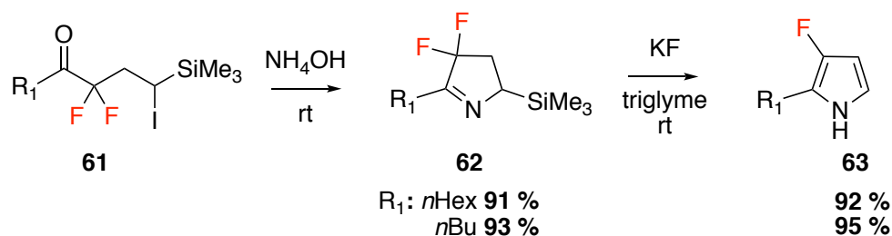
Figure 1.26: Synthesis of 2-alkyl-3-fluoropyrroles ( 63 ) from \alpha,\alpha -difluoro- \gamma -iodo- \gamma -TMS ketones.
