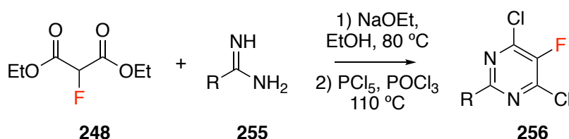
Figure 4.8: Synthesis of 2-substituted 4,6-dichloro-5-fluoropyrimidine derivatives ( 256 ).
