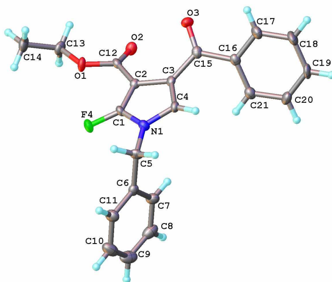
Figure 3.44: Molecular structure of 227 as determined by x-ray crystallography.
