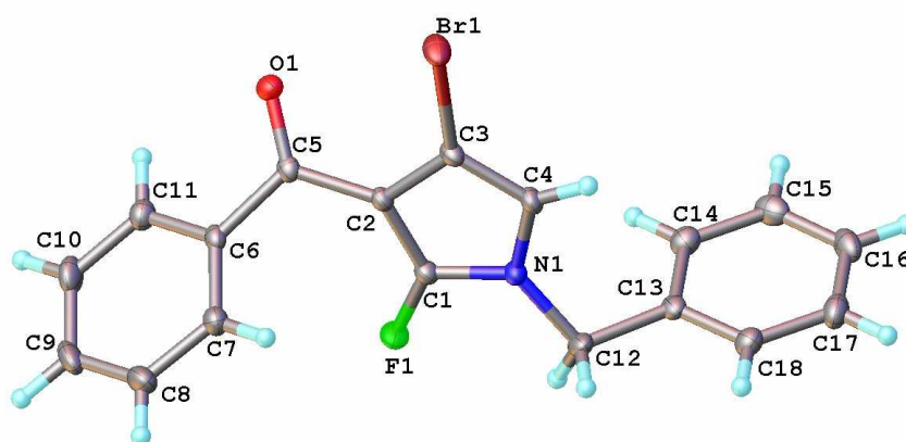
Figure 3.36: Molecular structure of 223 as confirmed by x-ray crystallography.
