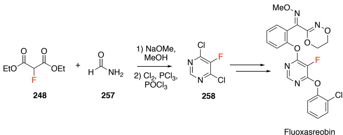
Figure 4.9: Synthesis of commercial herbicide Fluoxastrobin from diethyl 2-fluoromalonate.
