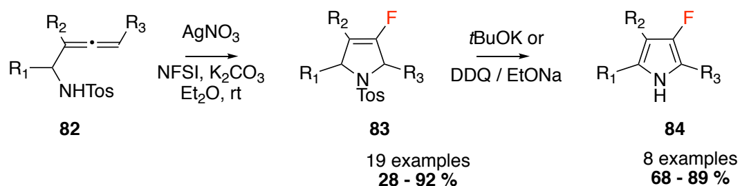
Figure 1.31: Silver catalysed aminofluorination of allenes and subsequent aromatisation to 3-fluoropyrrole derivatives.
