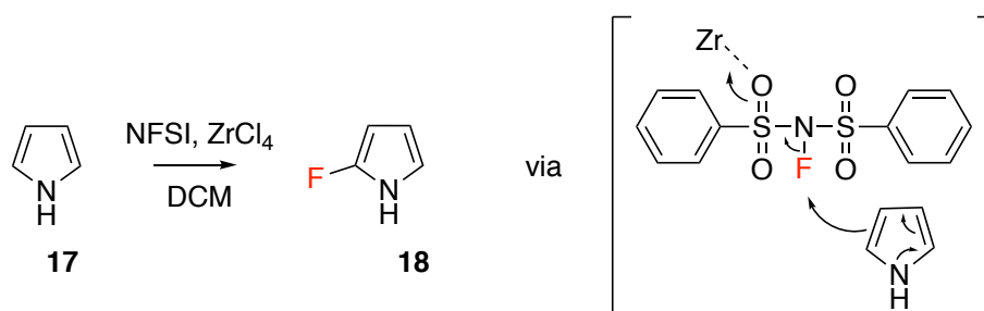
Figure 1.11: Lewis acid catalysed fluorination of pyrrole using NFSI.
