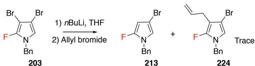
Figure 3.37: Attempted synthesis of 2-fluoro-3-allyl-4-bromo- N -benzylpyrrole.
