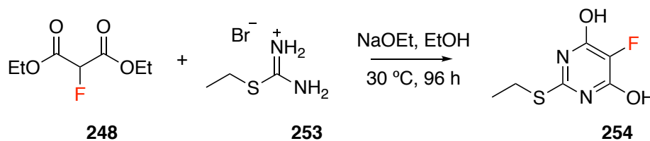
Figure 4.7: Synthesis of 5-fluoropyrimidine derivative 254 from diethyl 2-fluoromalonate 248 .
