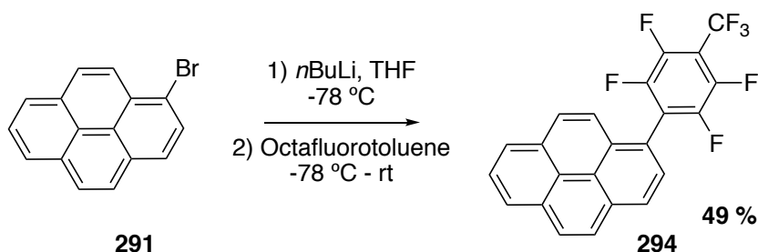
Figure 5.6: Synthesis of 1-(2,3,5,6-tetrafluoro-4-(trifluoromethyl)phenyl)pyrene ( 294 ).
