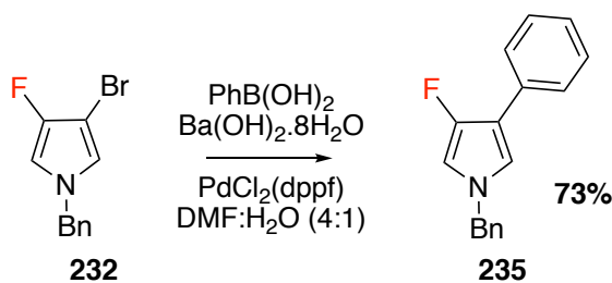
Figure 3.58: Synthesis of 3-fluoro-4-phenyl- N -benzylpyrrole.
