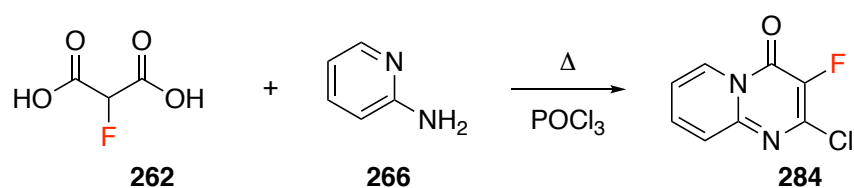
Figure 4.24: Proposed synthesis of 2-chloro-3-fluoro-4 H -pyrido[1,2- a ]pyrimidin-4-one 284 .
