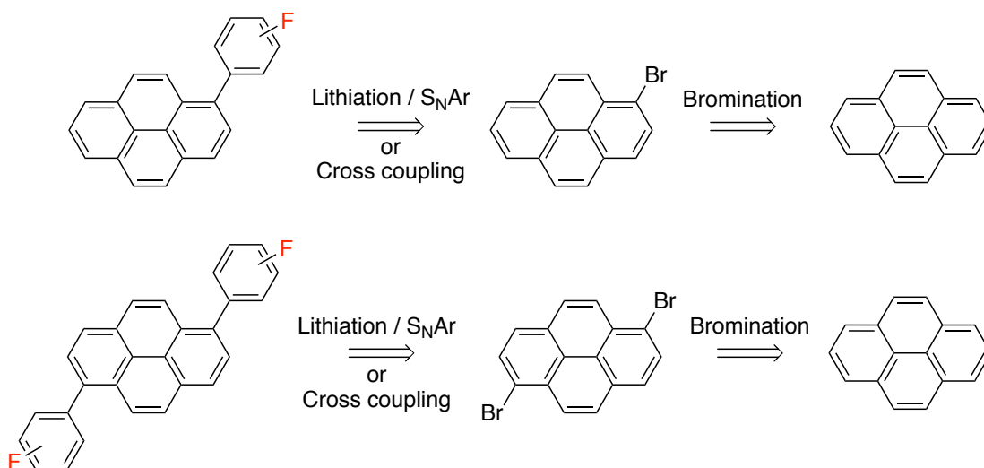
Figure 5.1: Proposed synthetic route to fluorinated pyrene derivatives.
