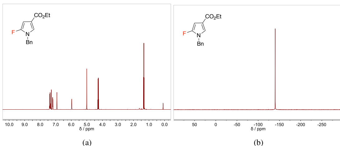
Figure 3.33: 1 H (a) and 19 F (b) NMR spectra of isolated ethyl 2-fluoro- N -benzylpyrrole-4-carboxylate ( 217 ).
