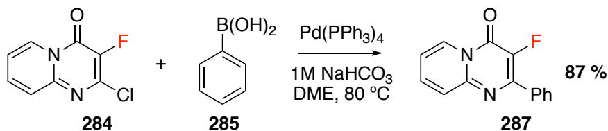
Figure 4.30: Synthesis of 2-phenyl-3-fluoro-4 H -pyrido[1,2- a ]pyrimidin-4-one ( 287 ).
