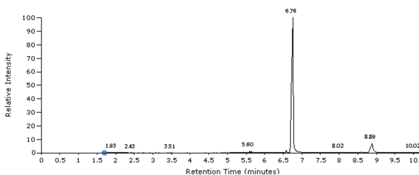
Figure 5.3: GC-MS trace showing the formation of mono- and dibromopyrene products.
