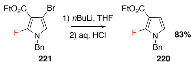
Figure 3.40: Synthesis of 2-fluoro- N -benzylpyrrole-3-carboxylate.
