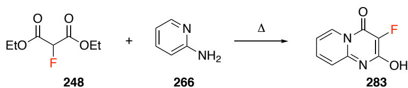
Figure 4.23: Attempted thermal condensation of 2-fluoromalonate ester 248 and 2-aminopyridine.
