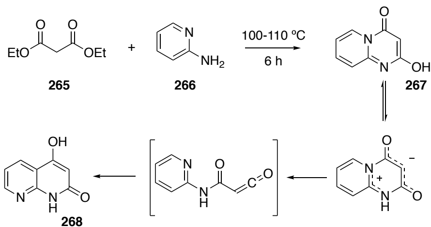
Figure 4.15: Thermal condensation of 2-aminopyridine and diethyl malonate.
