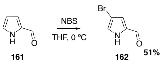
Figure 2.10: Bromination of pyrrole-2-carboxaldehyde using NBS.
