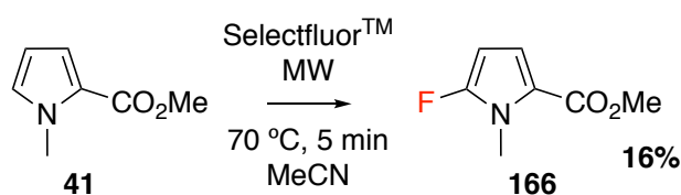
Figure 2.13: Synthesis of methyl N -methyl-5-fluoropyrrole-2-carboxylate ( 166 ) with Selectfluor TM under MW conditions.
