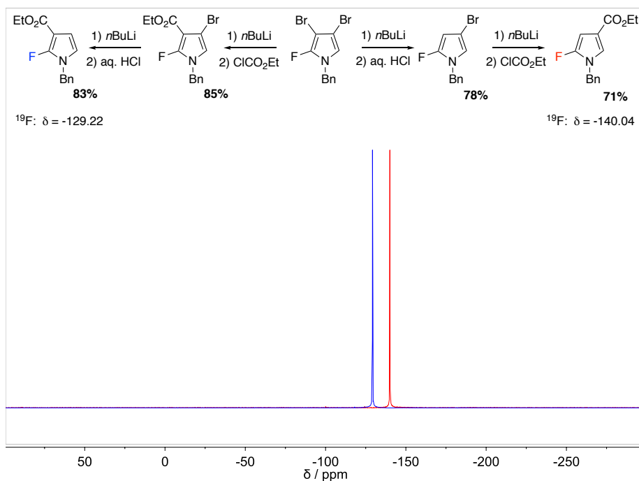
Figure 3.41: Overlaid 19 F NMR spectra of fluorinated regioisomers 217 and 220 .
