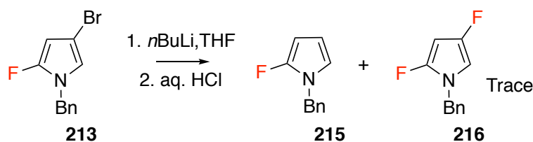
Figure 3.31: Attempted synthesis of 2,4-difluoropyrrole derivative 216 .
