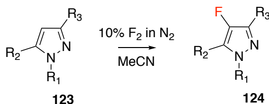
Figure 1.43: Synthesis of 4-fluoropyrazole derivatives using F 2 gas.
