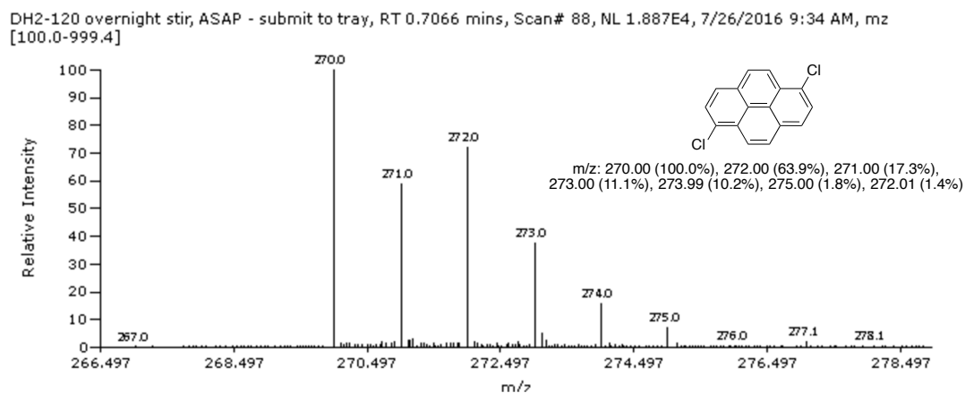
Figure 5.11: ASAP analysis showing the correct mass associated with 1,6-dichloropyrene.
