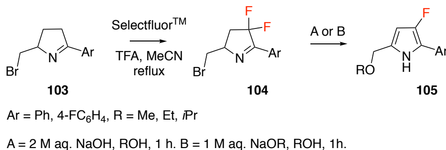
Figure 1.36: Synthesis of 3-fluoropyrroles bearing an alkoxyethyl substituent.
