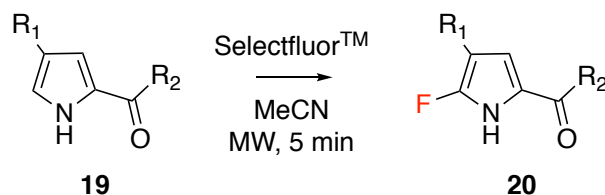
Figure 1.12: Microwave assisted fluorination of substituted pyrrole derivatives using Selectfluor™.
