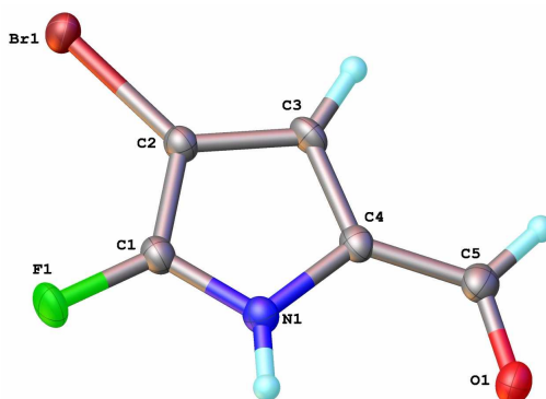
Figure 2.11: Molecular structure of 163 as determined by x-ray crystallography.
