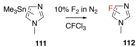
Figure 1.40: Synthesis of 2- and 5-fluoroimidazoles from organostannane derivatives.
