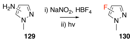
Figure 1.46: Photochemical Balz-Schiemann reaction for the synthesis of 3-, 4- and 5-fluoropyrazoles.
