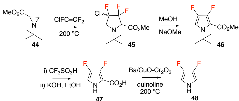
Figure 1.22: Synthesis of 3,4-difluoropyrrole ( 48 ) from t -butyl aziridine derivative ( 44 ).
