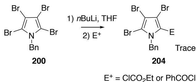
Figure 3.22: Attempted synthesis of substituted tribromopyrrole derivatives.
