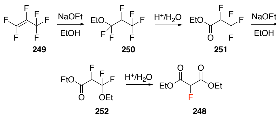
Figure 4.6: Synthesis of 2-fluoromalonate esters from HFP.
