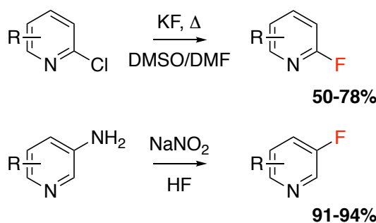
Figure 1.6: Synthesis of 2-fluoro and 3-fluoropyridine derivatives.
