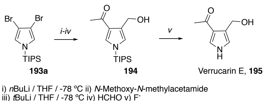
Figure 3.9: Sequential metal-halogen exchange approach towards verrucarin E.
