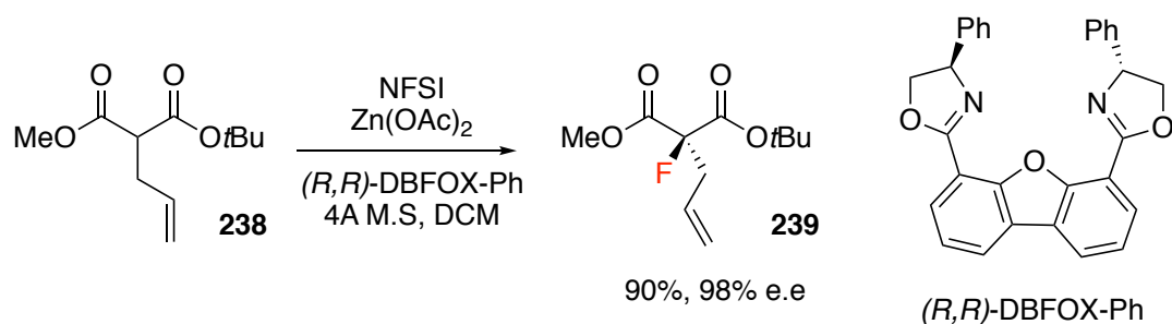
Figure 4.2: Assymmetric fluorination of malonic ester derivative 238 with NFSI.
