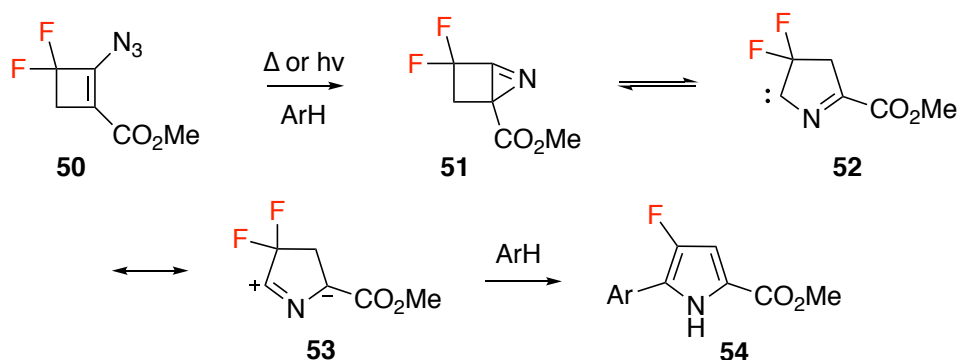
Figure 1.24: Buhr's synthesis of 5-aryl-3-fluoropyrrole derivatives 54 .
