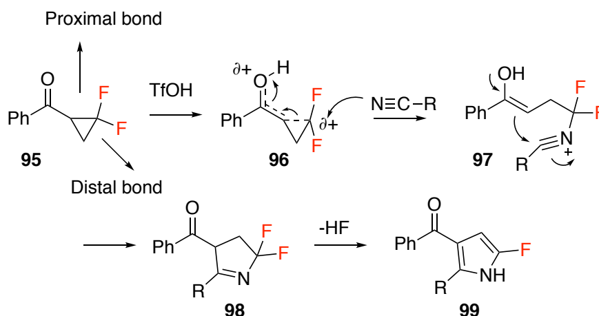
Figure 1.34: TfOH promoted synthesis of 2-fluoropyrrole derivatives from gem -difluorocyclopropyl ketones.
