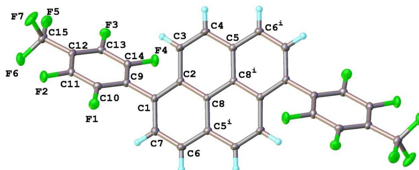
Figure 5.9: Molecular structure of 295 as determined by x-ray crystallography.
