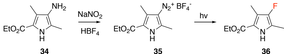
Figure 1.18: Photochemical modification of the Balz-Schiemann reaction.
