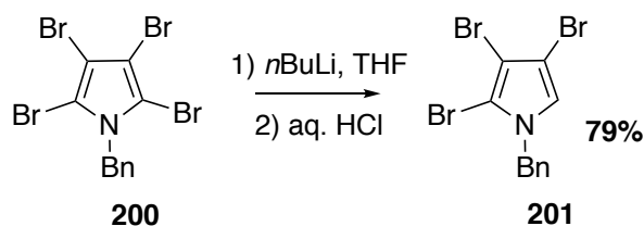
Figure 3.16: Hydrodebromination of 2,3,4,5-tetrabromo- N -benzylpyrrole.
