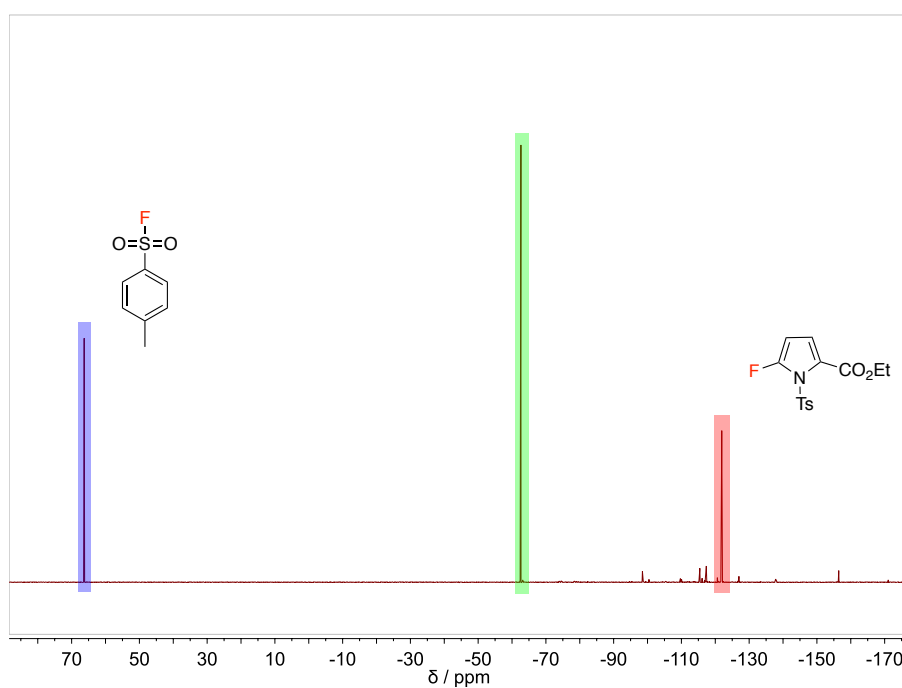
Figure 2.18: 19 F NMR of the crude product mixture showing the formation of fluorinated by-product (blue) and desired product (red) against the fluorinated reference (green).
