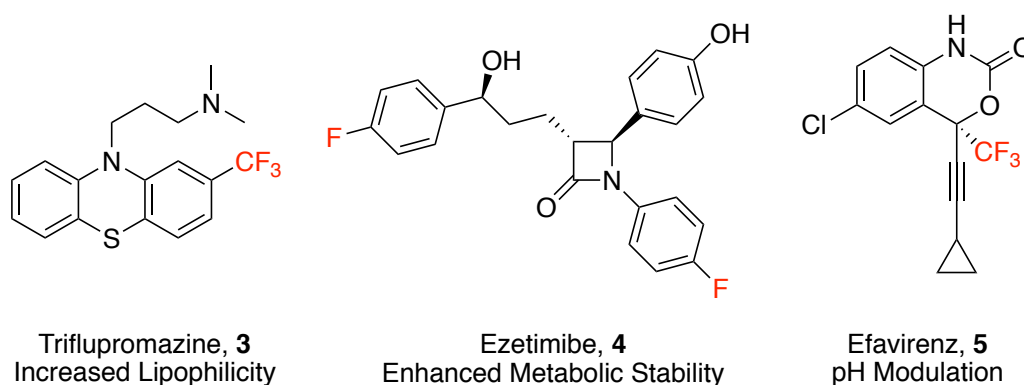
Figure 1.2: Examples of strategically fluorinated pharmaceuticals 3 , 4 and 5 .
