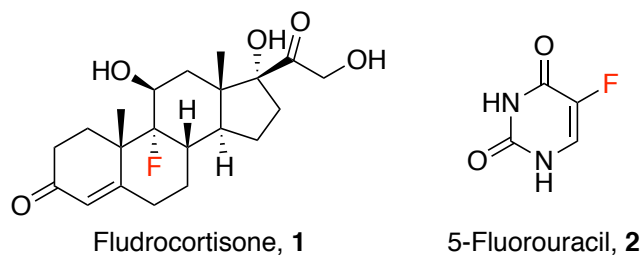
Figure 1.1: Structures of the first fluorine containing drugs.
