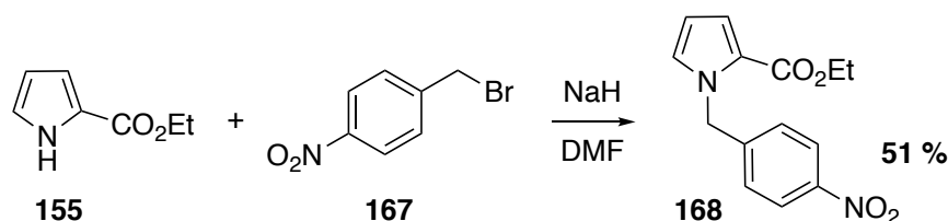
Figure 2.14: Synthesis of ethyl N -(4-nitrobenzyl)pyrrole-2-carboxylate ( 168 ).
