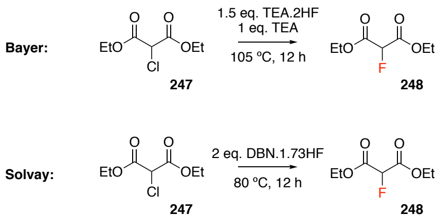
Figure 4.5: Halogen exchange protocols for the synthesis of 2-fluoromalonate 248 .
