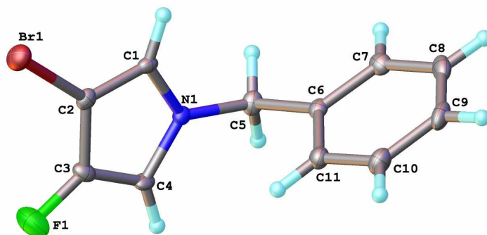
Figure 3.56: Molecular structure of 232 as determined by x-ray crystallography.
