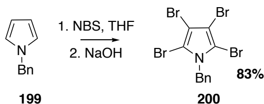
Figure 3.14: Bromination of N -benzylpyrrole using NBS.
