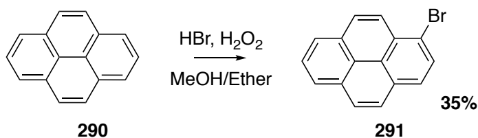
Figure 5.2: Synthesis of 1-bromopyrene ( 291 ) with HBr and H 2 O 2 .
