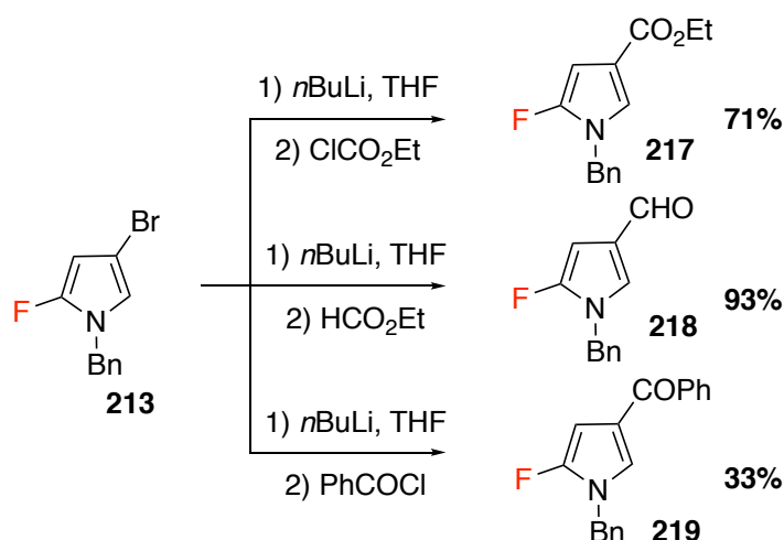
Figure 3.32: Synthesis of 2-fluoro-4-substituted pyrrole derivatives 217 , 218 and 219 .
