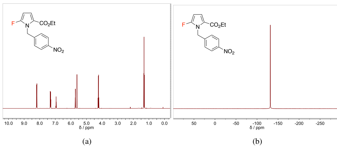
Figure 2.15: 1 H (a) and 19 F (b) NMR spectra of isolated ethyl N -(4-nitrobenzyl)-5-fluoropyrrole-2-carboxylate 169 .
