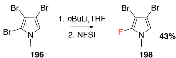
Figure 3.13: Synthesis of 2-fluoro-3,4-dibromopyrrole derivative 198 .
