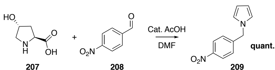
Figure 3.24: Synthesis of N -(4-nitrobenzyl)pyrrole via redox reaction of 4-hydroxy-L-proline.
