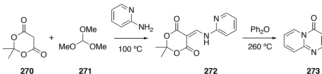
Figure 4.17: Synthesis of pyrido[1,2- a ]pyrimidin-4-one ( 273 ) using Meldrum's acid.
