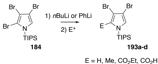
Figure 3.8: Metal-halogen exchange of tribromopyrrole derivative 184 and subsequent reactions with various electrophiles.
