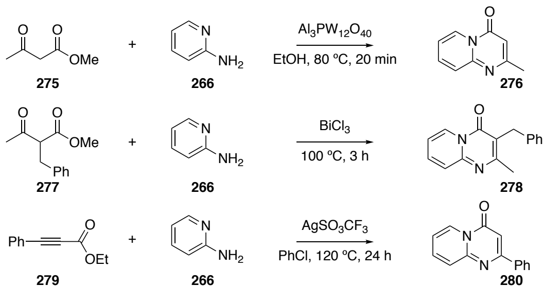
Figure 4.19: Metal catalysed synthesis of pyrido[1,2- a ]pyrimidin-4-ones derivatives.
