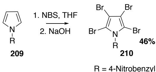
Figure 3.25: Bromination of N -(4-nitrobenzyl)pyrrole using NBS.
