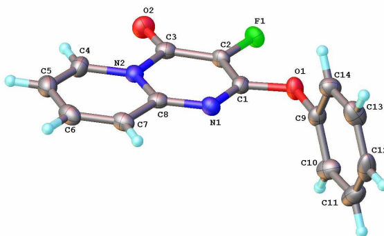
Figure 4.29: Molecular structure of 286 as determined by x-ray crystallography.
