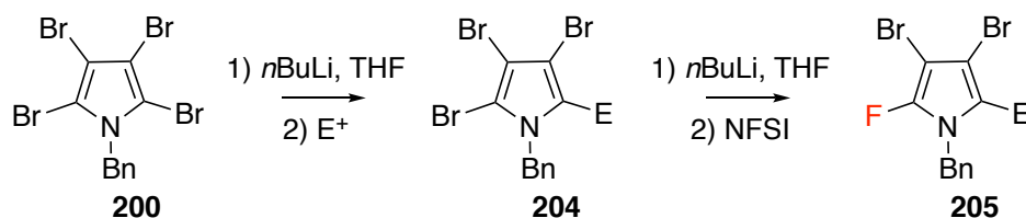
Figure 3.21: Proposed synthetic route to 2-fluoro-5-substituted-3,4-dibromopyrroles.
