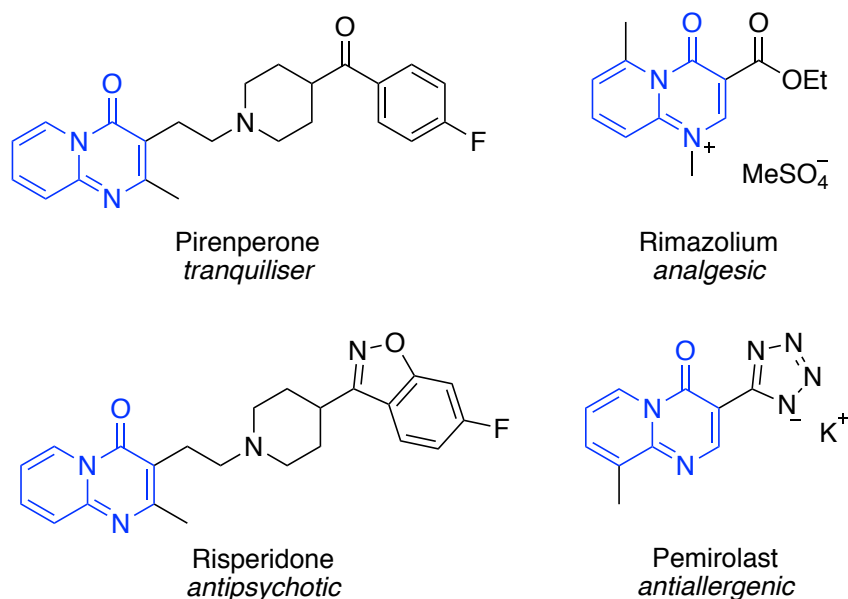
Figure 4.12: Notable pyrido[1,2- a ]pyrimidin-4-one containing drugs.
