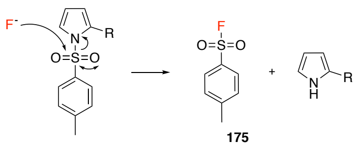
Figure 2.19: Possible reaction mechanism resulting in the formation of fluorinated by-product 175 .
