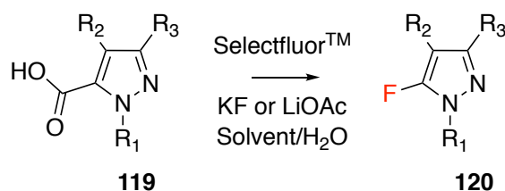
Figure 1.41: Synthesis of 5-fluoropyrazole derivatives by fluorodecarboxylation using Selectfluor TM .
