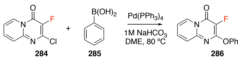
Figure 4.28: Attempted Suzuki reaction of 2-chloro-3-fluoro-4 H -pyrido[1,2- a ]pyrimidin-4-one.
