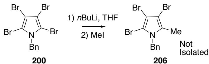
Figure 3.23: Attempted synthesis of 2-methyl substituted tribromopyrrole derivative 206 .
