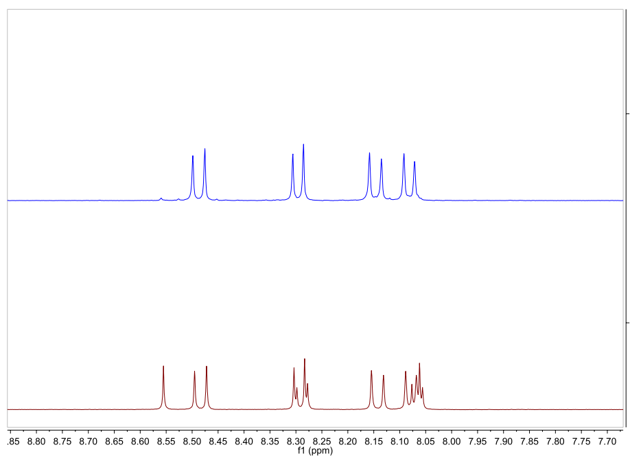
Figure 5.5: Aromatic region of the ^1\text{H} NMR spectra before (red) and after (blue) recrystallisations from toluene.
