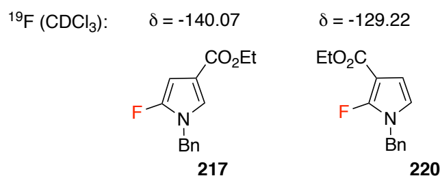
Figure 3.34: Reported ^{19}\text{F} chemical shifts of the 2-fluorinated 3- and 4-pyrrole ester regioisomers. [29]
