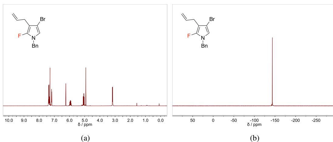
Figure 3.39: 1 H (a) and 19 F (b) NMR spectra of isolated 2-fluoro-3-allyl-4-bromo- N -benzylpyrrole ( 224 ).
