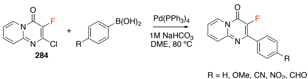
Figure 4.33: Synthetic routes to 2 substituted 3-fluoro-4 H -pyrido[1,2- a ]pyrimidin-4-ones.
