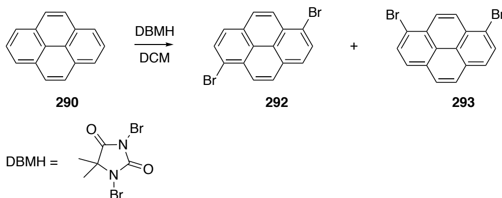
Figure 5.4: Synthesis of dibromopyrenes using DBMH.
