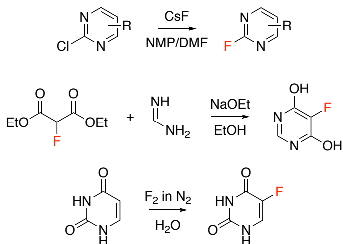
Figure 1.7: Synthesis of 2-fluoro and 5-fluoropyrimidines.
