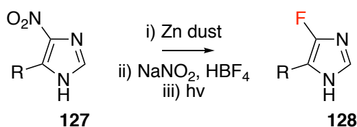
Figure 1.45: Photochemical Balz-Schiemann reaction for the synthesis of 4-fluoroimidazoles.
