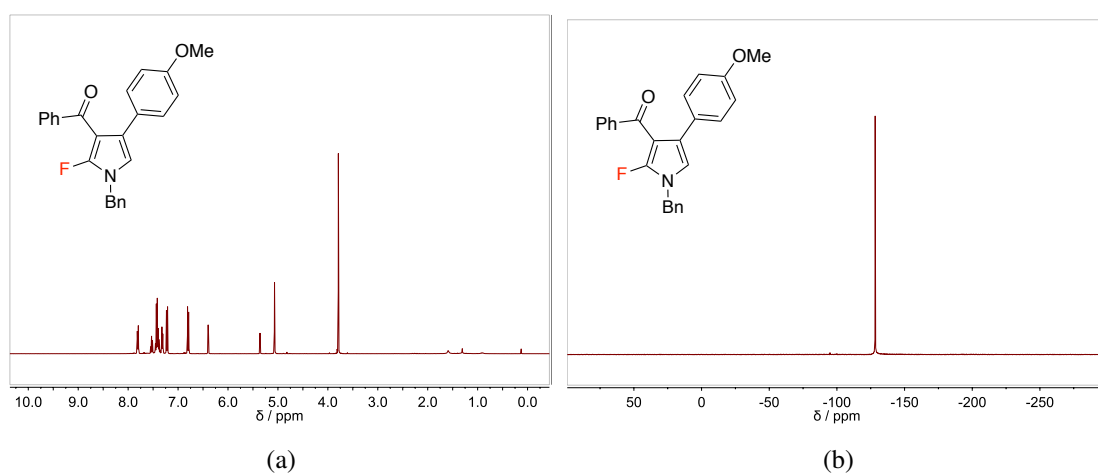
Figure 3.49: Illustrative ^1\text{H} (a) and ^{19}\text{F} (b) NMR spectra of isolated 2-fluoro-3-benzoyl-4-(4-methoxyphenyl)- N -benzylpyrrole 230b .
