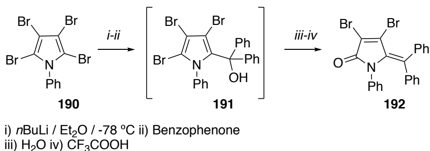
Figure 3.7: Metal-halogen exchange reaction of tetrabromopyrrole scaffold 190 .
