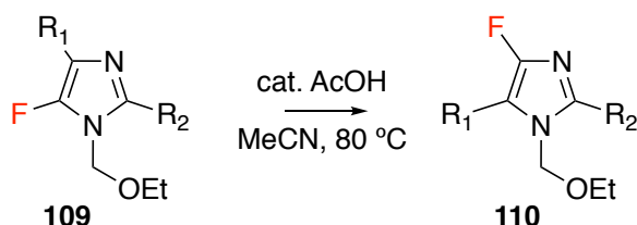
Figure 1.39: Controlled protecting group migration to produce 4-fluoroimidazoles from 5-fluoroimidazole derivatives.
