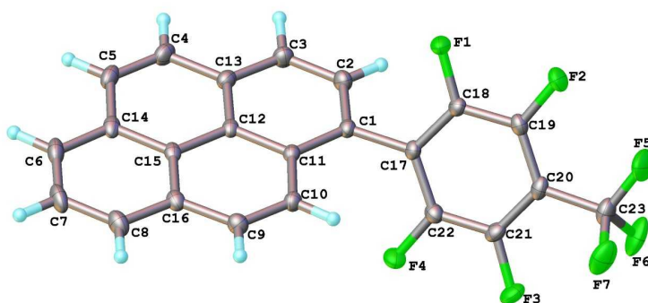
Figure 5.7: Molecular structure of 294 as determined by x-ray crystallography.
