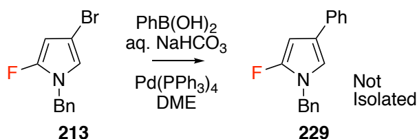
Figure 3.46: Attempted Suzuki cross-coupling of 2-fluoro-4-bromopyrrole derivative 213 .
