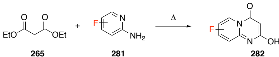
Figure 4.20: Synthesis of fluorinated pyrido[1,2- a ]pyrimidin-4-ones using fluorinated 2-aminopyridines.
