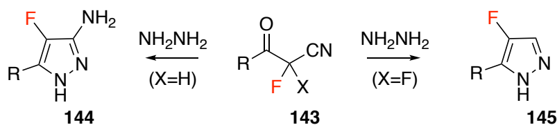
Figure 1.53: Synthesis of 4-fluoropyrazole derivatives from fluorinated \beta -ketonitriles.
