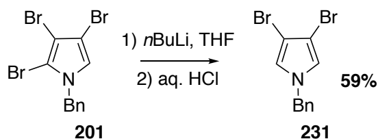
Figure 3.52: Synthesis of N -benzyl-3,4-dibromopyrrole 231 .
