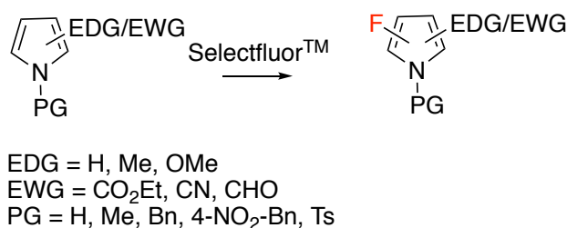
Figure 2.1: Proposed strategy for the synthesis of fluoropyrroles.
