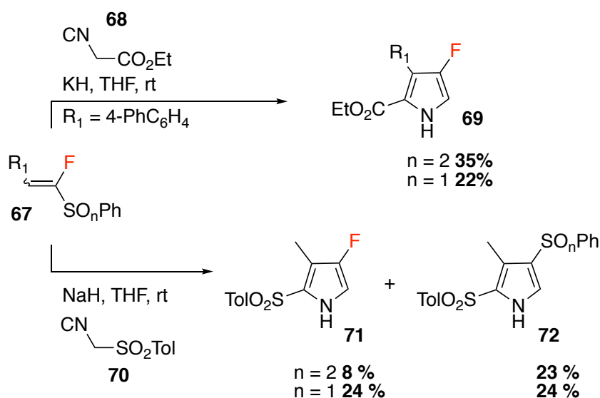
Figure 1.28: Synthesis of 3-fluoropyrrole derivatives 69 and 71 from isocyanide derivatives.
