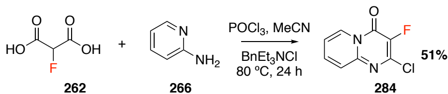
Figure 4.32: Synthesis of 2-chloro-3-fluoro-4 H -pyrido[1,2- a ]pyrimidin-4-one ( 284 ).
