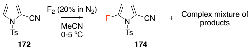
Figure 2.20: Attempted fluorination of substrate 172 using F 2 gas.
