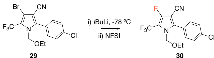
Figure 1.15: Synthesis of highly functionalised 3-fluoropyrrole derivative 30 .
