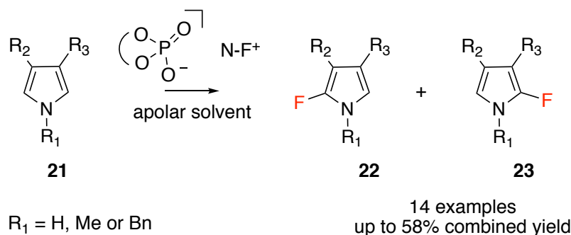
Figure 1.13: A phase transfer catalysis approach to substituted fluoropyrroles.
