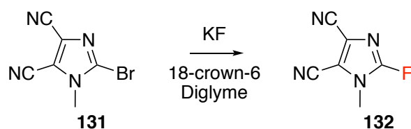
Figure 1.48: Halex process for the synthesis of 2-fluoroimidazole derivative 132 .
