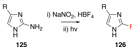
Figure 1.44: Photochemical Balz-Schiemann reaction for the synthesis of 2-fluoroimidazoles.
