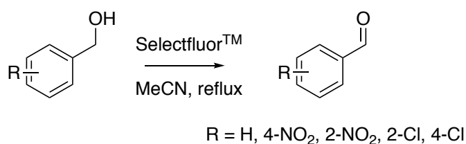
Figure 2.3: Oxidation of benzyl alcohols by Selectfluor TM . [82]
