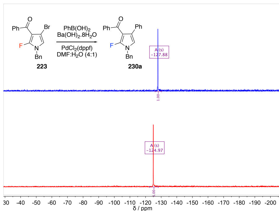
Figure 3.47: ^{19}\text{F} NMR spectra of the reaction mixture at time t=0 (red) and t=10\text{min} (blue) showing full conversion from the starting material.
