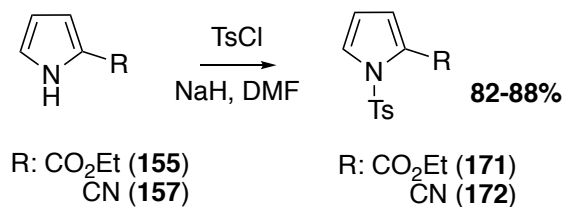
Figure 2.17: Synthesis of Ts protected pyrrole derivatives 171 and 172 .
