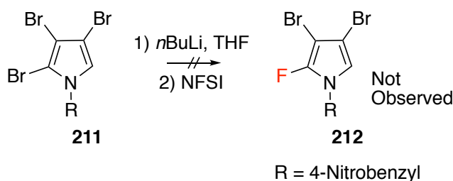
Figure 3.27: Attempted fluorination of 2,3,4-tribromo- N -(4-nitrobenzyl)pyrrole.
