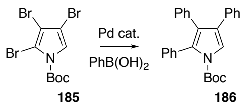
Figure 3.5: Synthesis of 2,3,4-triphenylpyrrole derivative 186 .
