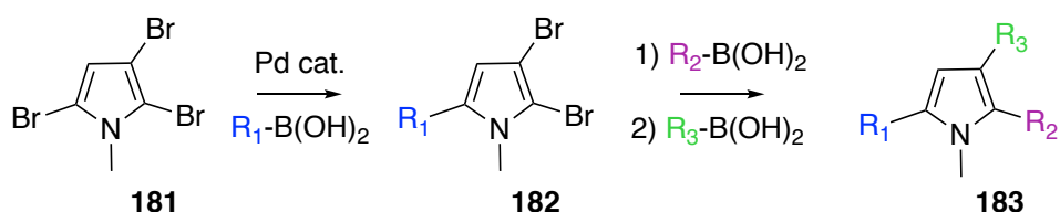
Figure 3.3: Regioselective Suzuki cross-coupling reactions of 2,3,5-tribromopyrrole derivative 181 .
