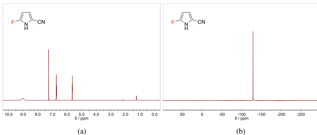
Figure 2.9: 1 H (a) and 19 F (b) NMR spectra of isolated 5-fluoropyrrole-2-carbonitrile 158 .
