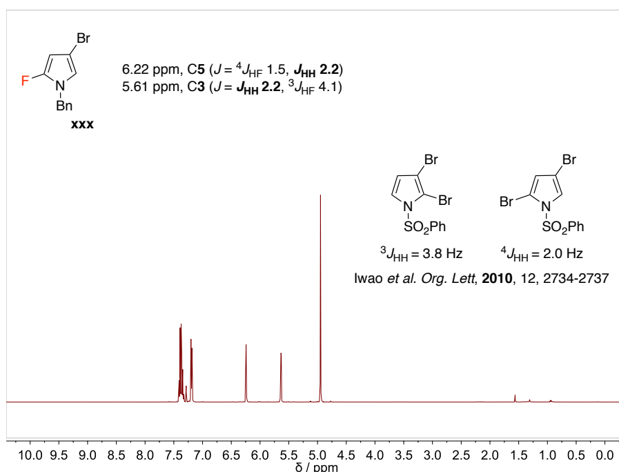
Figure 3.29: {}^1\text{H} NMR spectrum of isolated hydrodebrominated product and related literature J values. [105]
