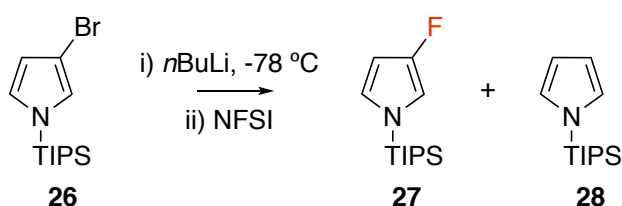
Figure 1.14: Synthesis of 3-fluoropyrrole derivative 27 via lithiation and quenching of brominated pyrroles.
