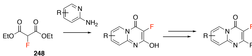
Figure 4.22: General strategy for the synthesis of fluorinated pyridopyrimidinones from 2-fluoromalonate ester 248 .
