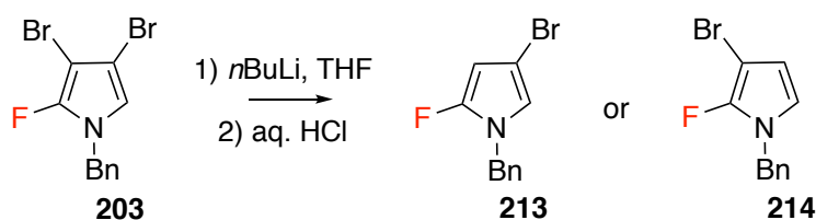
Figure 3.28: Possible regioisomeric products formed by dehydrobromination of dibrominated pyrrole derivative 203 .
