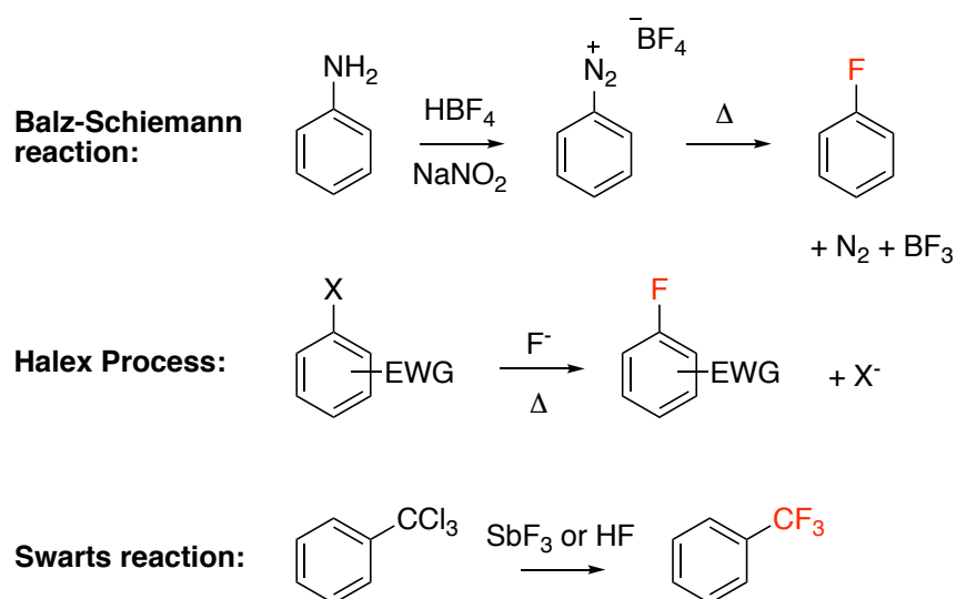
Figure 1.4: Traditional routes to fluoro- and trifluoromethyl-aromatic subunits of pharmaceuticals.
