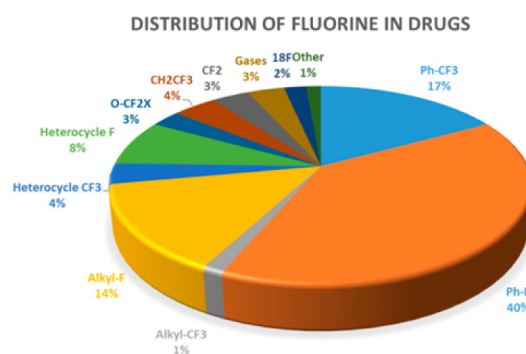
Figure 1.3: Distribution of fluorinated moieties in FDA approved drugs (1950-2014). [5]
