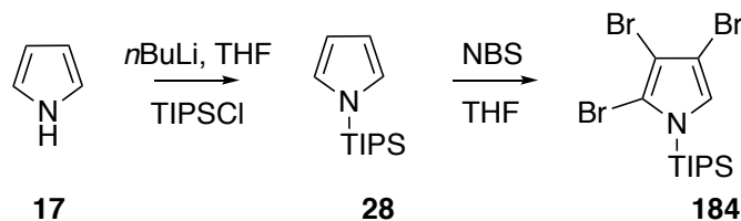
Figure 3.4: Synthesis of N -TIPS-2,3,4-tribromopyrrole ( 184 ).
