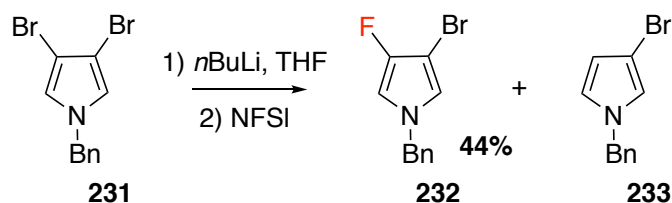
Figure 3.54: Synthesis of 3-fluoro-4-bromopyrrole derivative 232 .
