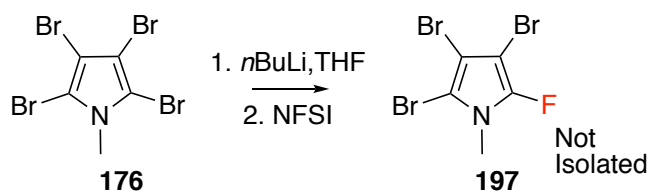
Figure 3.12: Attempted fluorination of 2,3,4,5-tetrabromo- N -methylpyrrole.
