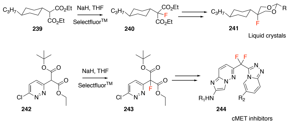
Figure 4.3: Fluorination of malonate esters using Selectfluor TM .
