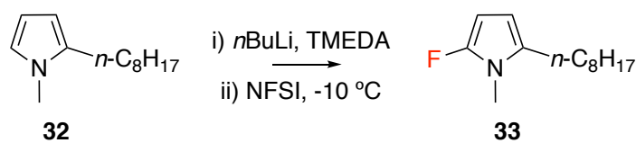
Figure 1.17: Synthesis of 2-fluoropyrrole derivative 33 .
