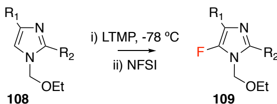
Figure 1.38: Synthesis of 5-fluoroimidazole derivatives using NFSI.
