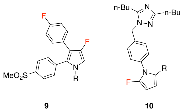
Figure 1.8: Examples of biologically active fluoropyrrole derivatives. [22,23]
