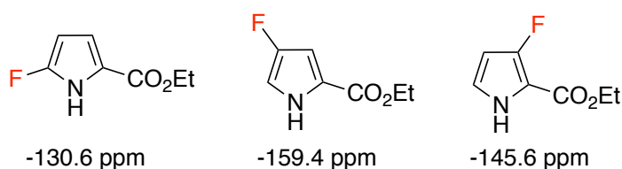
Figure 2.6: DFT predicted 19 F chemical shifts of monofluoropyrrole regioisomers.
