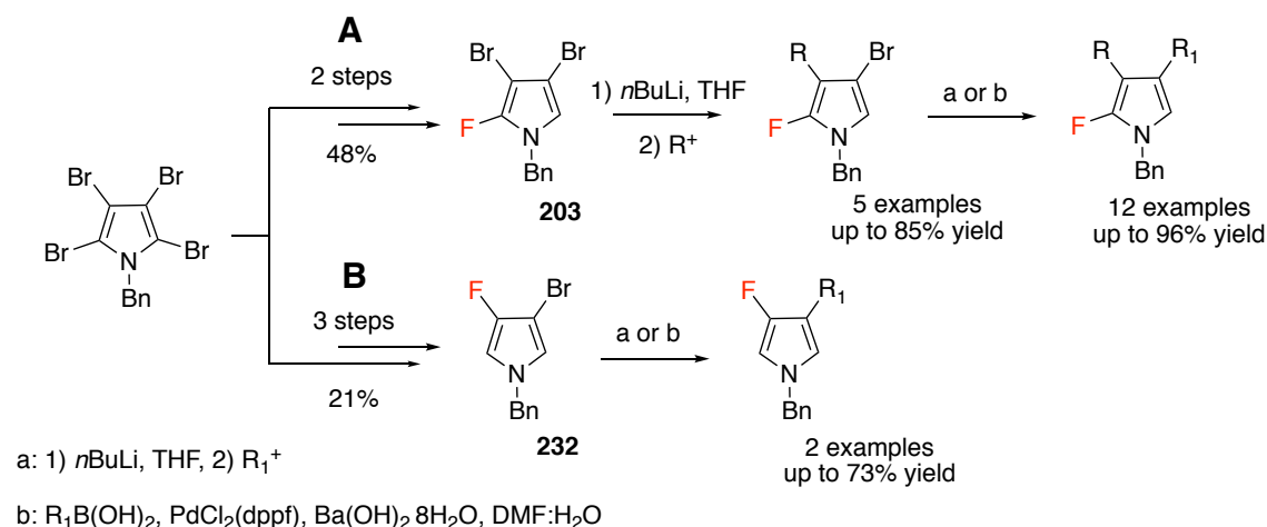
Figure 3.59: Summary of the library of 2- and 3-fluoropyrroles synthesised in this study.
