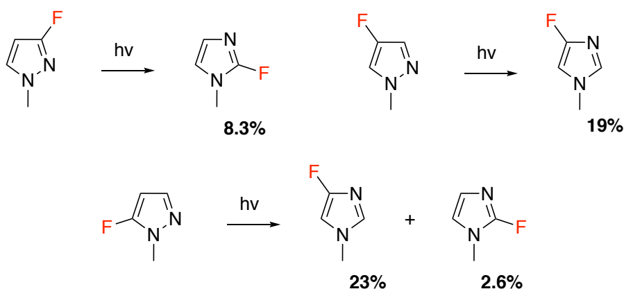
Figure 1.47: Photoinduced ‘nitrogen walk’ for the synthesis of fluoroimidazole derivatives.
