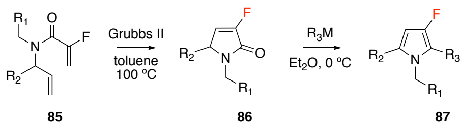
Figure 1.32: Ring closing metathesis and alkylation-aromatisation protocol for the synthesis of 3-fluoropyrrole derivatives ( 87 ).
