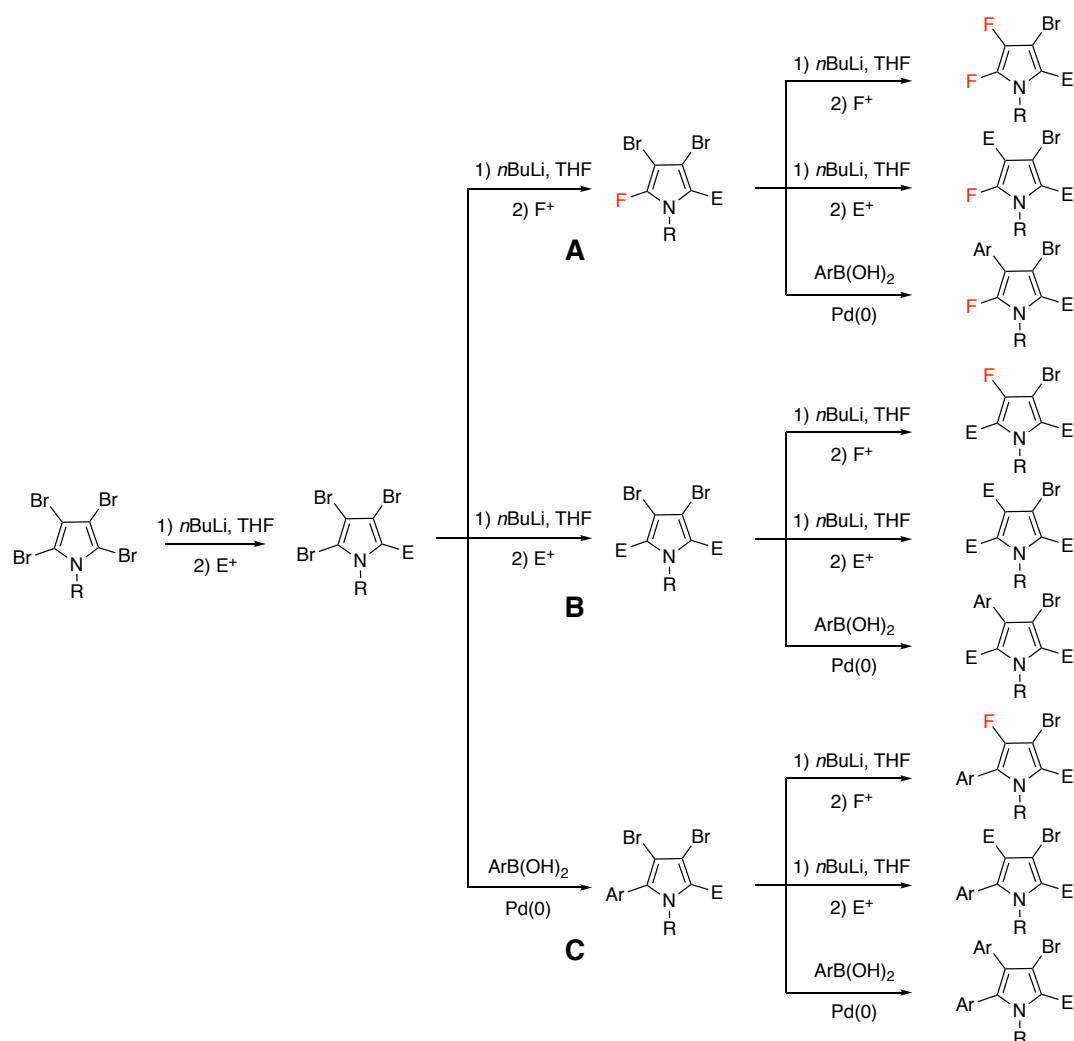
Figure 3.1: General bromination-derivatisation strategy to access a diverse library of functionalised pyrroles.
