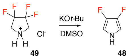
Figure 1.23: Improved synthesis of 3,4-difluoropyrrole ( 48 ).
