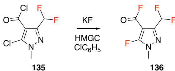
Figure 1.50: Synthesis of 5-fluoropyrazole derivative 136 using KF.
