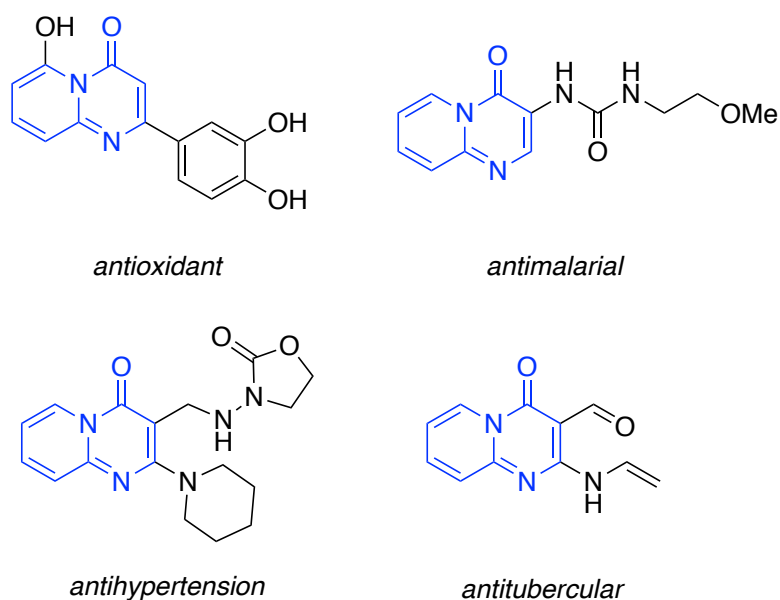
Figure 4.13: Examples of biologically active pyrido[1,2- a ]pyrimidin-4-ones.
