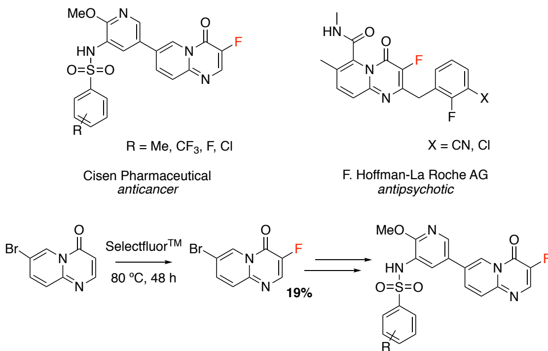
Figure 4.21: Patented 3-fluorinated pyrido[1,2- a ]pyrimidin-4-ones.
