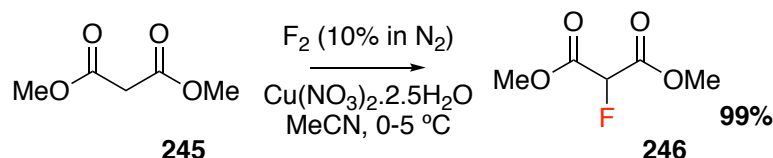
Figure 4.4: Elemental fluorine for the synthesis of 2-fluoromalonate ester 246 .
