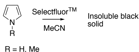
Figure 2.2: Polymerisation of pyrrole and N -methylpyrrole by Selectfluor TM .
