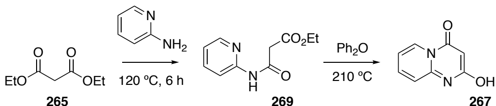
Figure 4.16: Two step process for the synthesis of 2-hydroxy-4 H -pyrido[1,2- a ]pyrimidin-4-one ( 267 ).
