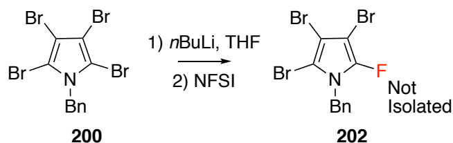
Figure 3.17: Attempted fluorination of 2,3,4,5-tetrabromo- N -benzylpyrrole.
