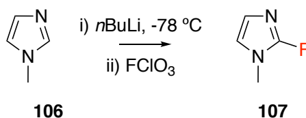
Figure 1.37: Synthesis of 2-fluoroimidazole derivative using perchloryl fluoride.
