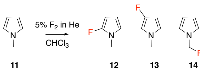
Figure 1.9: Fluorination reaction of N -methylpyrrole using F 2 .
