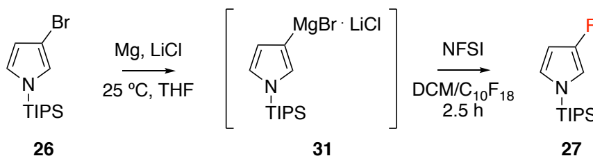
Figure 1.16: Grignard strategy for the synthesis of 3-fluoropyrrole derivative 27 .
