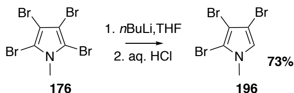
Figure 3.11: Hydrodebromination of 2,3,4,5-tetrabromo- N -methylpyrrole.
