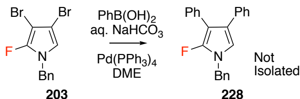
Figure 3.45: Attempted Suzuki cross-coupling of 2-fluoro-3,4-dibromopyrrole derivative 203 .
