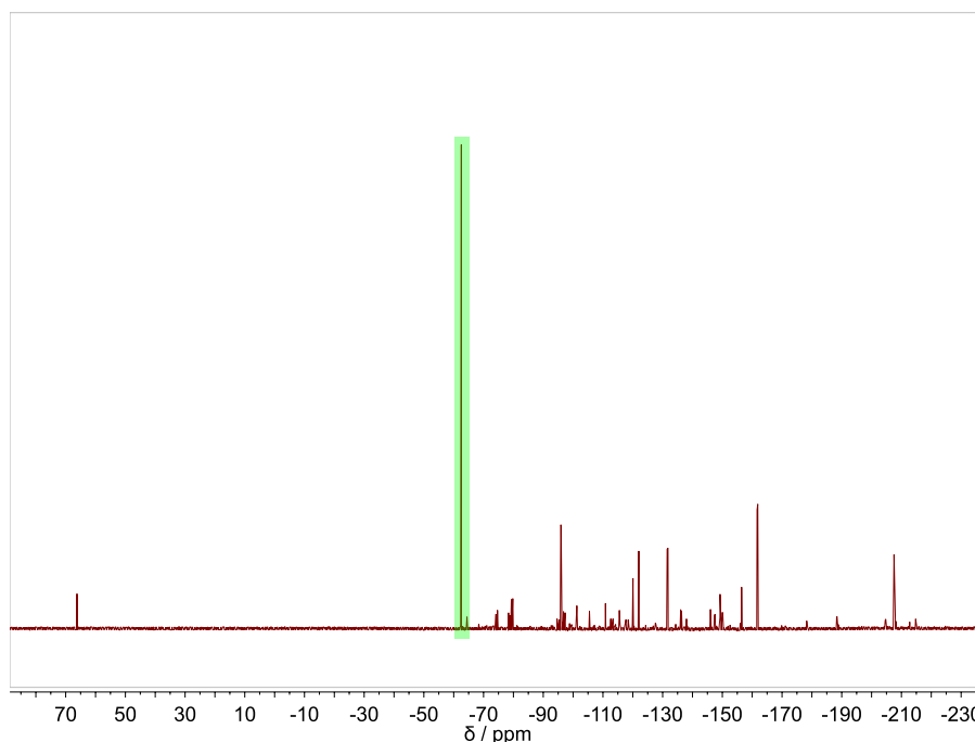
Figure 2.21: ^{19}\text{F} NMR spectrum of the crude reaction mixture following addition of 1.05 eq. \text{F}_2 (external reference highlighted in green).
