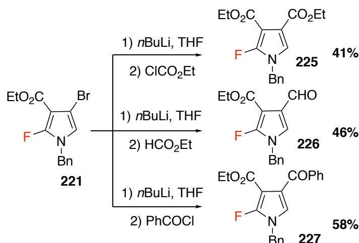
Figure 3.42: Synthesis of 2-fluoro-3,4-disubstituted pyrrole derivatives 225 , 226 and 227 by sequential lithiation and quenching.
