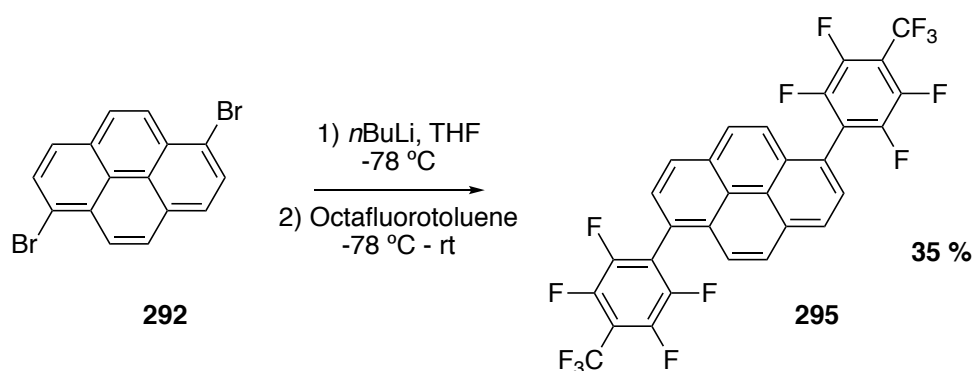
Figure 5.8: Synthesis of 1,6-di(2,3,5,6-tetrafluoro-4-(trifluoromethyl)phenyl)pyrene ( 295 ).
