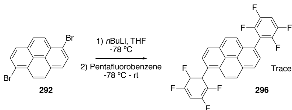
Figure 5.10: Attempted synthesis of tetrafluorobenzene substituted pyrene derivative 296 .
