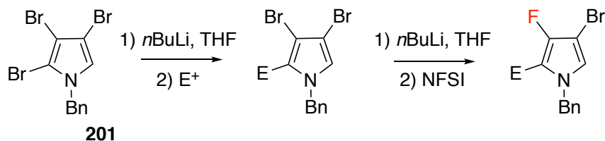
Figure 3.51: Synthetic strategy for the synthesis of 3-fluorinated pyrrole derivatives.
