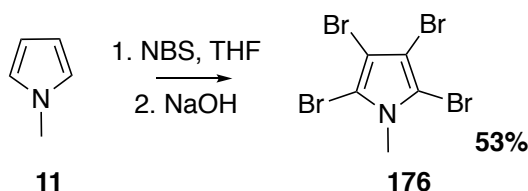
Figure 3.10: Bromination of N -methylpyrrole using NBS.
