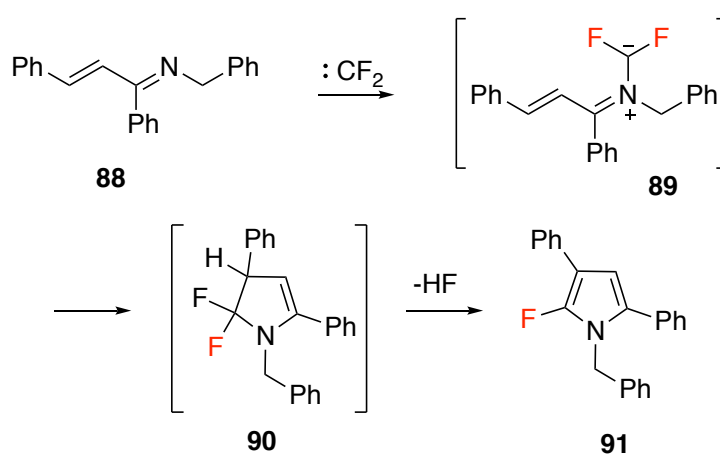
Figure 1.33: Synthesis of 2-fluoropyrrole derivative ( 91 ) from azadiene derivative ( 88 ).
