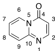
Figure 4.14: Labelled pyrido[1,2- a ]pyrimidin-4-one structure.
