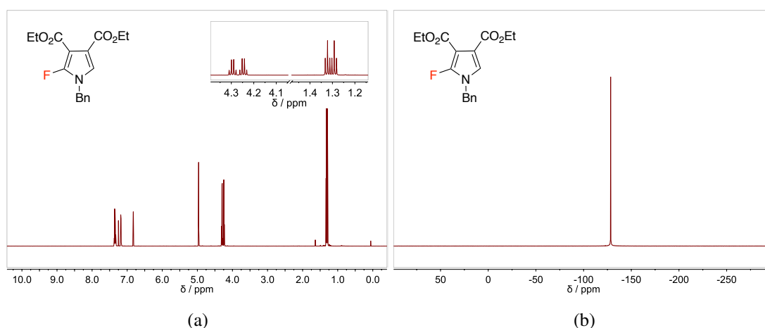
Figure 3.43: Illustrative 1 H (a) and 19 F (b) NMR spectra of isolated diethyl 2-fluoro- N -benzylpyrrole-3,4-dicarboxylate 225 .
