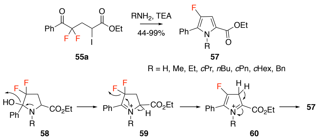
Figure 1.25: Synthesis of N -substituted 3-fluoropyrrole derivatives from 55a using primary amines.
