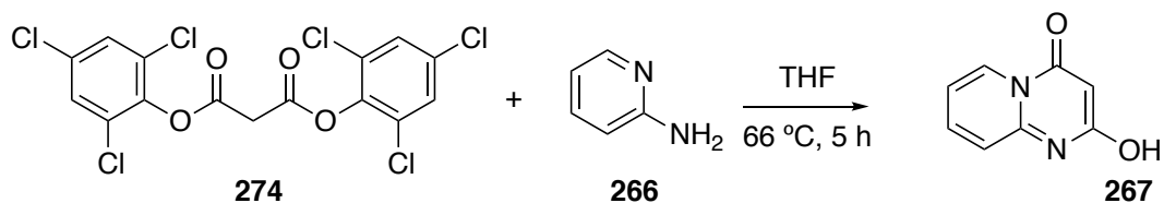
Figure 4.18: Low temperature condensation using activated ester 274 .
