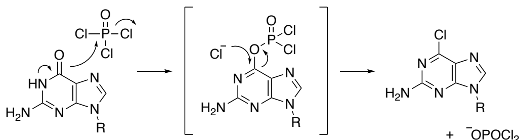
Figure 4.26: Chlorination reaction using \text{POCl}_3 studied by ^{31}\text{P} NMR spectroscopy. [155]
