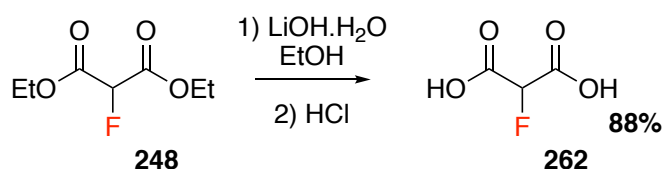
Figure 4.25: Hydrolysis of malonate ester to give 2-fluoromalonic acid ( 262 ).
