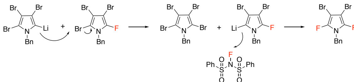
Figure 3.18: Proposed halogen dance type mechanism to account for the crude product composition.
