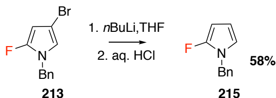
Figure 3.30: Synthesis of N -benzyl-2-fluoropyrrole.
