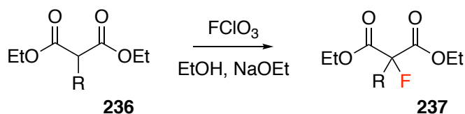
Figure 4.1: Synthesis of 2-fluoromalonate esters using \text{FClO}_3 .
