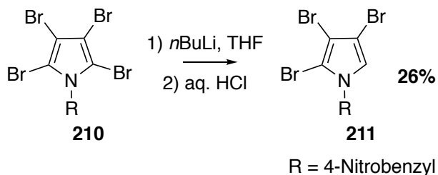
Figure 3.26: Hydrodebromination of 2,3,4,5-tetrabromo- N -(4-nitrobenzyl)pyrrole.
