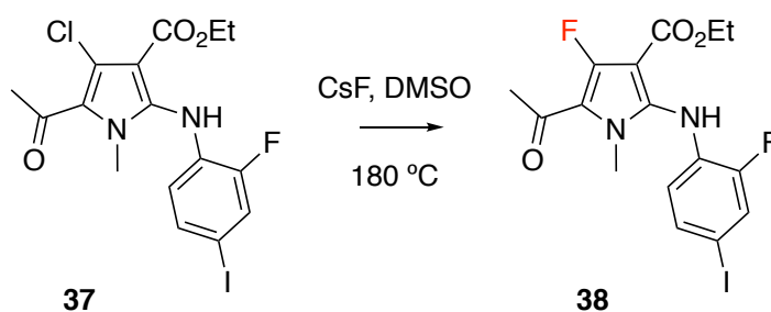
Figure 1.19: Nucleophilic substitution using CsF to produce 3-fluoropyrrole derivative 38 .
