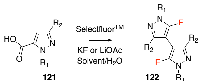
Figure 1.42: Synthesis of fluorinated pyrazole dimers with a 4,4'-linkage.
