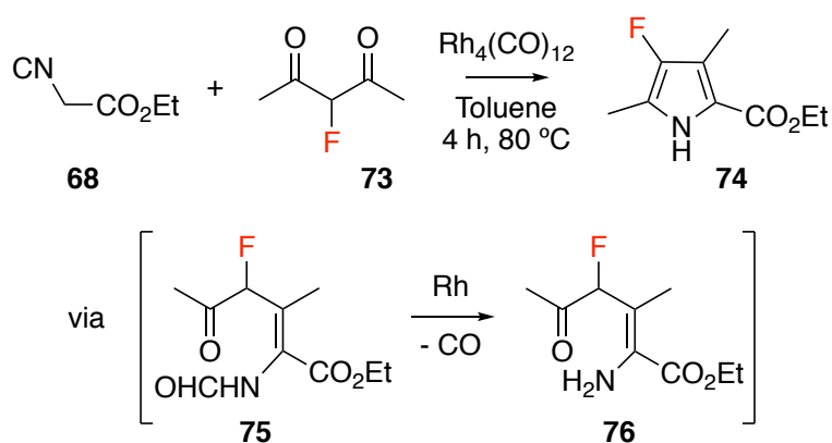
Figure 1.29: Rhodium catalysed synthesis of 74 from ethyl isocyanoacetate 68 .
