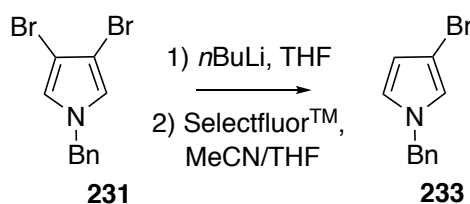
Figure 3.55: Attempted fluorination using Selectfluor TM resulting in exclusive hydrodebromination.
