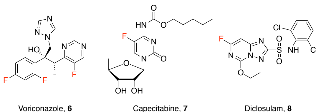
Figure 1.5: Commercialised life science products containing a fluorinated six-membered azaheterocycle.
