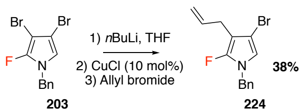
Figure 3.38: Allylation reaction by transmetalation with Cu I salt.
