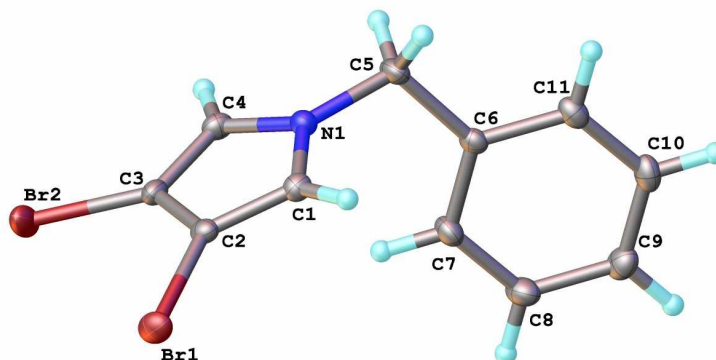
Figure 3.53: Molecular structure of 231 as determined by x-ray crystallography.
