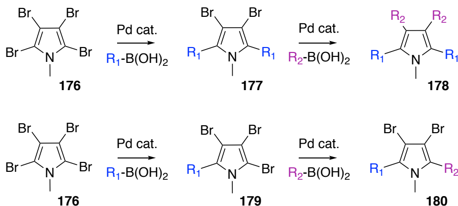
Figure 3.2: Regioselective Suzuki cross-coupling reactions of tetrabromopyrrole derivative 176 .
