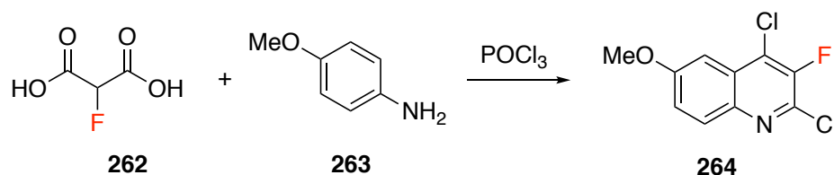
Figure 4.11: One step synthesis of 2,4-dichloro-3-fluoroquinoline derivative 264 from 2-fluoromalonic acid.
