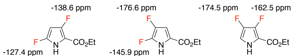
Figure 2.7: DFT predicted ^{19}\text{F} chemical shifts of difluoropyrrole regioisomers.
