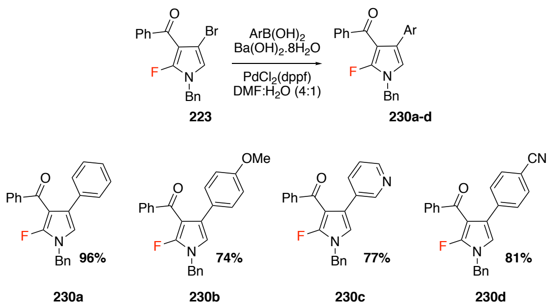
Figure 3.48: Suzuki cross-coupling reactions to give 2-fluoro-3-benzoyl-4-arylpyrrole derivatives 230a-d .
