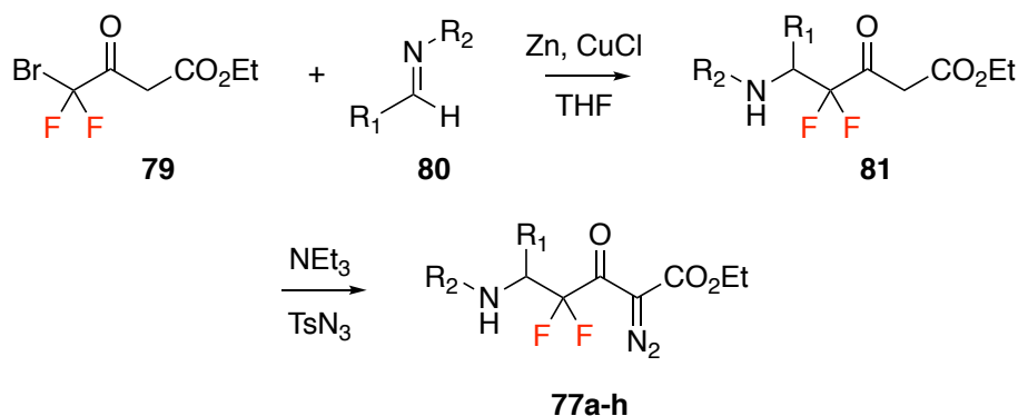
Figure 1.30: Synthesis of diazo-intermediates 77a-h .
