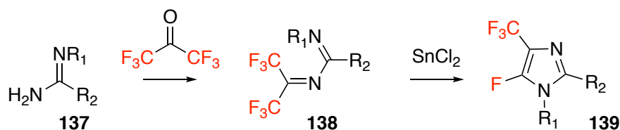
Figure 1.51: Synthesis of 5-fluoroimidazole derivatives from hexafluoroacetone and amidine precursors.
