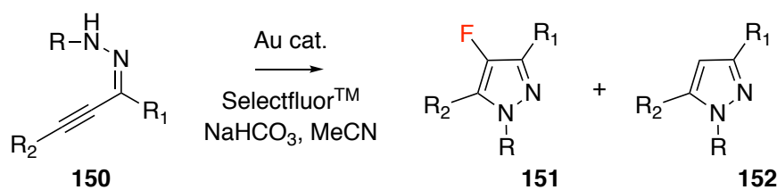
Figure 1.56: Gold catalyzed synthesis of 4-fluoropyrazoles.
