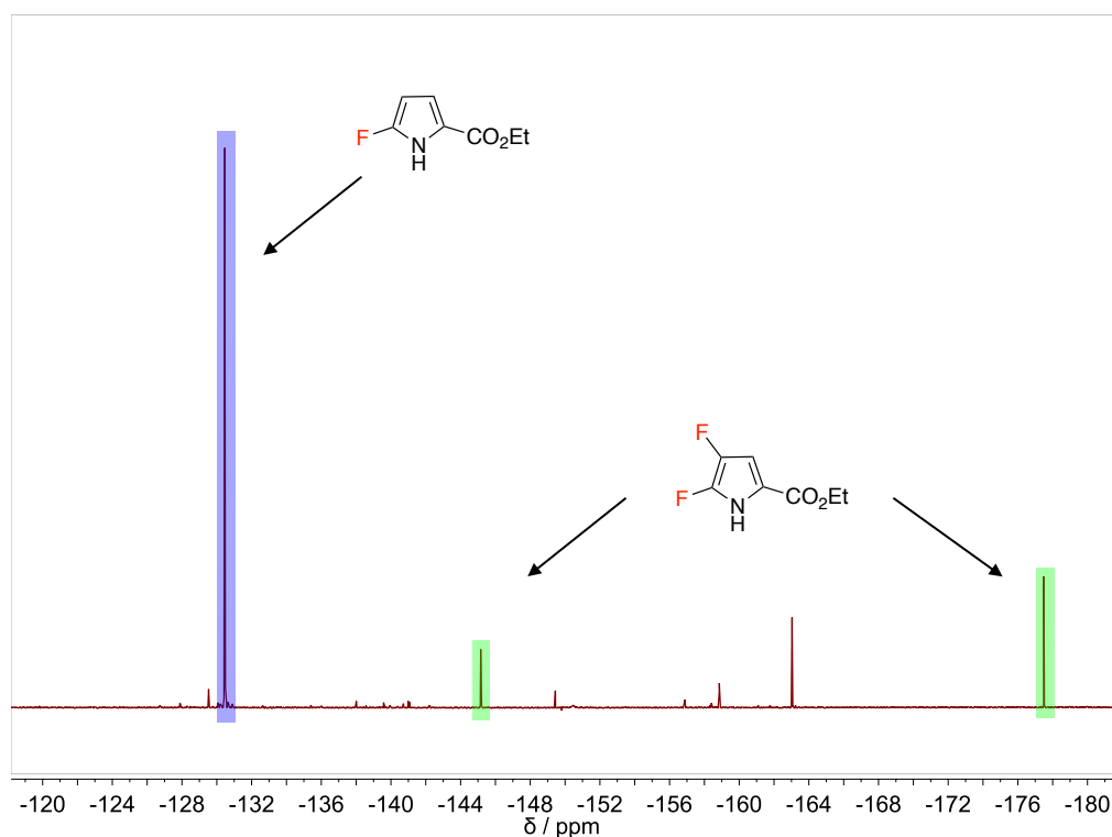
Figure 2.8: ^{19}\text{F} NMR of the crude product mixture from reaction of 155 with Selectfluor TM , showing the 5-fluoro (blue) and 4,5-difluoropyrrole (green) products.
