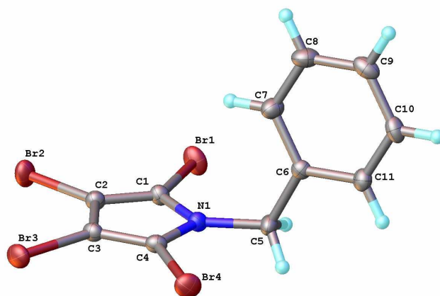
Figure 3.15: Molecular structure of 200 as confirmed by x-ray crystallography.
