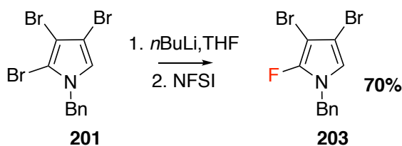
Figure 3.19: Synthesis of 2-fluoro-3,4-dibromopyrrole derivative 203 .
