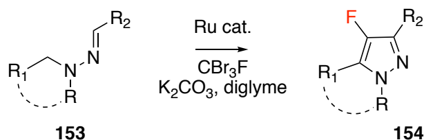
Figure 1.57: Ruthenium catalyzed synthesis of 4-fluoropyrazoles.
