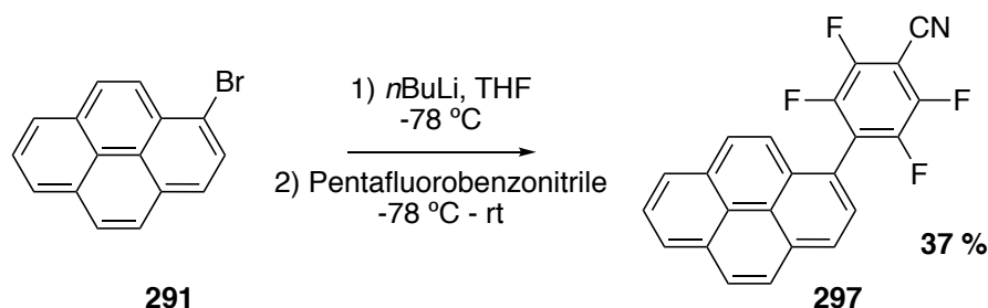
Figure 5.12: Synthesis of 1-(2,3,5,6-tetrafluorobenzonitrile)pyrene ( 297 ).
