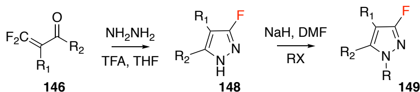
Figure 1.55: Synthesis of 3-fluoropyrazoles from 2,2-difluorovinylketones.
