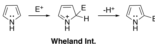
Figure 2.4: Electrophilic substitution of pyrrole via Wheland intermediate.
