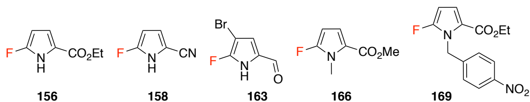
Figure 2.22: Fluorinated pyrrole derivatives synthesised by reaction with Selectfluor TM .
