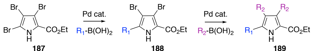
Figure 3.6: Regioselective Suzuki cross-coupling reactions of ethyl 2,3,4-tribromopyrrole-5-carboxylate ( 187 ).
