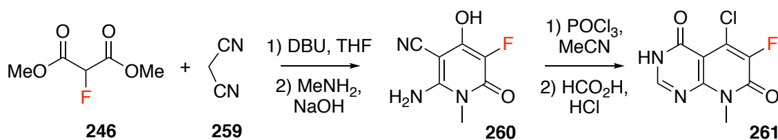
Figure 4.10: Synthesis of 6-fluoro-8-methylpyrido[2,3- d ]pyrimidine-4,7-(3 H ,8 H )-dione ( 261 ) from dimethyl 2-fluoromalonate.
