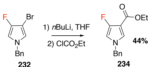
Figure 3.57: Synthesis of ethyl 3-fluoro- N -benzylpyrrole-4-carboxylate.
