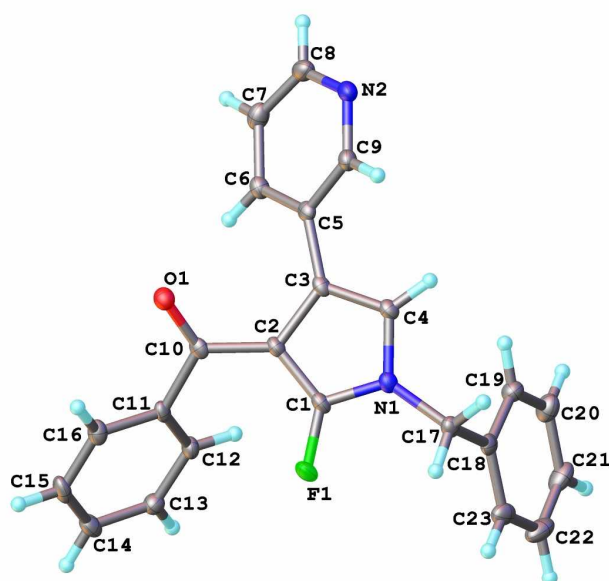
Figure 3.50: Molecular structure of 230c as determined by x-ray crystallography.
