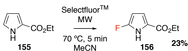
Figure 2.5: Synthesis of ethyl 5-fluoropyrrole-2-carboxylate ( 156 ) with Selectfluor TM under MW conditions.
