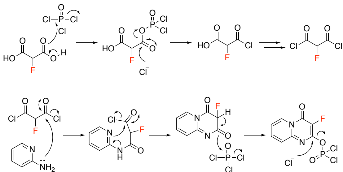
Figure 4.27: Proposed mechanism for the synthesis of 2-chloro-3-fluoro-4 H -pyrido[1,2- a ]pyrimidin-4-one.
