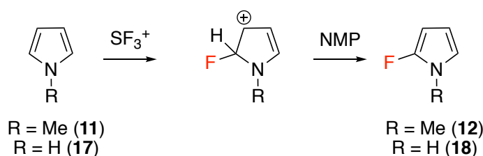
Figure 1.10: Fluorination of pyrrole and N -methylpyrrole using \text{SF}_3^+ .
