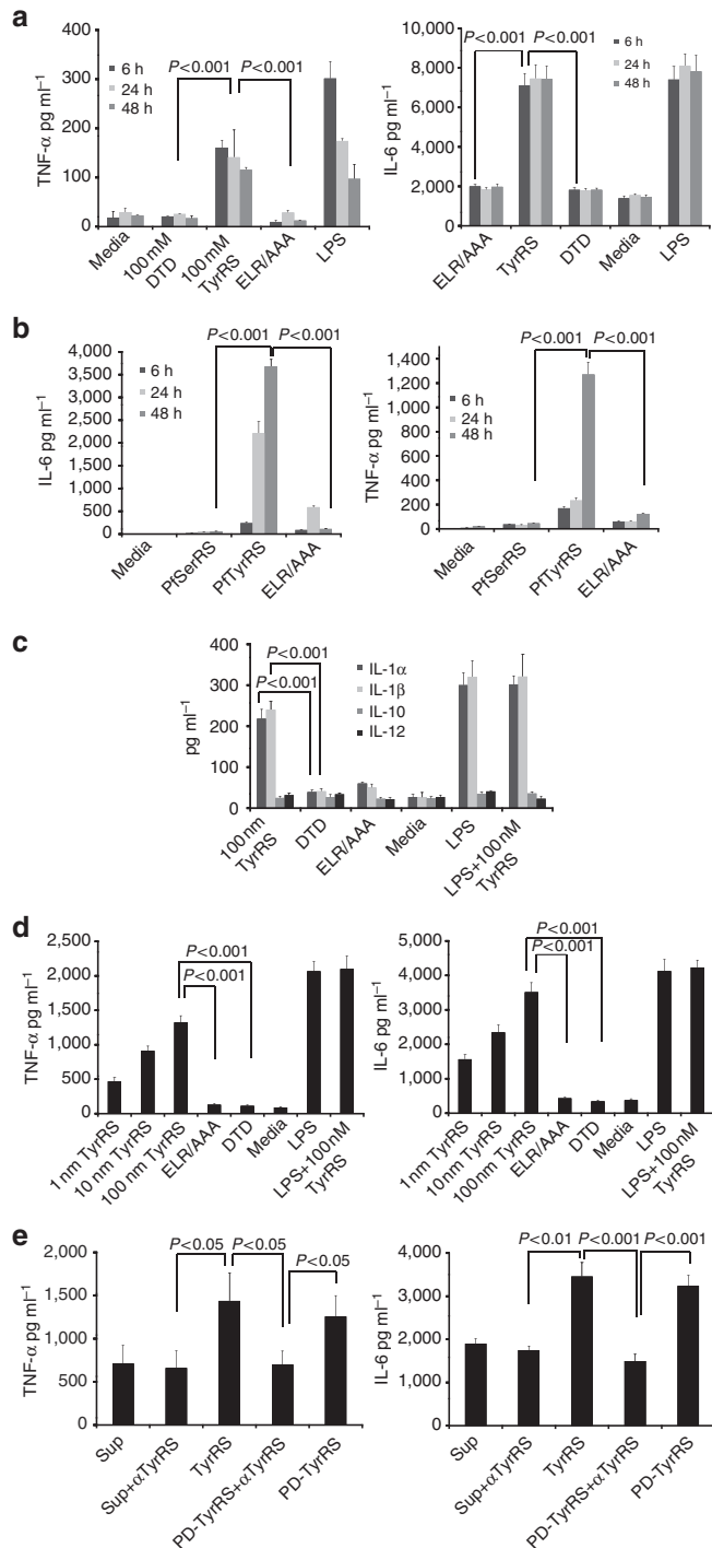
Figure 5 | Effect of PfTyrRS on mouse macrophages. (a) Cytokines levels were measured using BioPlex kit (Bio-Rad) and the secretion profiles of TNF- \alpha and IL-6 using mouse macrophages were measured at different time points. Media alone, PfDTD/PfSerRS enzymes and ELR-AAA mutant of PfTyrRS were used as negative controls. LPS was used as positive control in all experiments. (b) Identical experiment as in (a) except that the human macrophage cell line ThP1 was used. This experiment has the extra negative control of PfSerRS. (c) Secretion profiles of extra cytokines (IL-1, IL-10 and IL-12) that are secreted from human macrophages on exposure to PfTyrRS . (d) Dose-dependent increase in secretion of TNF- \alpha and IL-6 when increasing concentrations of PfTyrRS were used with human macrophages. (e) Cytokine secretion profiles using P. falciparum culture supernatants alone (Sup), supernatants incubated with anti-TyrRS antibody (Sup + \alpha TyrRS), parasite culture supernatant-immunoprecipitated PfTyrRS (PD-TyrRS) and finally parasite culture supernatant -immunoprecipitated PfTyrRS with its antibody (PD-TyrRS + \alpha TyrRS). TNF- \alpha and IL-6 secretion is clearly enhanced significantly when immunoprecipitated PfTyrRS (PD-TyrRS) is used. Triggering activity of PfTyrRS (PD-TyrRS) is blocked when pre-incubated with anti- PfTyrRS antibodies, indicating specific activation of macrophages with native PfTyrRS (PD-TyrRS). Experiments were repeated three times and error bars indicate standard deviation. Tukey's test was performed and P -values are shown such that the end points of the lines below P -value represent the datasets that were compared.
