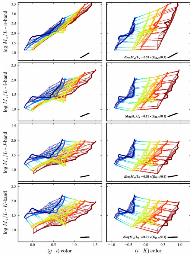
Figure 14. Variations in M_*/L as a function of restframe (g - i) and (i - K) colour for models in our SPL. All symbols and their meanings are as in the directly comparable Fig. 10. In contrast to (g - i) , optical-minus-NIR colours contain virtually no information directly pertaining to M/L , or to age. Instead, the optical-to-NIR colour is sensitive primarily to variations in dust and metallicity. While the inclusion of NIR data into the SPS fitting calculation may in principle lead to tighter constraints on t , \tau , Z , and E_{B-V} , it will have little to no impact on the accuracy of our M_*/L estimates.
