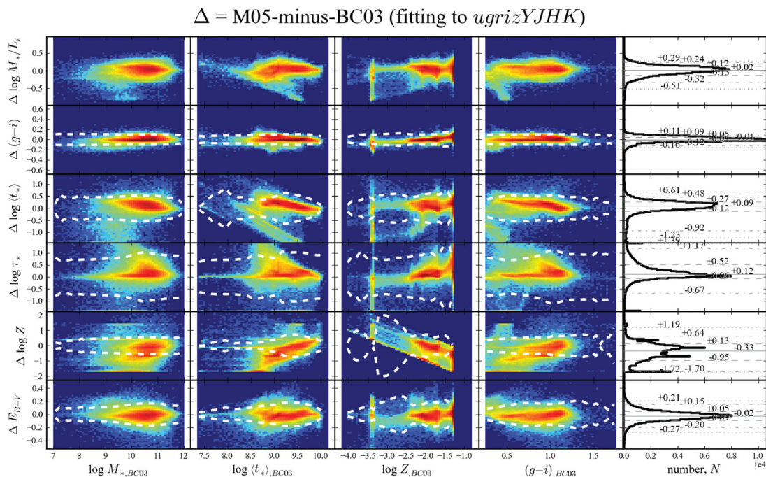
Figure 9. Comparison between M05- and BC03-based parameter estimates, derived from fits to the ugrizYJHK SEDs. The ‘ \Delta ’s in this figure should be understood as the M05-based-minus-BC03-based parameter values; all symbols and their meanings are analogous to Fig. 8. While, as expected, there are some systematics in the inferred values of M_* as a function of \langle t_* \rangle , the global agreement is very good. In comparison to Fig. 8, the systematic differences between parameters derived on the basis of the different stellar evolution models (but the same ugrizYJHK data) are considerably larger than the differences between the values inferred with or without the inclusion of the NIR data (but the same stellar evolution models). This suggests that our apparent inability to adequately fit the observed optical-to-NIR SED shapes of GAMA galaxies is not a product of errors in the stellar evolution models. At the same time, however, the ‘random’ differences between the M05- and BC03-based SP parameter estimates are larger than the formal uncertainties when the NIR data are included. This is not true when using only the optical data. That is, the model dependence of the SP parameter estimates becomes significant if, and only if, the NIR data are included.
