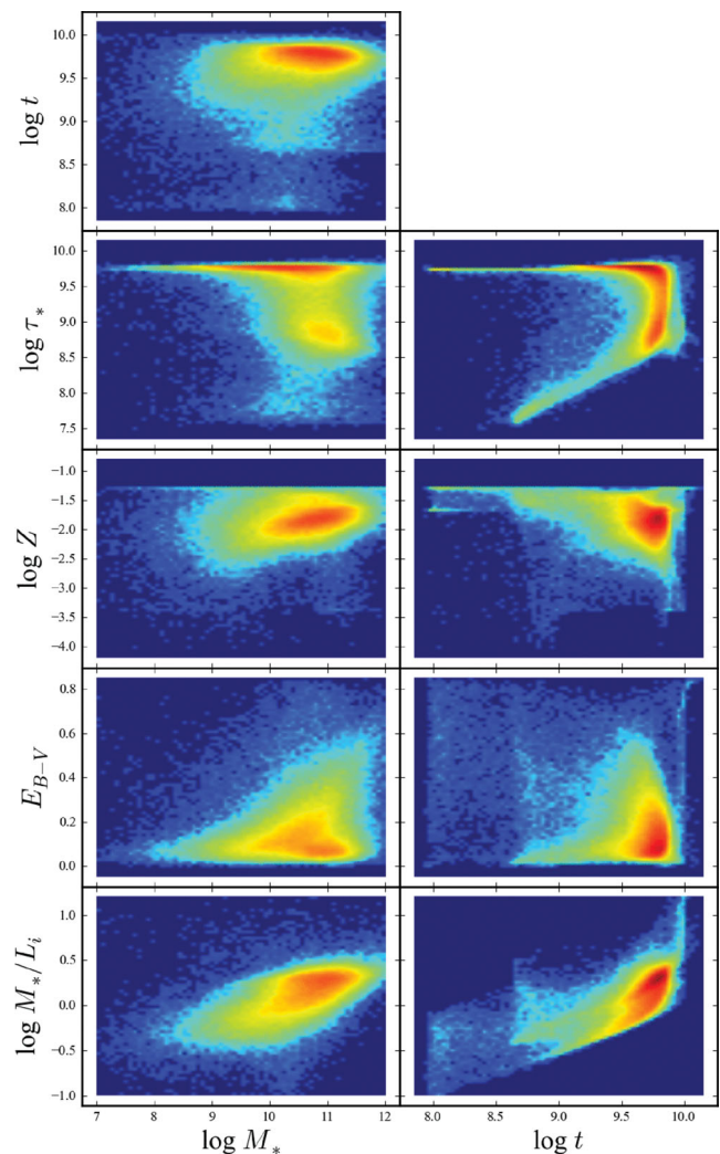
Figure 3. Illustrating the inferred distribution of SP parameters for GAMA galaxies. In this figure, we show the interrelationships between several important SP parameters for GAMA galaxies. Note that the SPL covers the full range of t , \tau and E_{B-V} shown. The observed relations between these parameters show that information about the process of galaxy formation and evolution can be extracted from galaxies’ SEDs. From an algorithmic point of view, the most important point to take from this plot is that by using a Bayesian approach, we are able for the most part to avoid ‘discretization’ errors (i.e. preferred parameter values) associated with the use of a discrete grid of parameter values (cf. Fig. 2). Further, note that particularly for t , \tau , and Z , these distributions are qualitatively different from those in Fig. 2.
