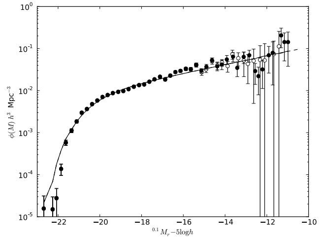
Figure 12. LF estimates in the r band for low-redshift galaxies ( z < 0.1 ) using the CMB reference frame (open circles) and the Tonry et al. (2000) multi-tractor flow model (filled circles) using the SWML estimator. The solid and dashed lines show the best-fitting Schechter functions which are indistinguishable.
