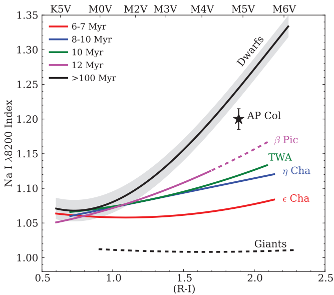
Figure 6. Na I index trends for various young, local associations from Lawson et al. (2009). The shaded band represents the variation around the mean dwarf trend seen in Lyo et al. (2004). The value of AP Col has been derived from our WiFeS R3000 spectra, smoothed to the approximate resolution of the Lawson et al. data. The error bar shows the variation observed among the four exposures. AP Col has an intermediate gravity, suggestive of an age between 12 and 100 Myr.
