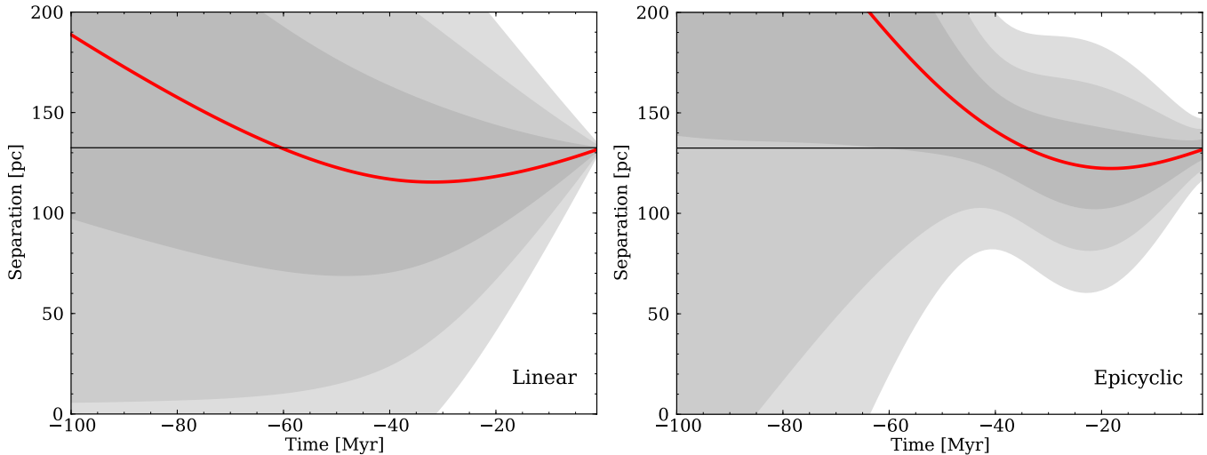
Figure 11. Separation between AP Col and the mean IC 2391 location (dotted line) as a function of time, with their current separation ( \sim 130 pc) on the right-hand side. Each plot shows the result of 1000 Monte Carlo simulations of the linear/ballistic (left) and epicyclic (right) approximations to Galactic dynamics, using the observed uncertainties in the observed AP Col and IC 2391 space motions. The shaded regions show 1 (darkest), 2, and 3\sigma (lightest) confidence intervals around the mean trend. If AP Col were a member of IC 2391, the separation of AP Col and IC 2391 should go to zero when they were both born ( \sim 40 – 50 Myr ago); they do not reasonably converge at the \sim 2\sigma level until \sim 80 Myr ago. This implies either interactions have modified the observed velocities, or that AP Col did not form near the core of IC 2391.
