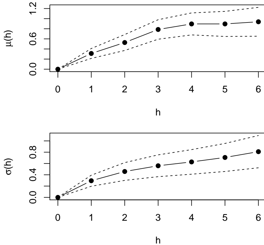
Figure 7: Pointwise estimates of \mu(h) and \sigma(h) with properties shown identical to Figure 6.
