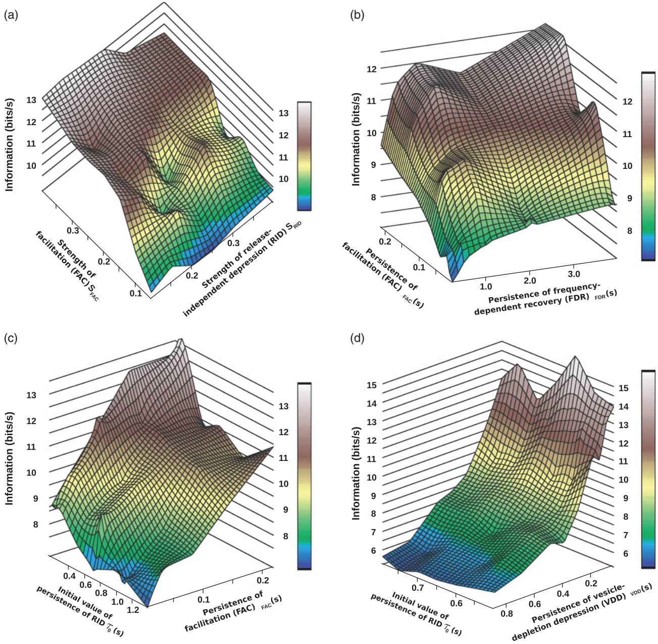
FIG. 7. (Color online) Extended investigations into the impact of short-term plasticity upon information transfer with spike timings. Error bars are omitted for clarity, but can be inferred as 8.0% of information values. All local variation in surfaces is below this level, except that seen in (a): the impact of the strength of RID ( S_{RID} ) and FAC ( S_{FAC} ) in a typical facilitating connection. RID clearly reduces information transfer and facilitation increases it, although a more complex interaction can be seen in the undulating region of the surface around S_{FAC} = S_{RID} (see text). (b) Time courses of FAC ( \tau_{FAC} ) and FDR ( \tau_{FDR} ) in a facilitating connection. Both processes enhance information transfer if slower decays are allowed, but a greater difference is seen at lower values of \tau_{FDR} than at higher values. (c) Time courses of FAC ( \tau_{FAC} ) and RID ( \tau_0 , the initial value of \tau_{RID} ) at a facilitating connection, confirming the generally positive influence of facilitation upon transfer rates, and the negative influence of RID. (d) Time courses of RID ( \tau_0 ) and VDD ( \tau_{VDD} ) in a typical depressing connection. While greater persistence of each decreases information transfer, VDD can be seen to have the larger influence in this case. Except for those shown on the axes, all parameter values were held constant at the values defined in Table II.
