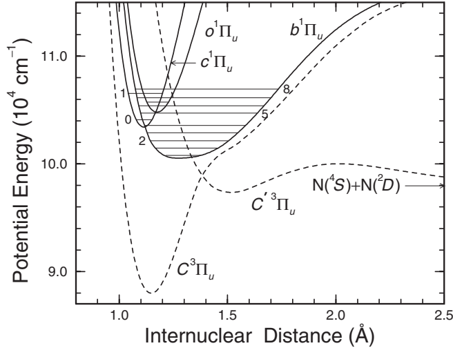
FIG. 1. Diabatic potential-energy curves used in the CC model, referred to the v = 0, J = 0 level of the X^1\Sigma_g^+ ground state (not shown). Solid curves: {}^1\Pi_u states. Dashed curves: {}^3\Pi_u states. The lowest singlet levels are indicated, associated with the nominal diabatic potential-energy curve, and emphasizing the perturbation resulting from the b \sim c crossing.
