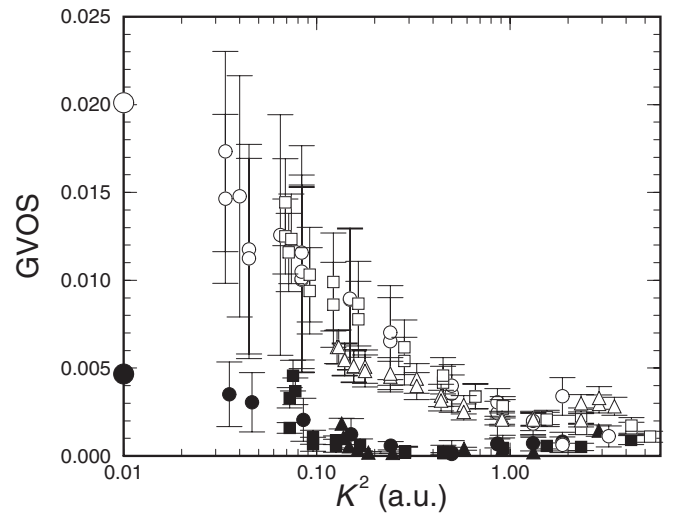
FIG. 3. Comparison of experimental GVOSs for b-X(5,0) and b-X(2,0) bands of N_2 (solid and open symbols, respectively). Circles: E_0 = 100 eV. Squares: E_0 = 50 eV. Triangles: E_0 = 30 eV. The optical oscillator strengths of Stark et al. [47], adjusted to room temperature [48], are also shown (large circles, plotted on the GVOS-axis for convenience).
