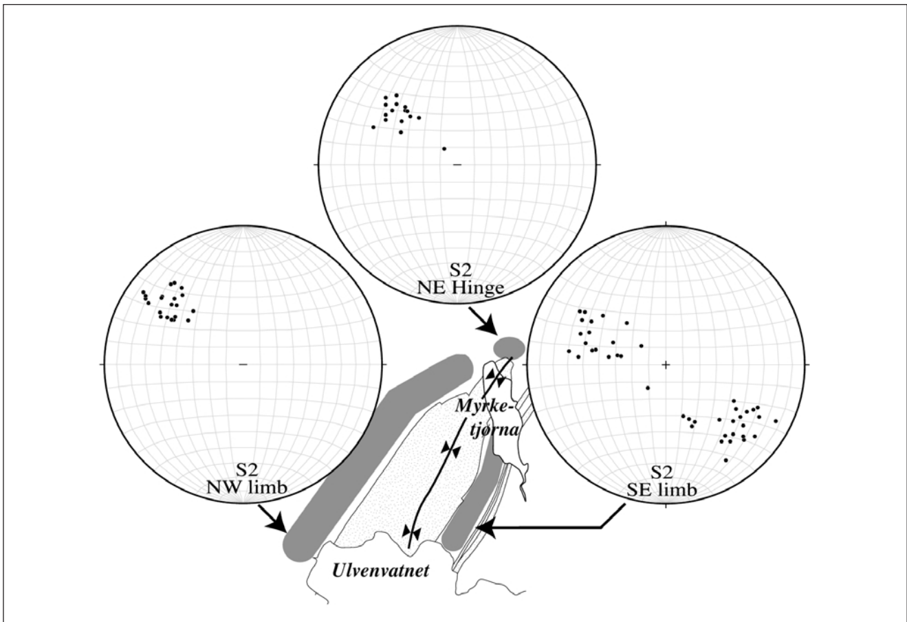
Fig. 5. Stereoplots of the second (S2) cleavage in phyllites of the Vaktal Fm. around the northeastern closure of the Ulven Syncline. Note anomalous orientations on the SE limb.
